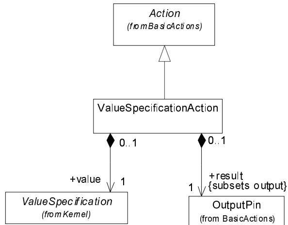
Figure 151 - Miscellaneous actions
