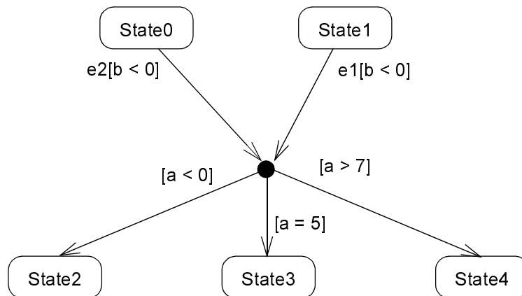
Figure 374 - Junction
