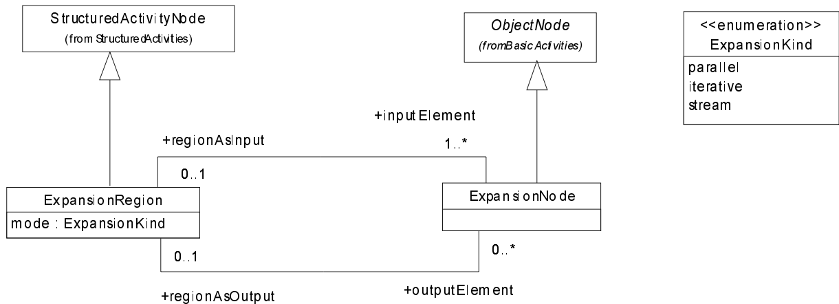
Figure 198 - Expansion regions
