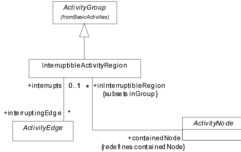
Figure 194 - Interruptible regions
