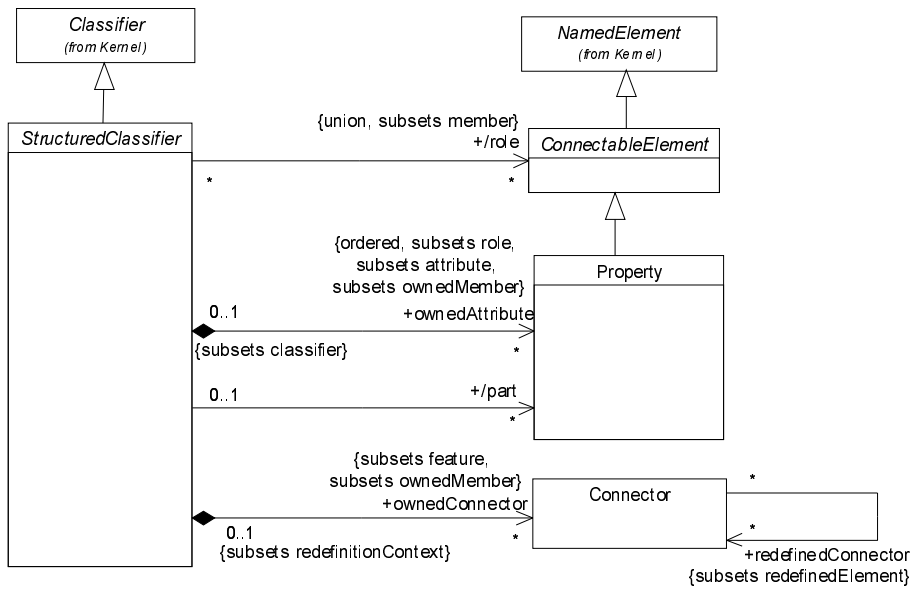
Figure 95 - Structured classifier
