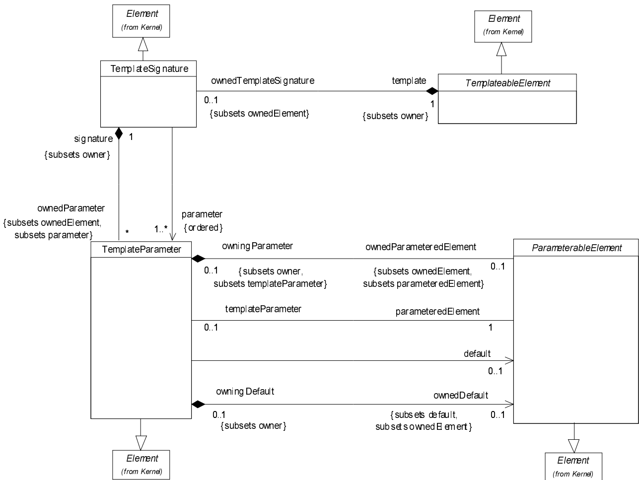
Figure 427 - Templates
