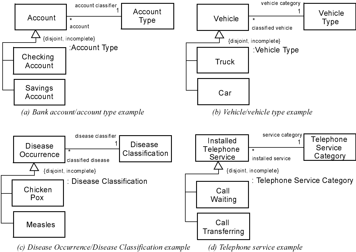
Figure 48 - Other power type examples
