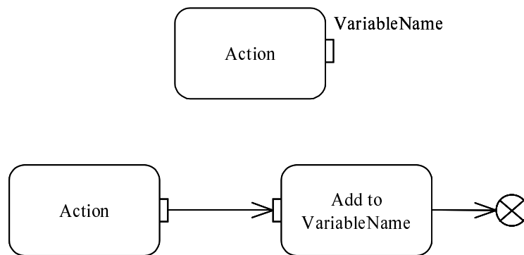
Figure 236 - Presentation option for AddVariableValueAction
