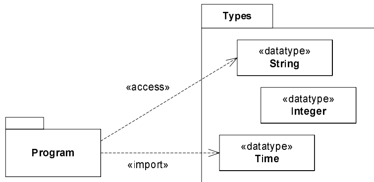
Figure 37 - Example of element import
