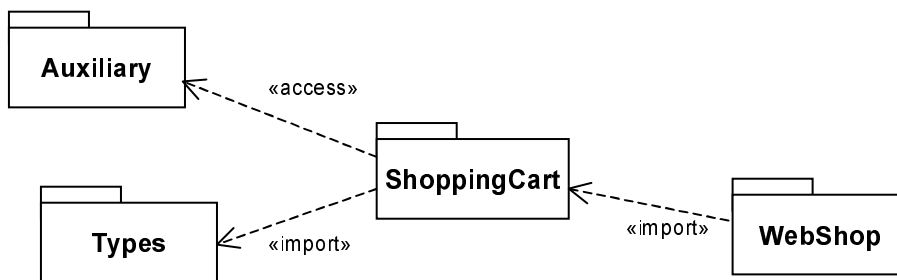
Figure 62 - Examples of public and private package imports
