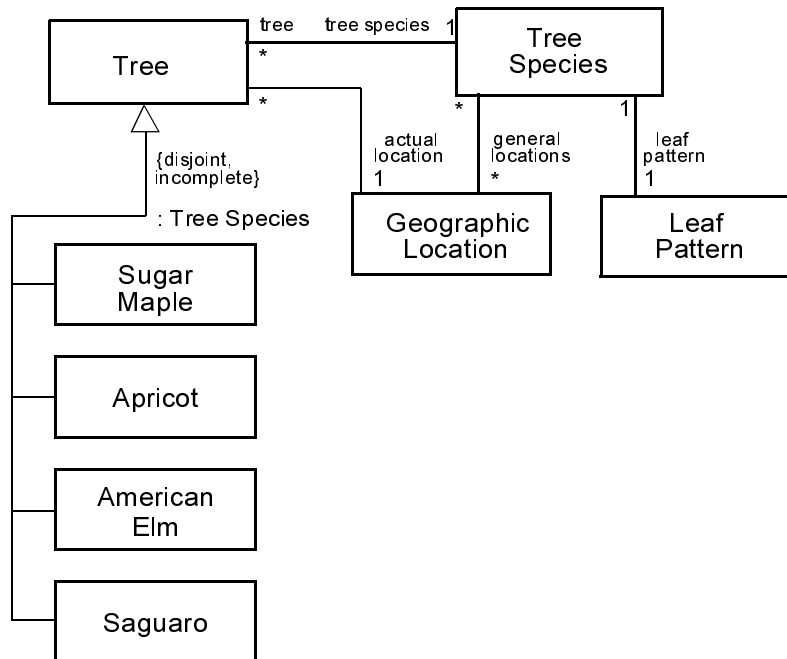
Figure 47 - Power type example and notation
