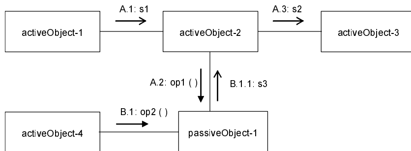
Figure 6 - Example illustrating the basic causality model of UML
