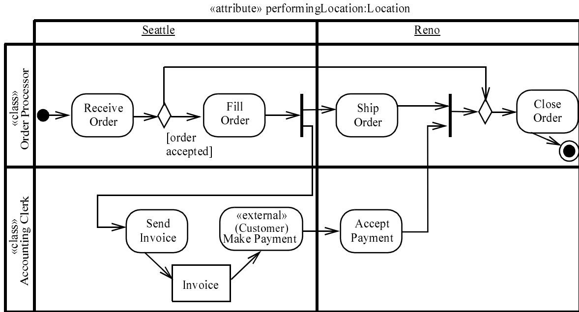
Figure 235 - Activity partition using multidimensional swimlane example
