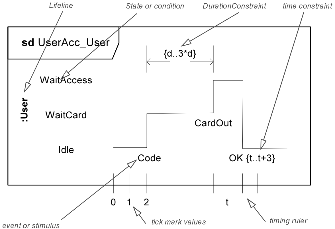
Figure 353 - A Lifeline for a discrete object
