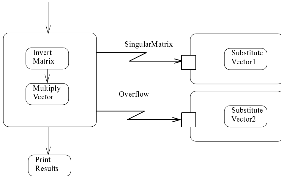
Figure 255 - Exception Handler example
