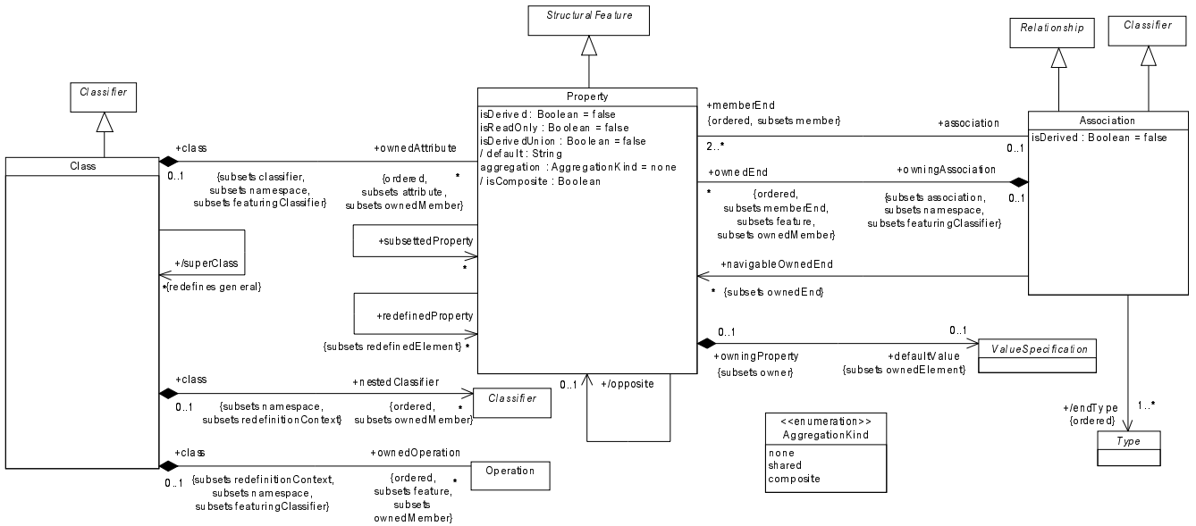
Figure 12 - The Classes diagram of the Kernel package
