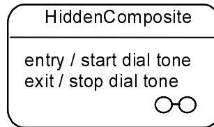
Figure 386 - Composite State with hidden decomposition indicator icon
