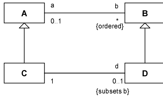
Figure 20 - Association ends with various adornments
