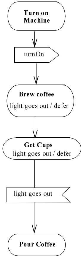
Figure 397 - Deferred Trigger Notation
