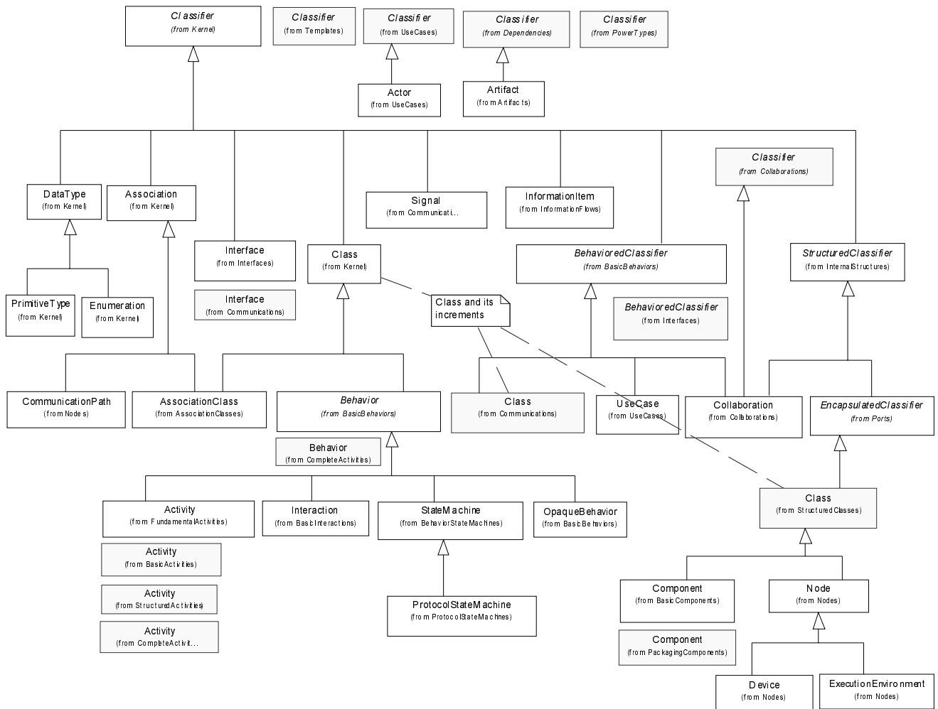
Figure 467 - Classifier hierarchy for UML 2.0 Superstructure
