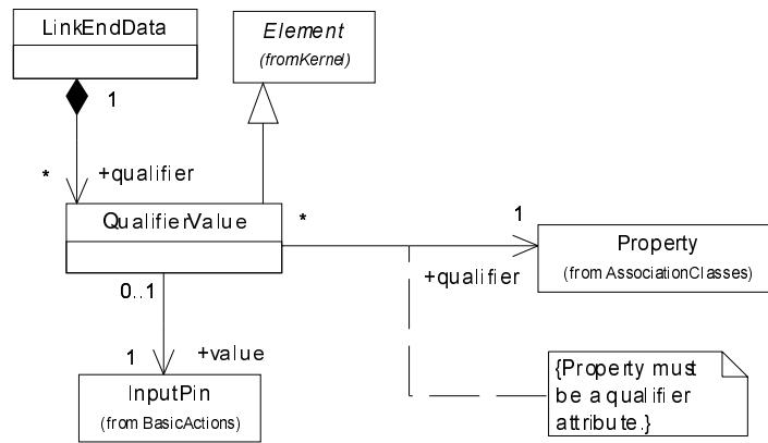
Figure 154 - Link identification (CompleteActions)
