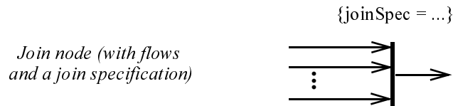
Figure 276 - Join node notations
