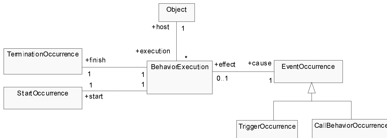
Figure 308 - Communication Domain Model
