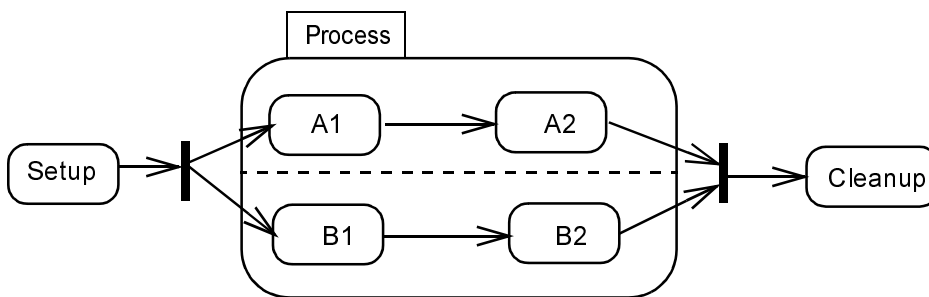
Figure 377 - Fork and Join
