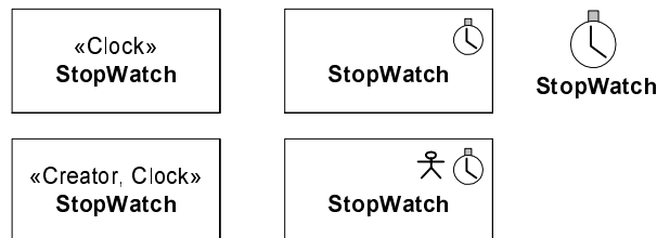
Figure 457 - Presentation options for an extended class
