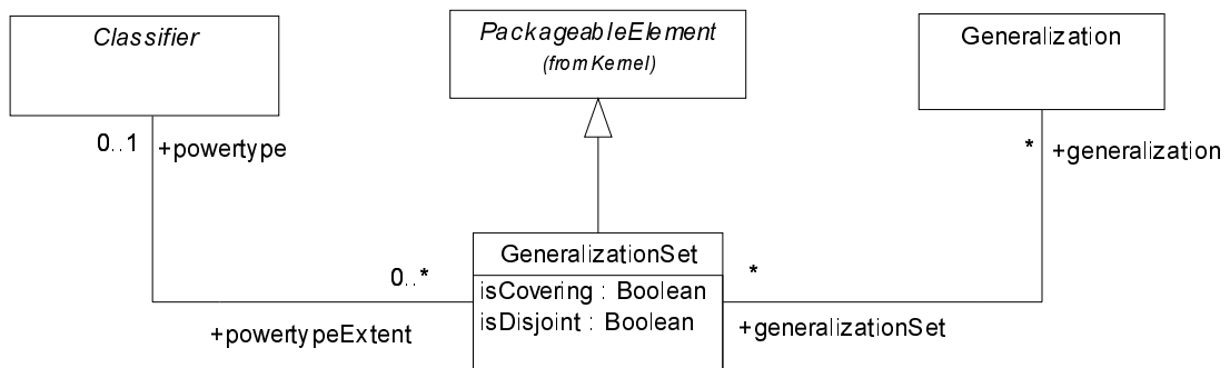
Figure 18 - The contents of PowerTypes package
