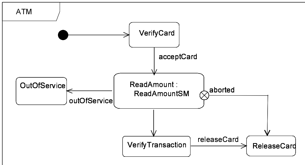
Figure 391 - SubmachineState with usage of exit point
