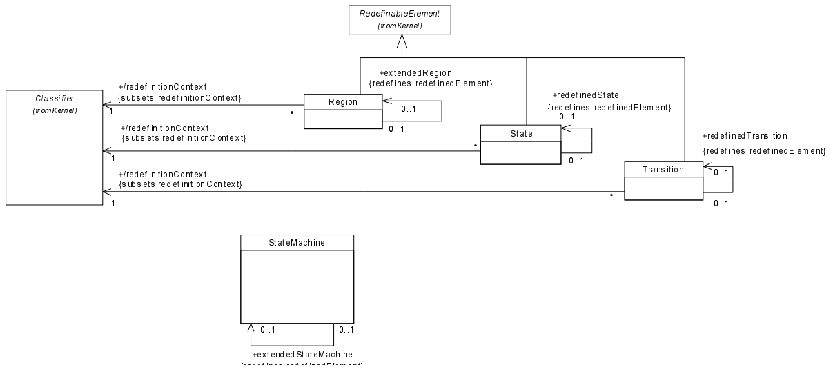
Figure 355 - State Machine Redefinitions
