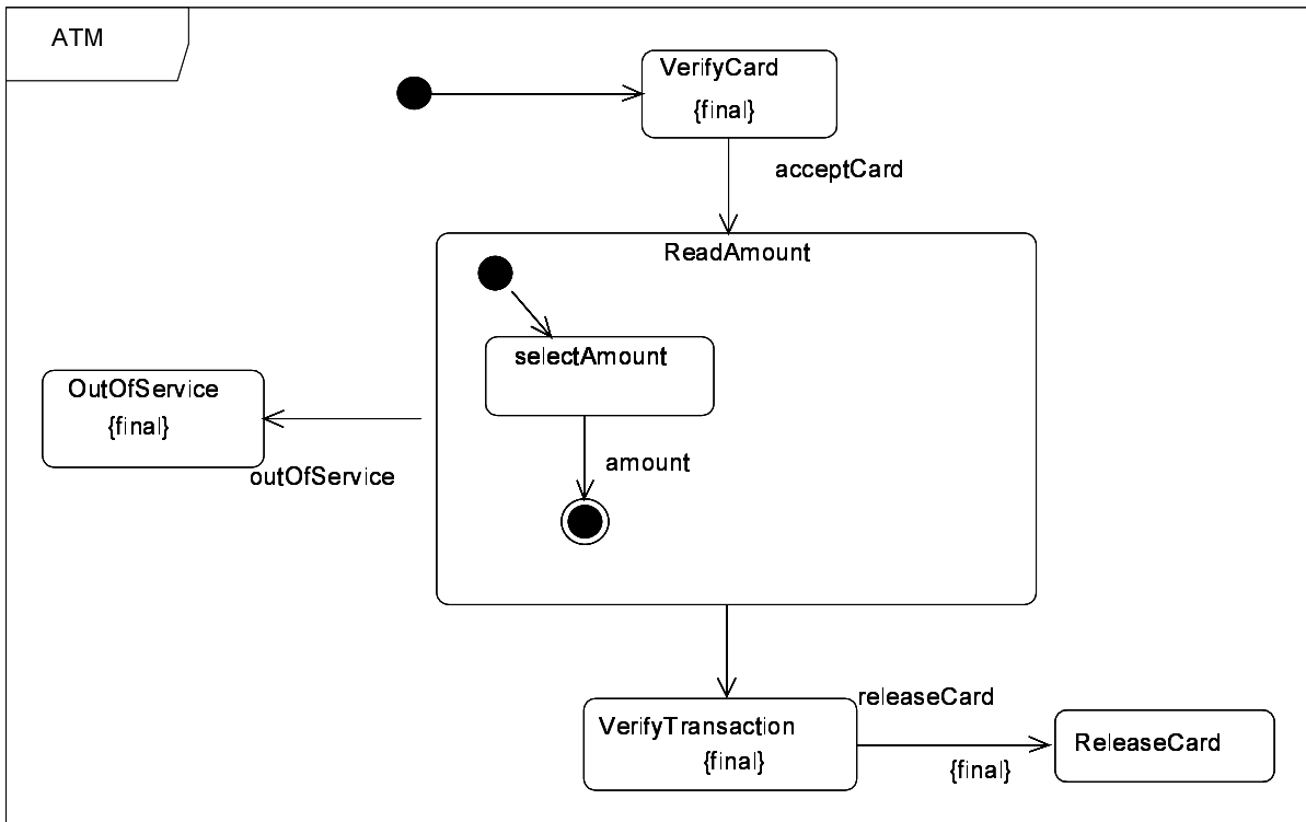
Figure 394 - A general state machine
