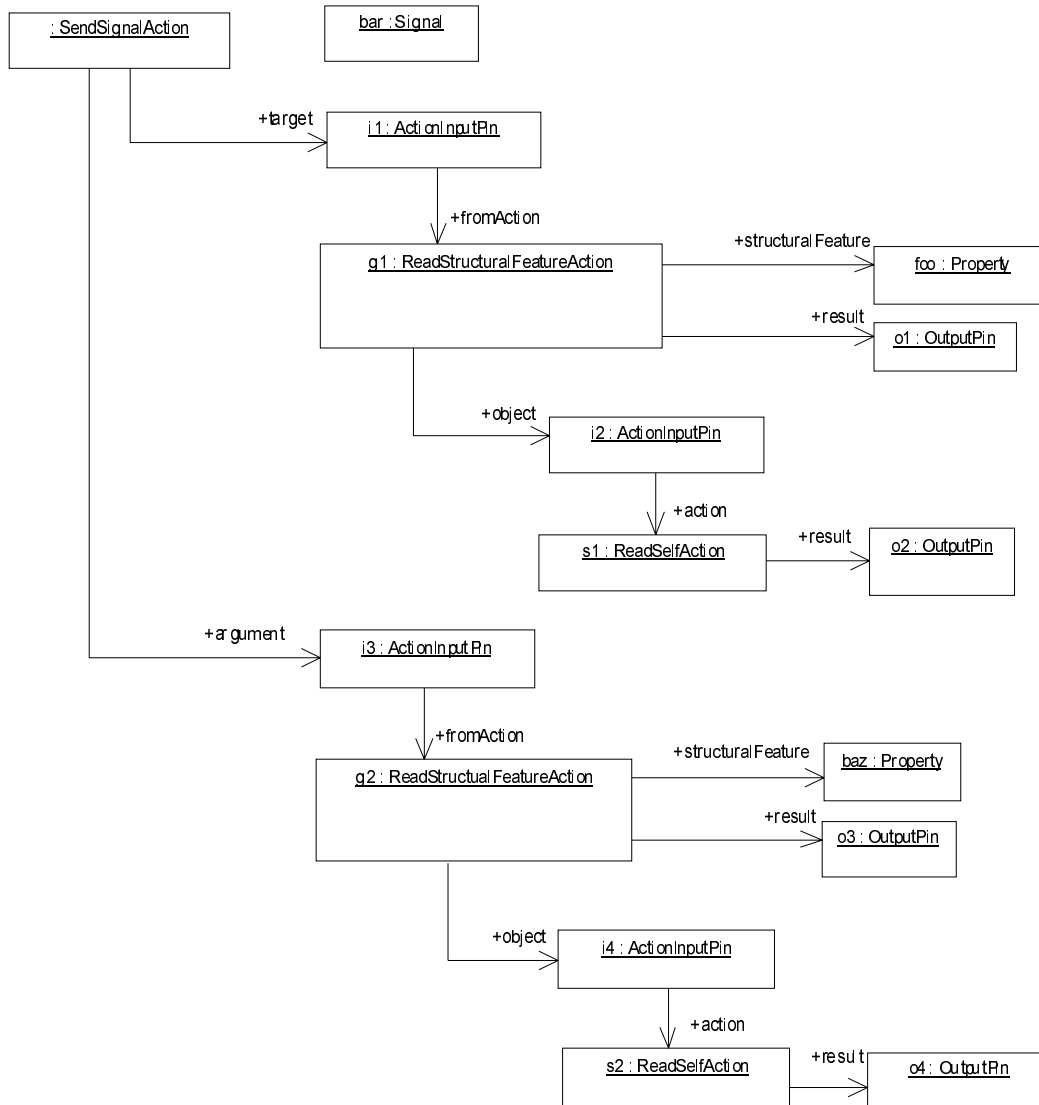
Figure 161 - Example repository model
