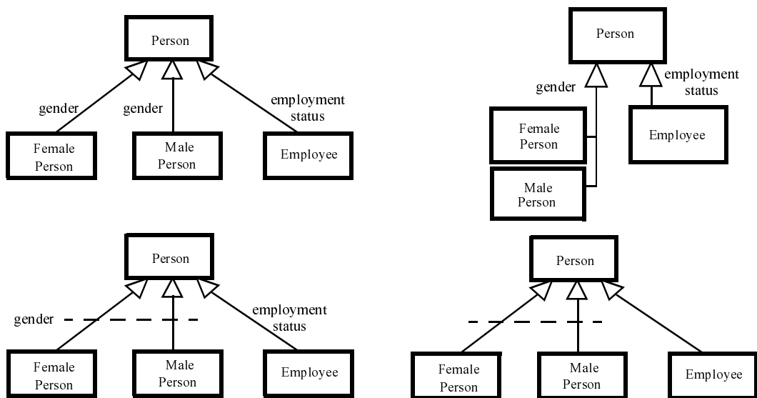
Figure 42 - Multiple subtype partitions (GeneralizationSets) example
