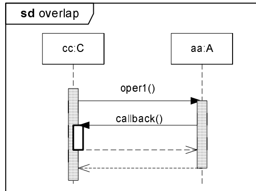
Figure 339 - Overlapping execution occurrences
