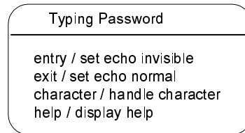
Figure 384 - State with compartments
