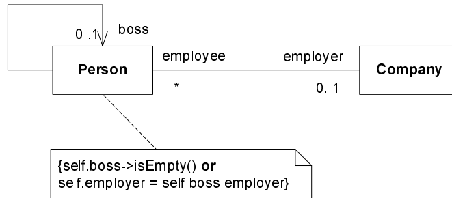
Figure 33 - Constraint in a note symbol
