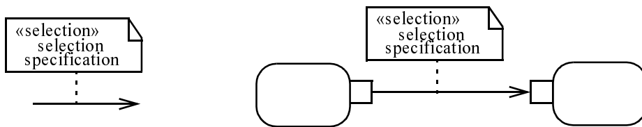
Figure 282 - Specifying selection behavior on an Object flow
