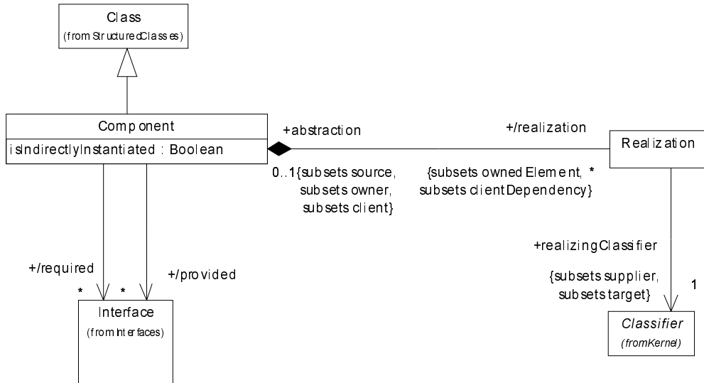
Figure 77 - The metaclasses that define the basic Component construct.
