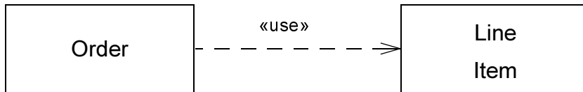
Figure 73 - An example of a use dependency
