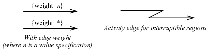
Figure 215 - Activity edge notation
