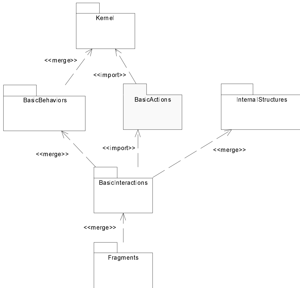
Figure 325 - Dependencies of the Interactions packages
