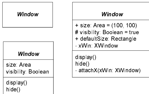
Figure 26 - Class notation: details suppressed, analysis-level details, implementation-level details
