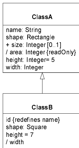
Figure 28 - Examples of attributes
