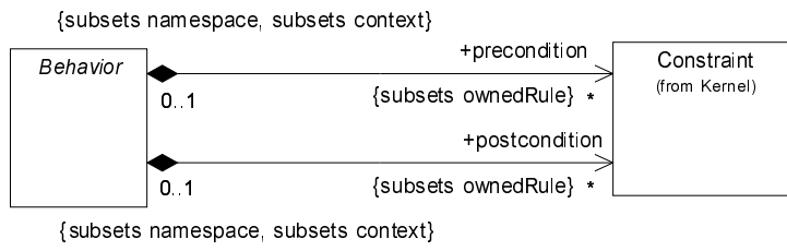
Figure 313 - Precondition and postcondition constraints for behavior
