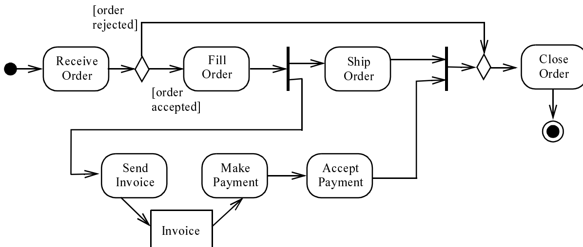
Figure 247 - Control node examples (with accompanying actions and control flows)
