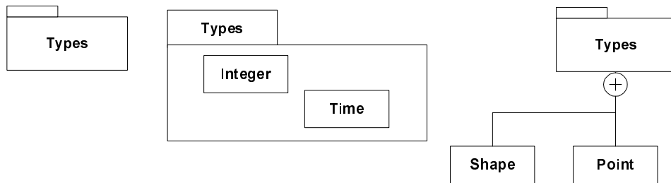
Figure 61 - Examples of a package with members
