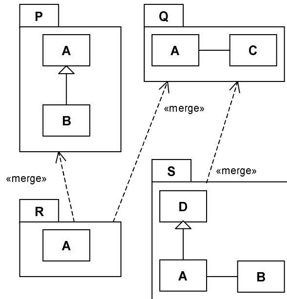
Figure 66 - Simple example of package merges
