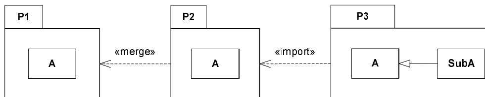
Figure 63 - Illustration of the meaning of package merge
