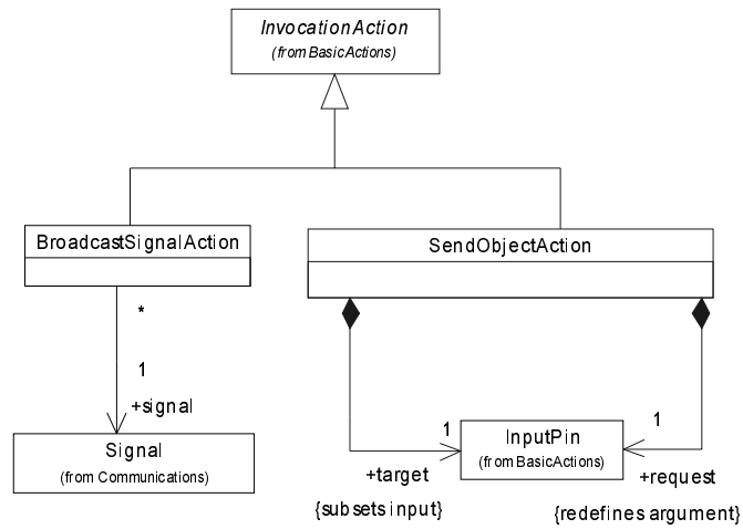
Figure 145 - Intermediate invocation actions
