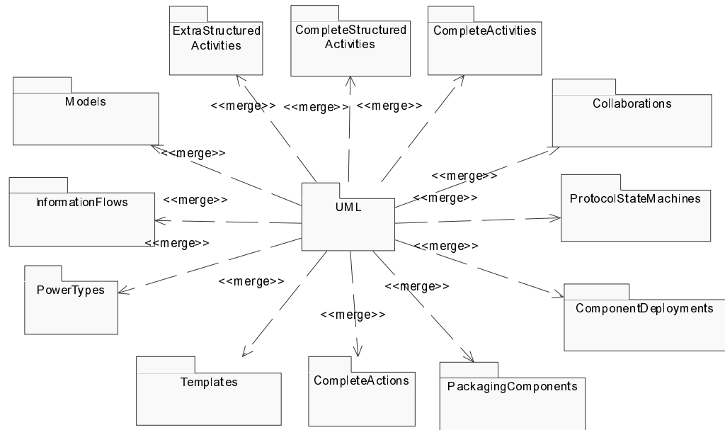
Figure 4 - Level 3 top-level package merges
