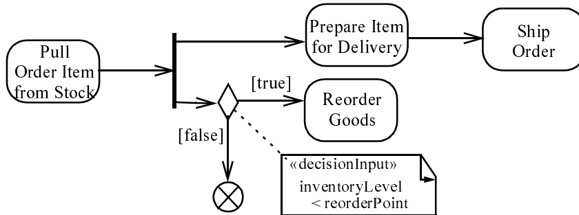
Figure 252 - Decision node example
