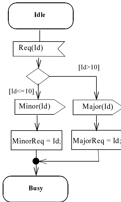
Figure 396 - Symbols for Signal Receipt, Sending and Actions on transition
