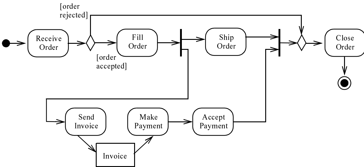
Figure 225 - Activity node example (where the arrowed lines are only the non-activity node symbols)
