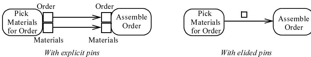
Figure 285 - Eliding objects flowing on the edge
