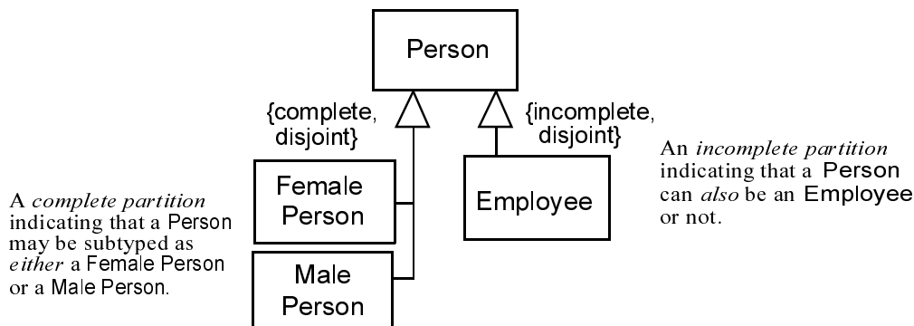
Figure 46 - Multiple ways of dividing subtypes (generalization sets) and constraint examples
