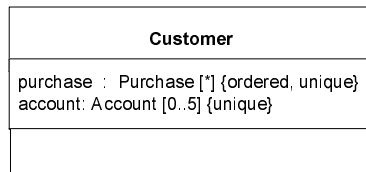
Figure 59 - Multiplicity within a textual specification
