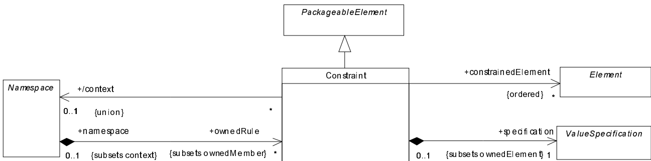
Figure 7 - The Constraints diagram of the Kernel package
