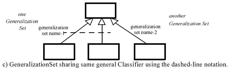
Figure 40 - GeneralizationSet designation notations
