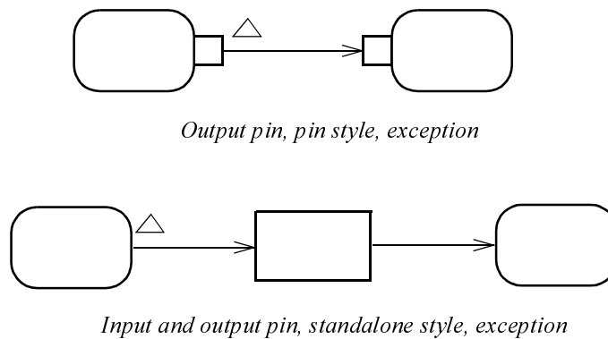
Figure 296 - Exception pin notations
