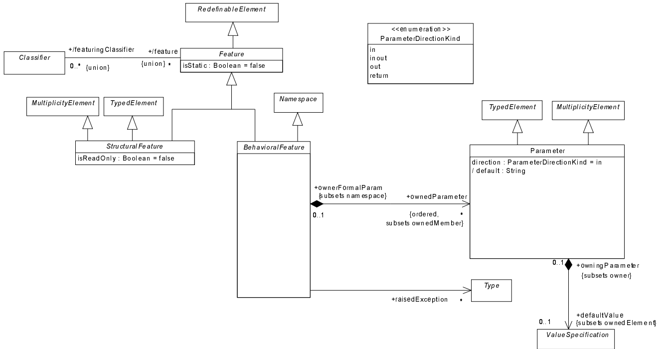
Figure 10 - The Features diagram of the Kernel package
