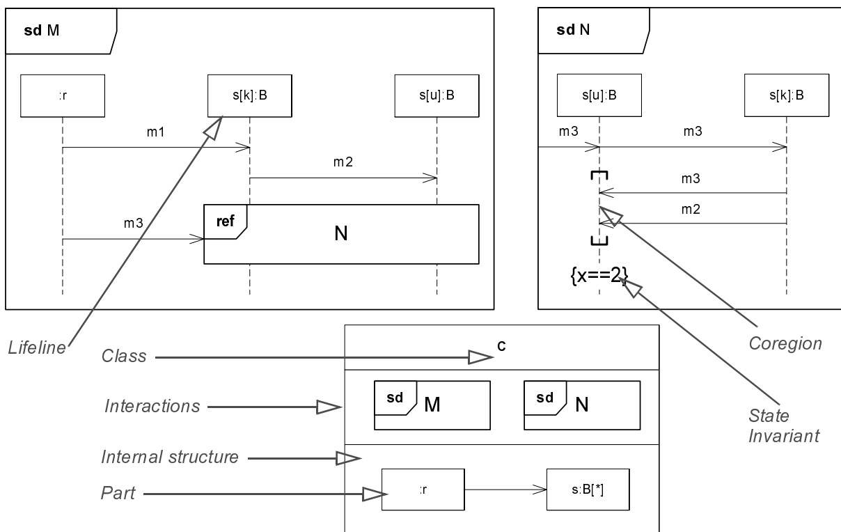
Figure 346 - Sequence Diagrams where two Lifelines refer to the same set of Parts (and Internal Structure)
