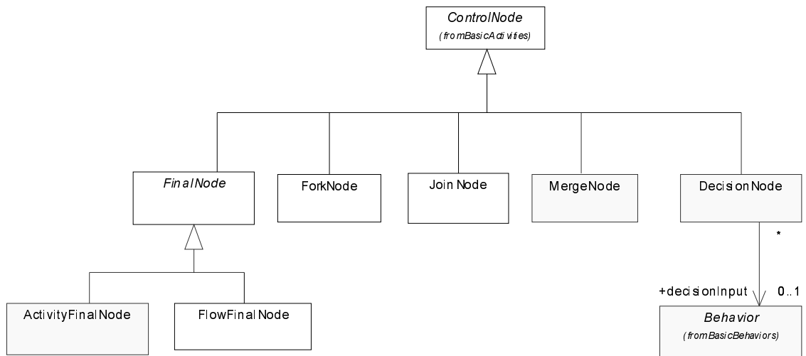
Figure 183 - Control nodes (IntermediateActivities)
