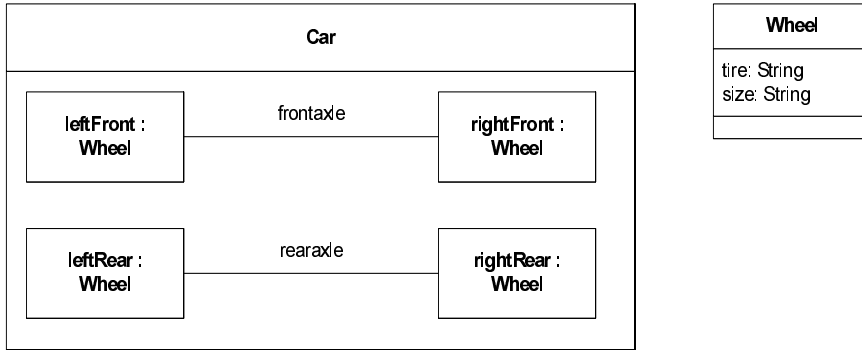
Figure 118 - Connectors and parts in a structure diagram
