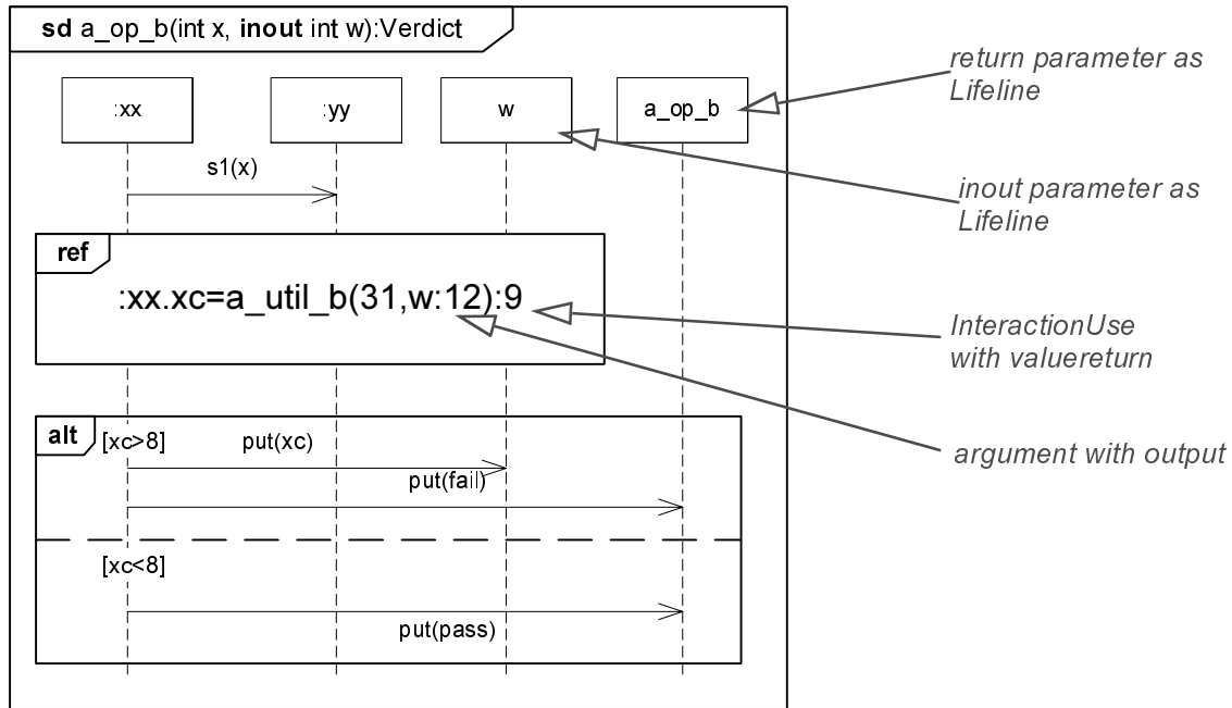
Figure 342 - InteractionUse with value return
