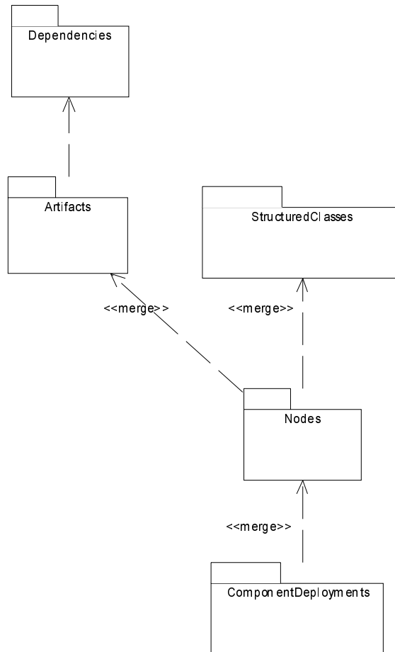
Figure 123 - Dependencies between packages described in this chapter
