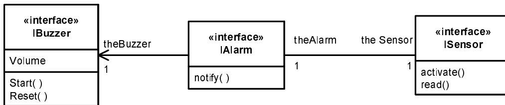
Figure 57 - A set of collaborating interfaces
