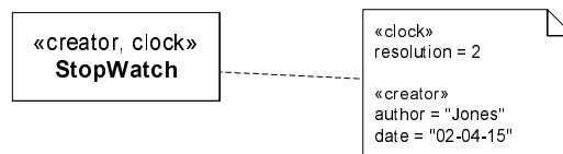
Figure 462 - Using stereotypes and showing values
