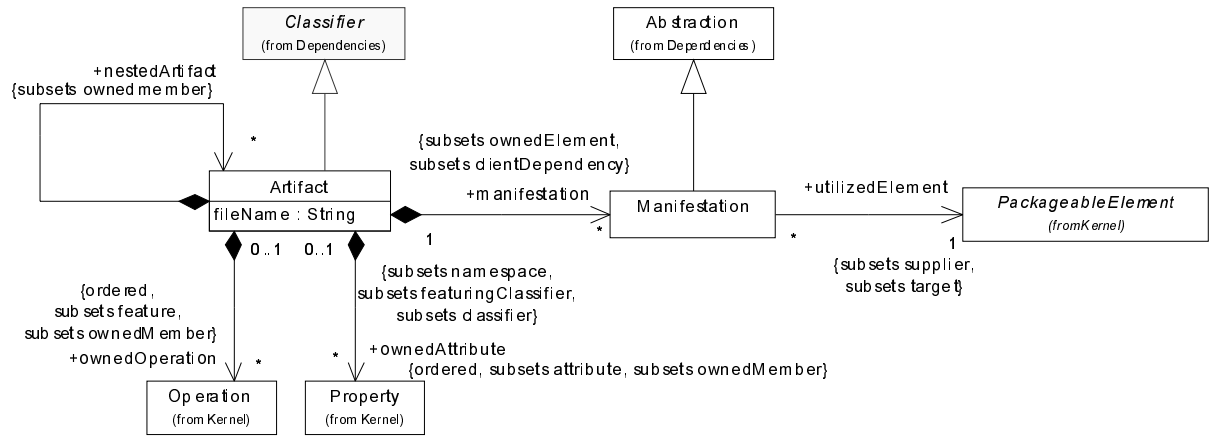
Figure 124 - The elements defined in the Artifacts package
