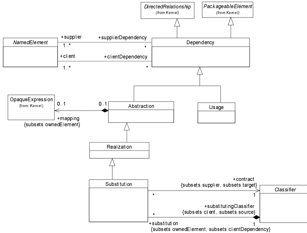
Figure 15 - The contents of Dependencies package
