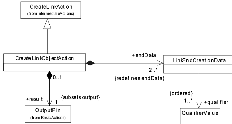
Figure 156 - Write link actions (CompleteActions)
