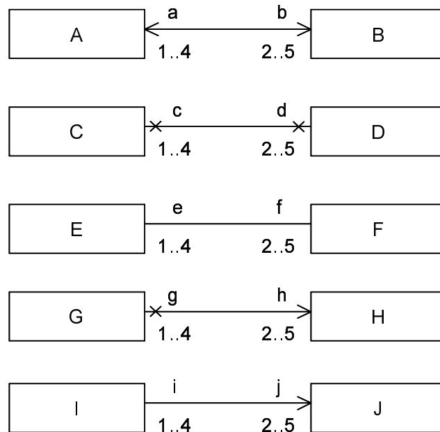
Figure 21 - Examples of navigable ends
