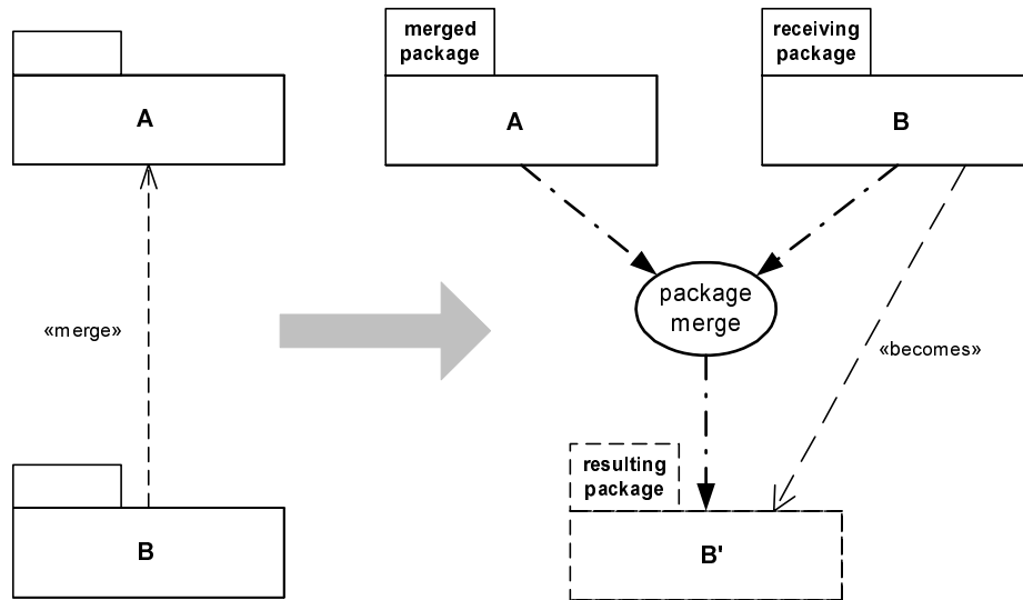
Figure 64 - Conceptual view of the package merge semantics
