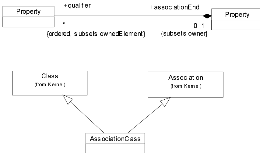
Figure 17 - The contents of AssociationClasses package
