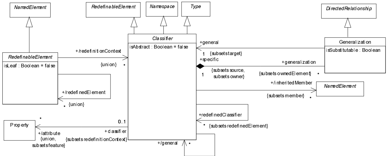
Figure 9 - The Classifiers diagram of the Kernel package
