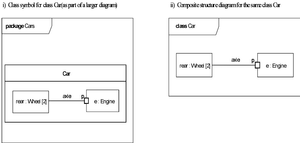
Figure 463 - A class diagram and a composite structure diagram
