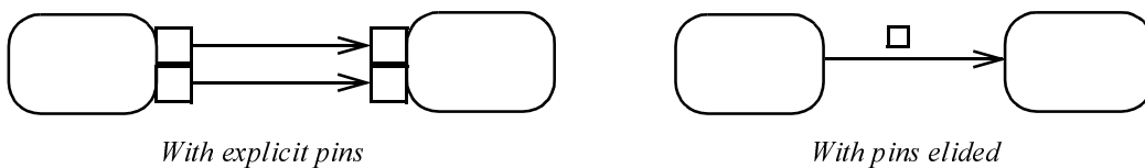
Figure 283 - Eliding objects flowing on the edge
