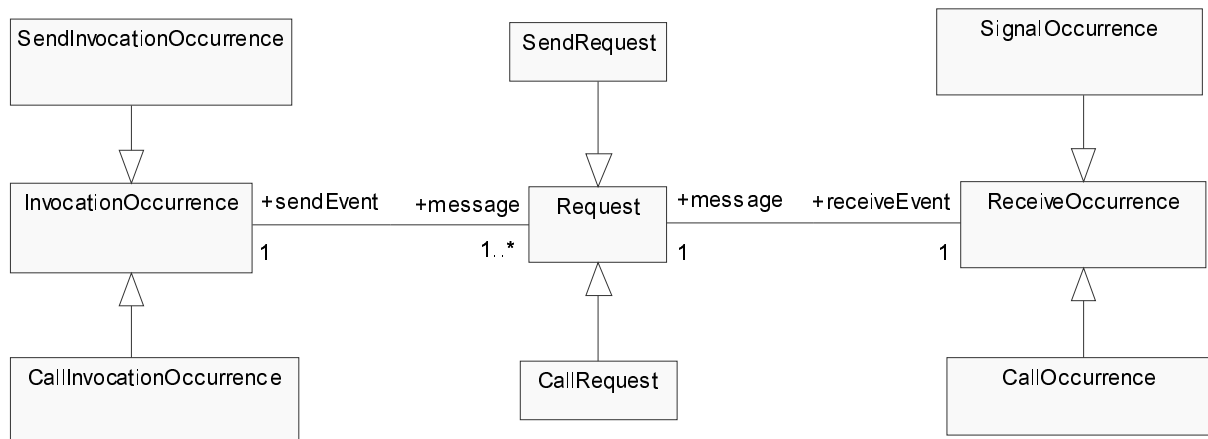
Figure 309 - Domain Model Showing Request Kinds
