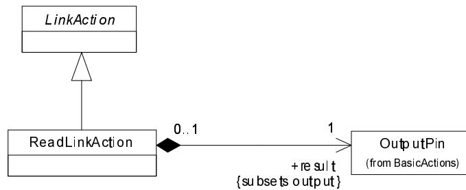
Figure 149 - Read link actions
