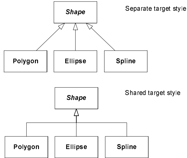
Figure 41 - Examples of generalizations between classes
