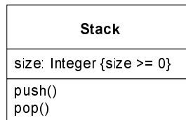
Figure 31 - Constraint attached to an attribute
