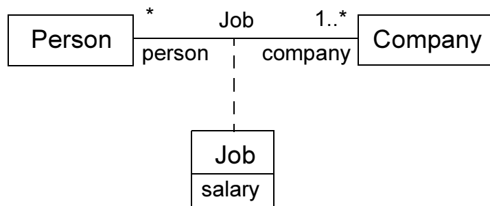
Figure 25 - An AssociationClass is depicted by an association symbol (a line) and a class symbol (a box) connected with a dashed line. The diagram shows the association class Job which is defined between the two classes Person and Company.
