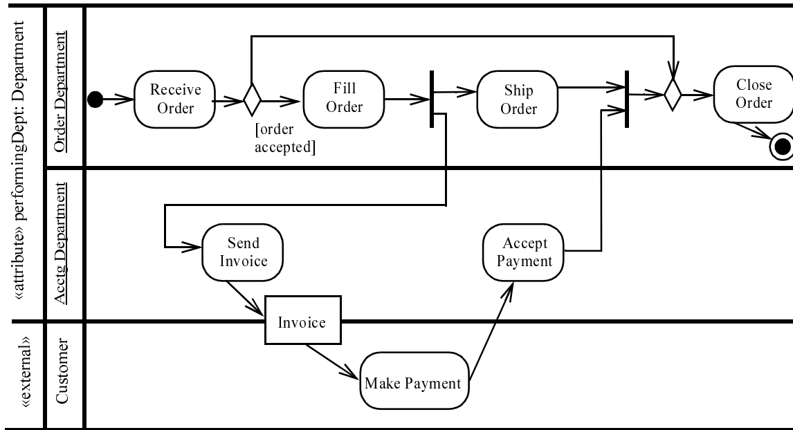
Figure 233 - Activity partition using swim lane example
