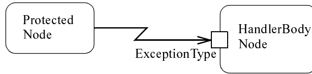
Figure 253 - Exception Handler Notation
