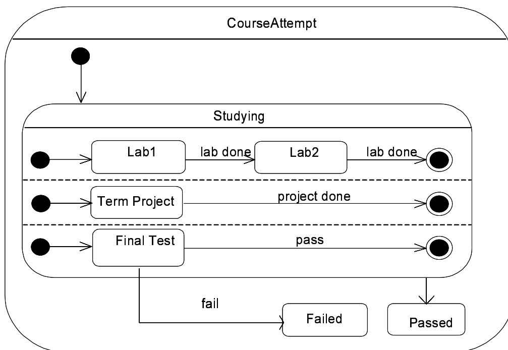
Figure 387 - Orthogonal state with regions
