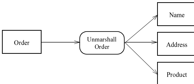
Figure 307 - Example of UnmarshallAction
