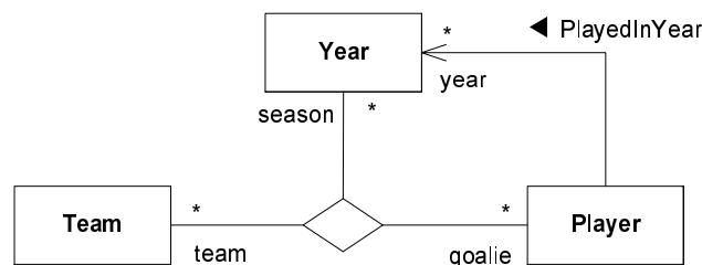
Figure 19 - Binary and ternary associations
