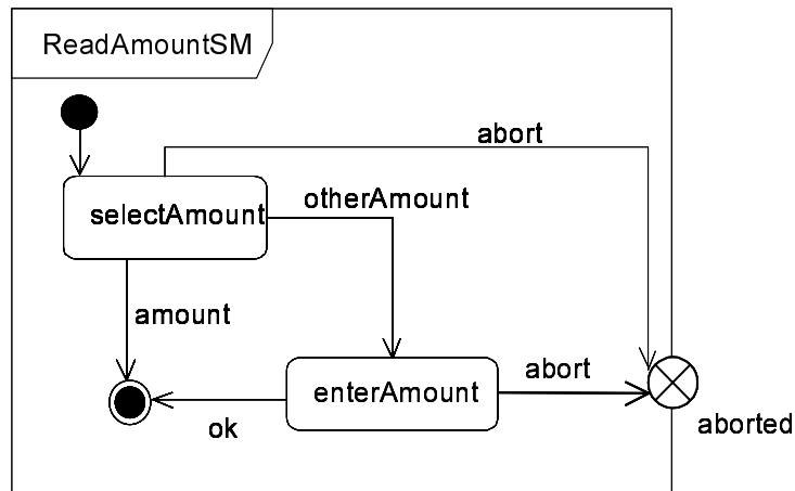
Figure 390 - State machine with exit point on the border of the statemachine
