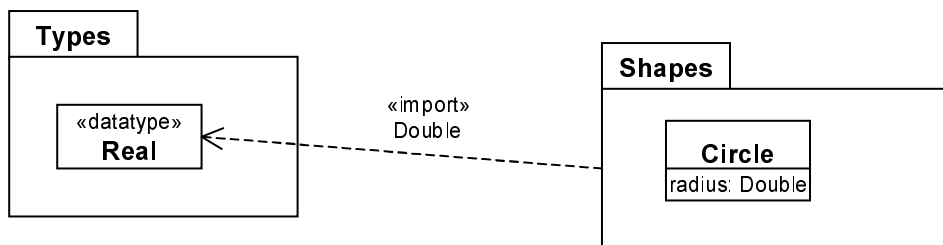
Figure 38 - Example of element import with aliasing
