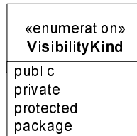
Figure 39 - Example of an enumeration
