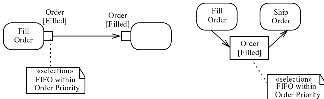
Figure 304 Specifying selection behavior on an ObjectFlow
