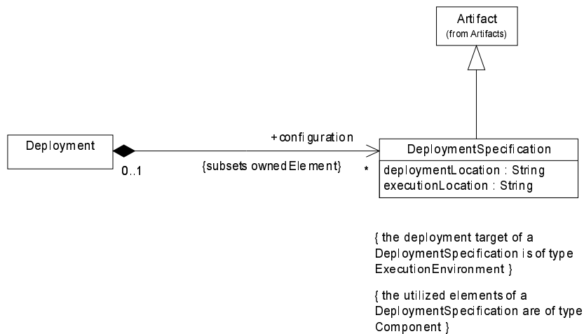
Figure 127 - The metaclasses that define component Deployment
