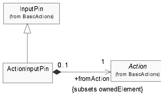
Figure 159 - Action input pin
