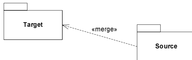
Figure 65 - Notation for package merge
