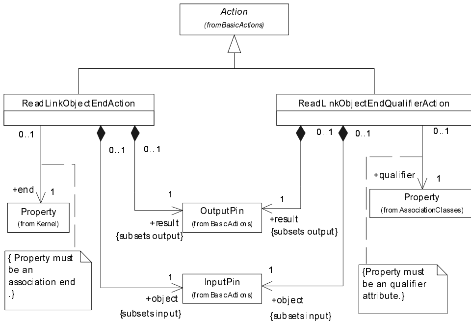
Figure 155 - Read link actions (CompleteActions)
