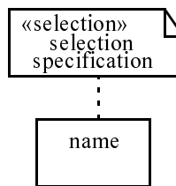
Figure 290 - Specifying selection behavior on an Object node
