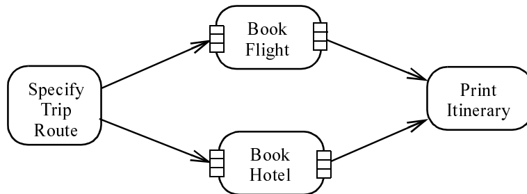
Figure 262 -Examples of expansion region shorthand
