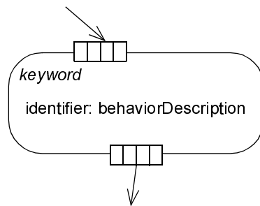
Figure 257 - Shorthand notation for expansion region containing single node
