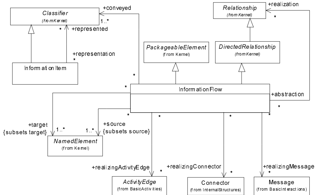
Figure 413 - The contents of the InformationFlows package
