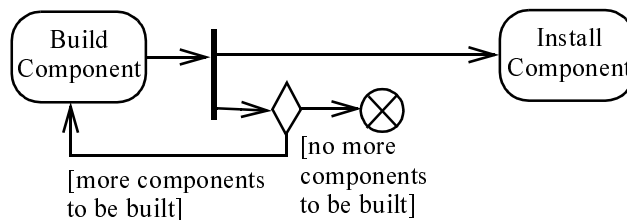
Figure 267 - Flow final example without merge edge
