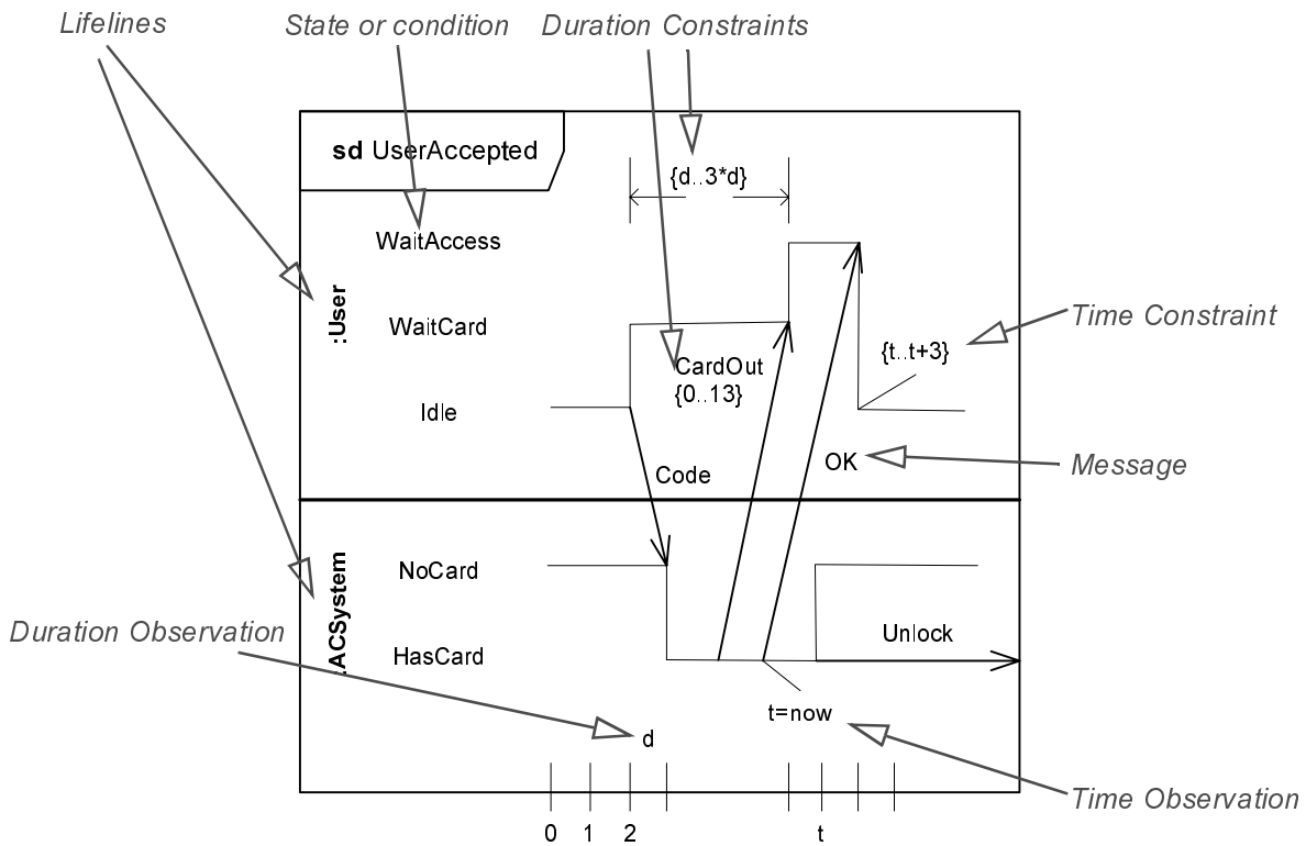
Figure 355 - Timing Diagram with more than one Lifeline and with Messages
