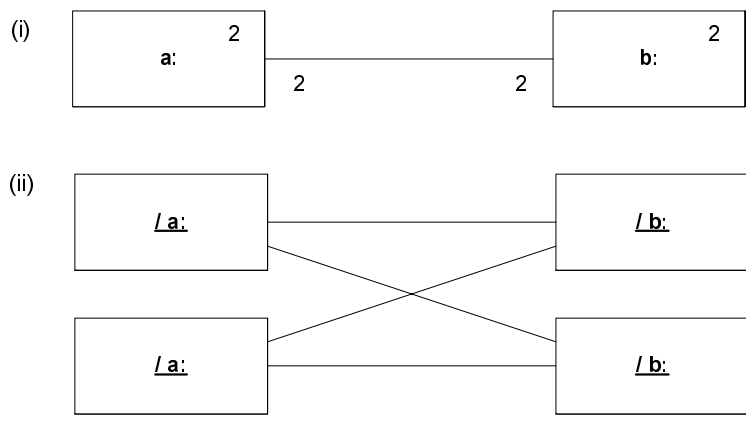
Figure 116 - “Star” connector pattern
