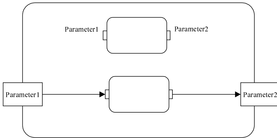
Figure 228 - Presentation option for flows between pins and parameter nodes
