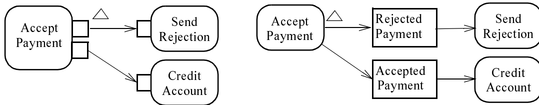
Figure 303 - Exception pin examples
