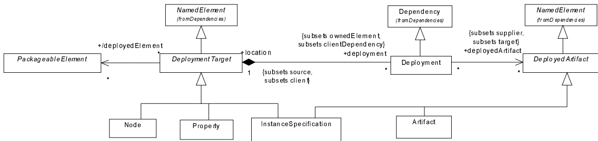
Figure 126 - The definition of the Deployment relationship between DeploymentTargets and DeployedArtifacts.
