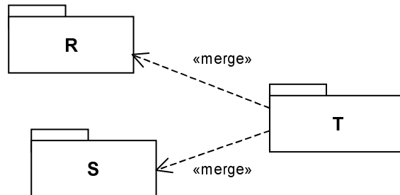
Figure 68 - Introducing additional package merges
