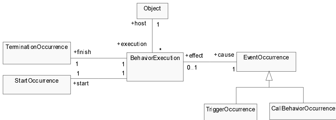
Figure 307 - Invocation Domain Model
