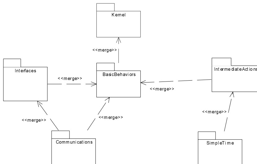
Figure 310 - Dependencies of the CommonBehaviors packages
