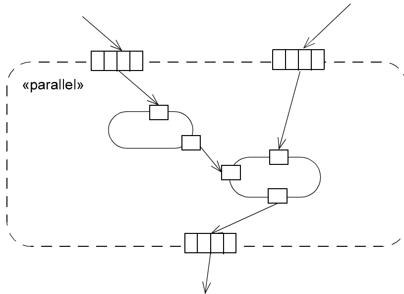
Figure 260 - Expansion region with 2 inputs and 1 output
