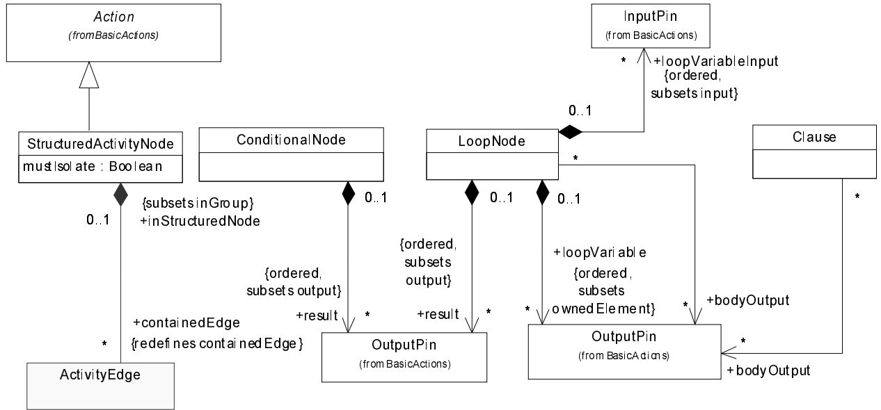
Figure 196 - Structured nodes (CompleteStructuredActivities)
