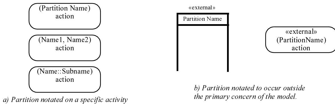
Figure 232 - Activity partition notations
