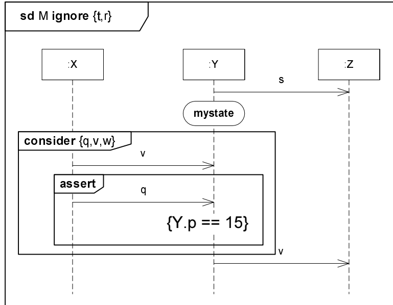
Figure 348 - Ignore, Consider, assert with State Invariants
