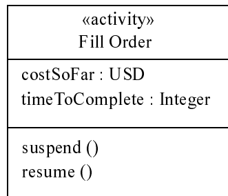
Figure 212 - Activity class with attributes and operations
