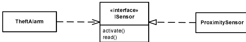
Figure 55 - Alternative notation for the situation depicted in Figure 53 and Figure 54
