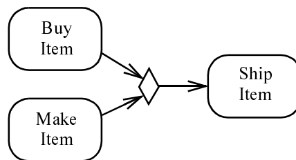
Figure 280 - Merge node example
