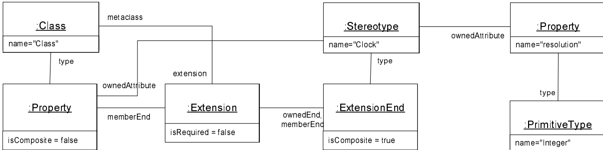
Figure 458 - An instance specification when defining a stereotype
