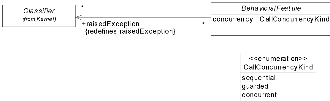
Figure 315 - Extensions to behavioral features
