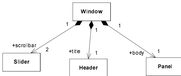
Figure 24 - Composite aggregation is depicted as a black diamond
