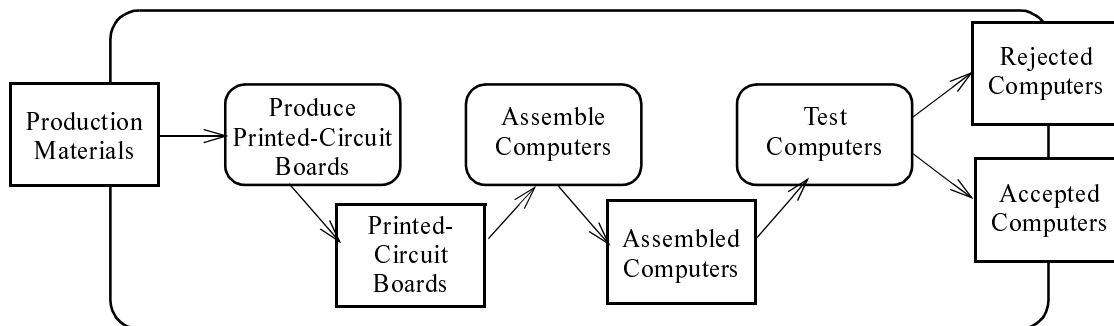
Figure 229 - Example of activity parameters.nodes
