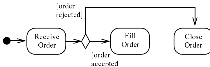
Figure 251 - Decision node example.
