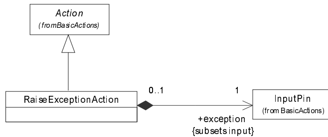
Figure 158 - Raise exception action
