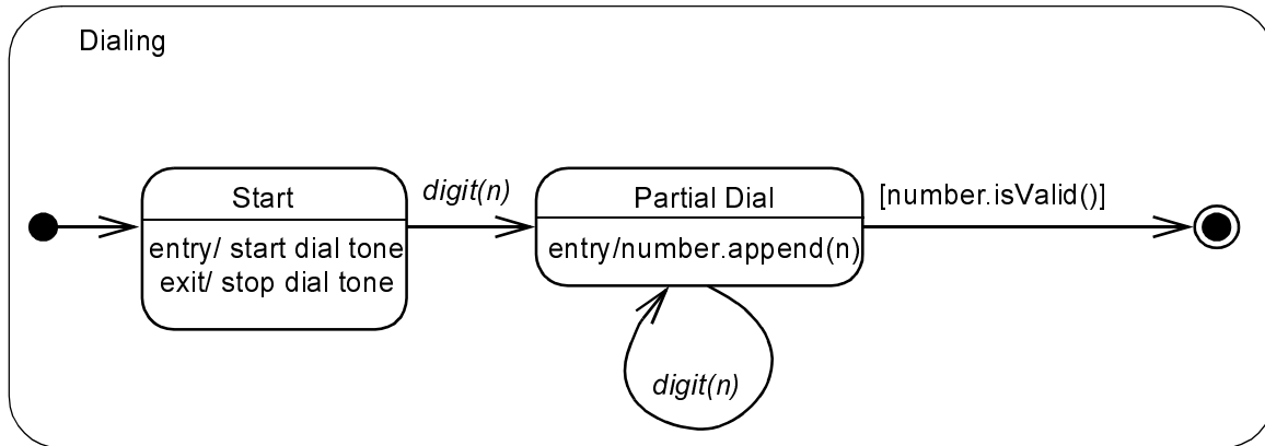
Figure 385 - Composite state with two states
