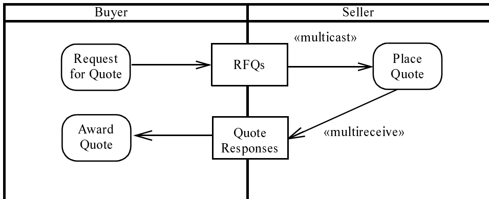
Figure 287 - Specifying multicast and multireceive on the edge
