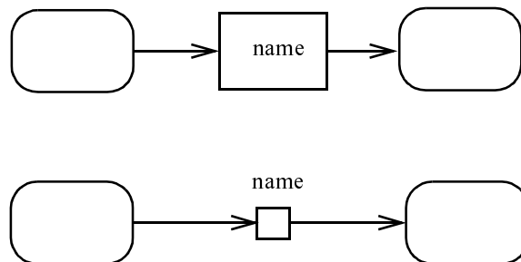
Figure 294 - Standalone pin notations
