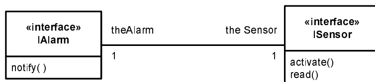
Figure 56 - IAlarm is the required interface for any classifier implementing ISensor; conversely, ISensor is the required interface for any classifier implementing IAlarm.
