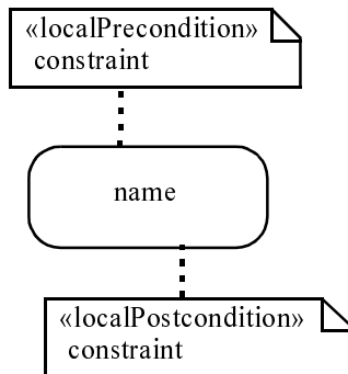
Figure 203 - Local pre- and postconditions
