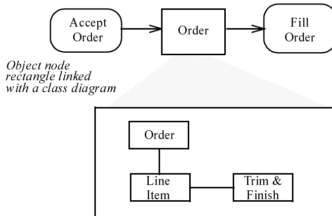
Figure 301 - Linking a class diagram to an object node
