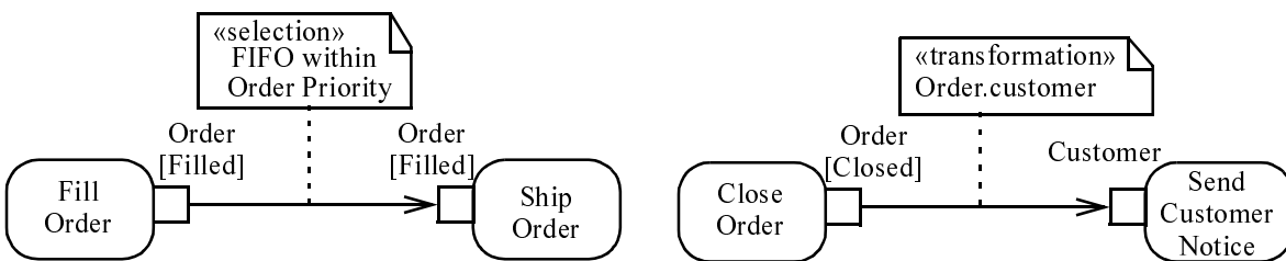
Figure 286 - Specifying selection behavior on an Object flow
