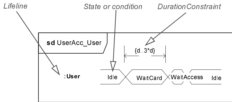
Figure 354 - Compact Lifeline with States
