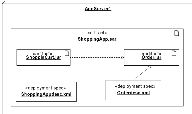
Figure 134 - DeploymentSpecifications related to the artifacts that they parameterize
