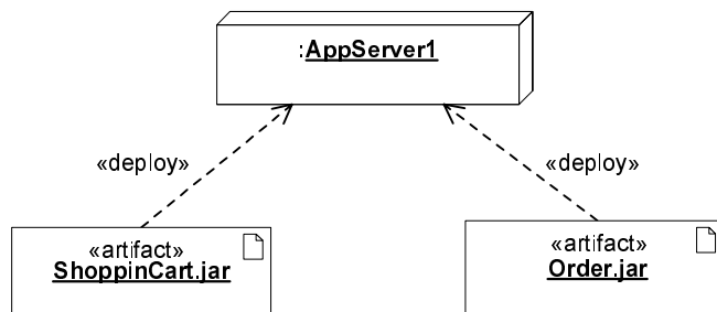
Figure 131 - An alternative deployment representation of using a dependency called «deploy» .
