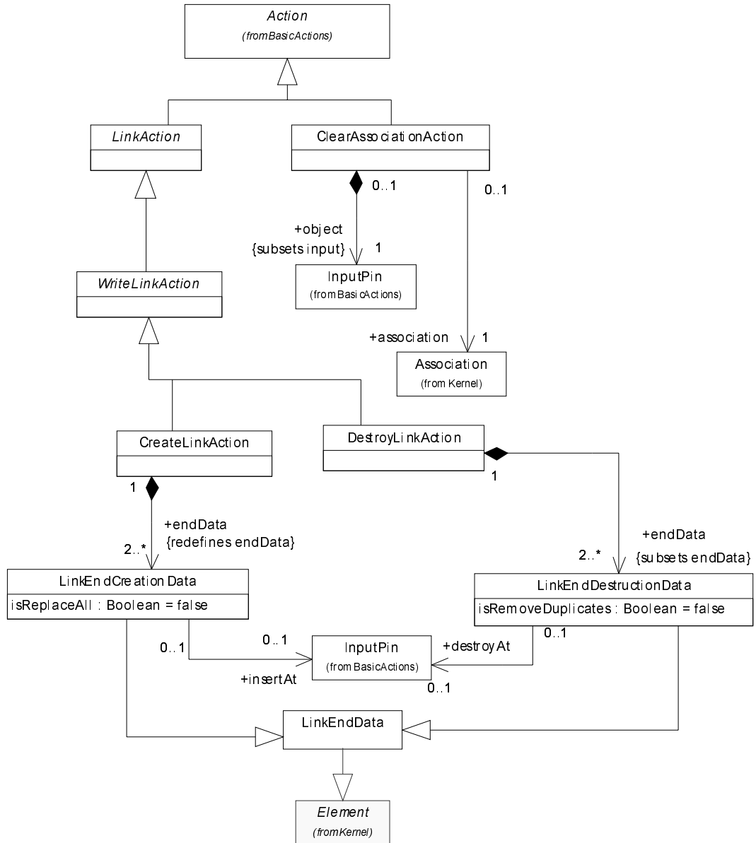
Figure 150 - Write link actions
