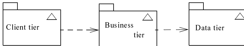
Figure 420 - Three models representing parts of a system
