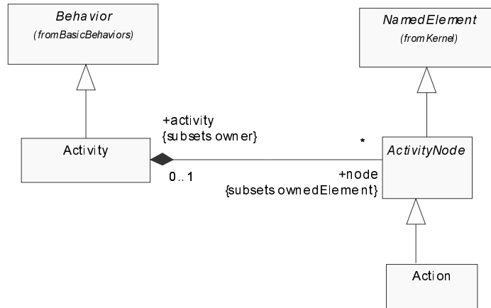
Figure 176 - Fundamental nodes
