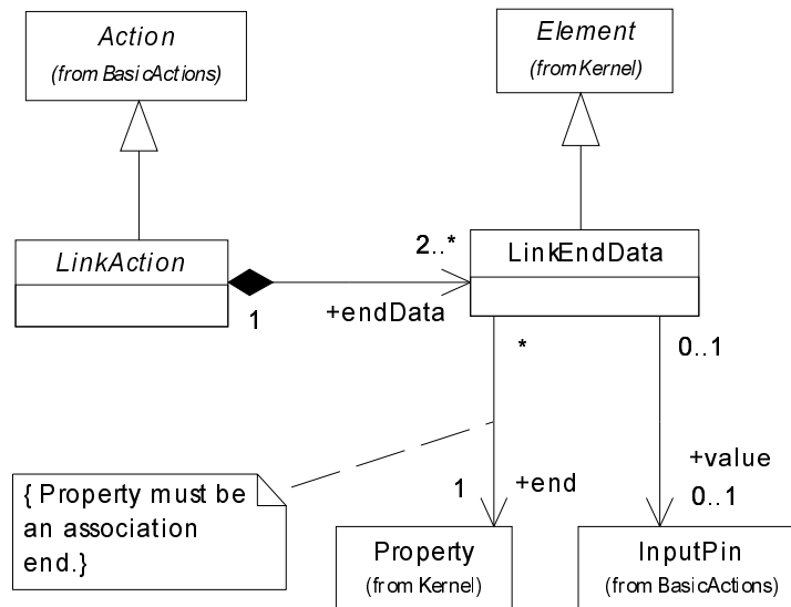
Figure 148 - Link identification
