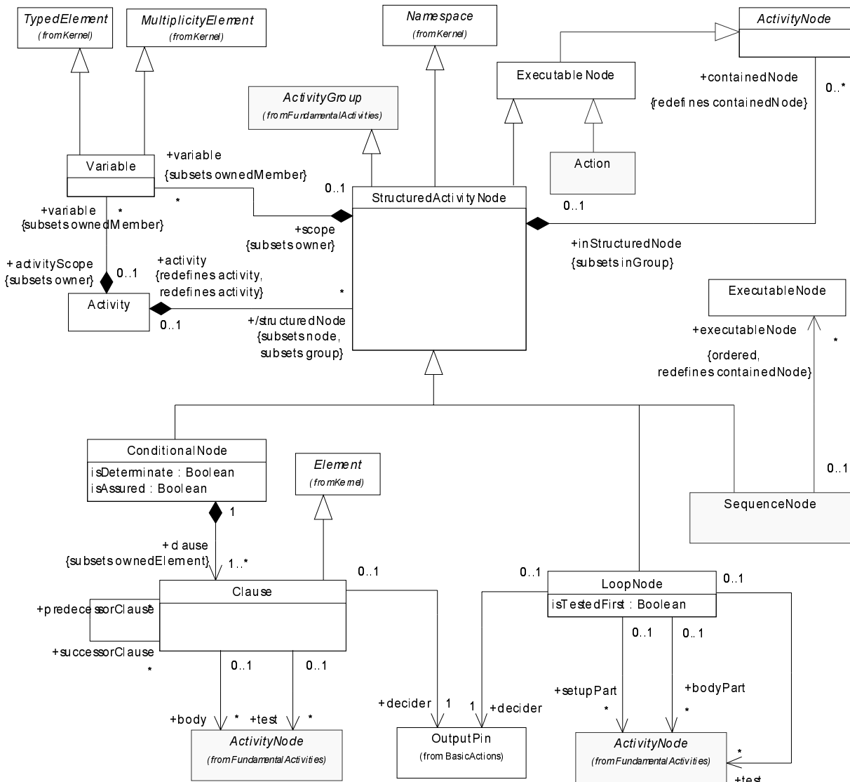
Figure 195 - Structured nodes
