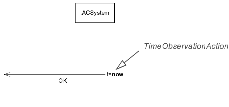
Figure 324 - Time observation
