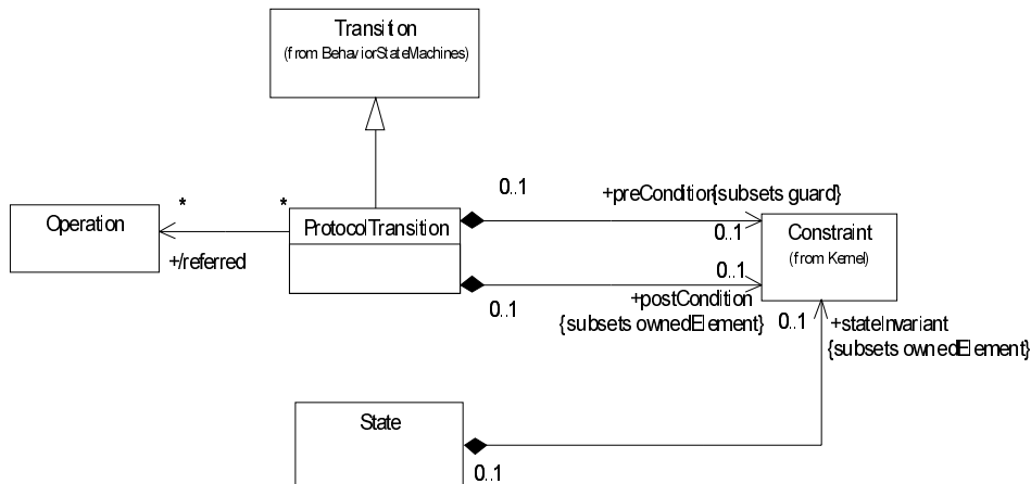
Figure 358 - Constraints
