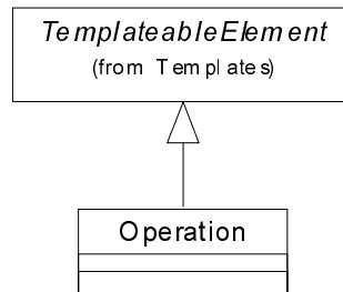
Figure 440 - Operation templates
