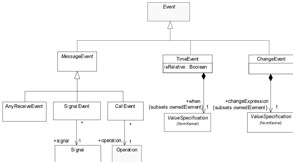
Figure 317 - Events
