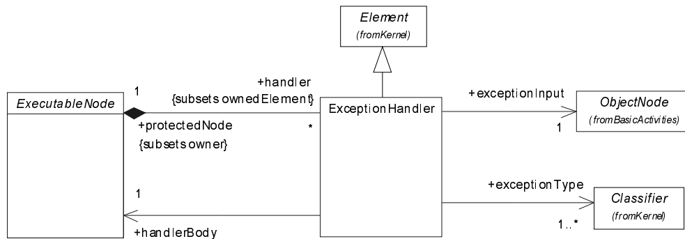
Figure 197 - Exceptions
