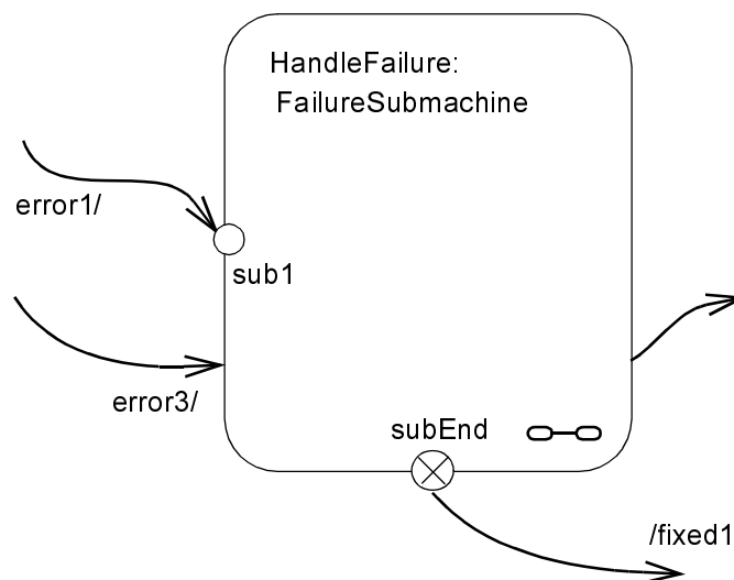
Figure 388 - Submachine State
