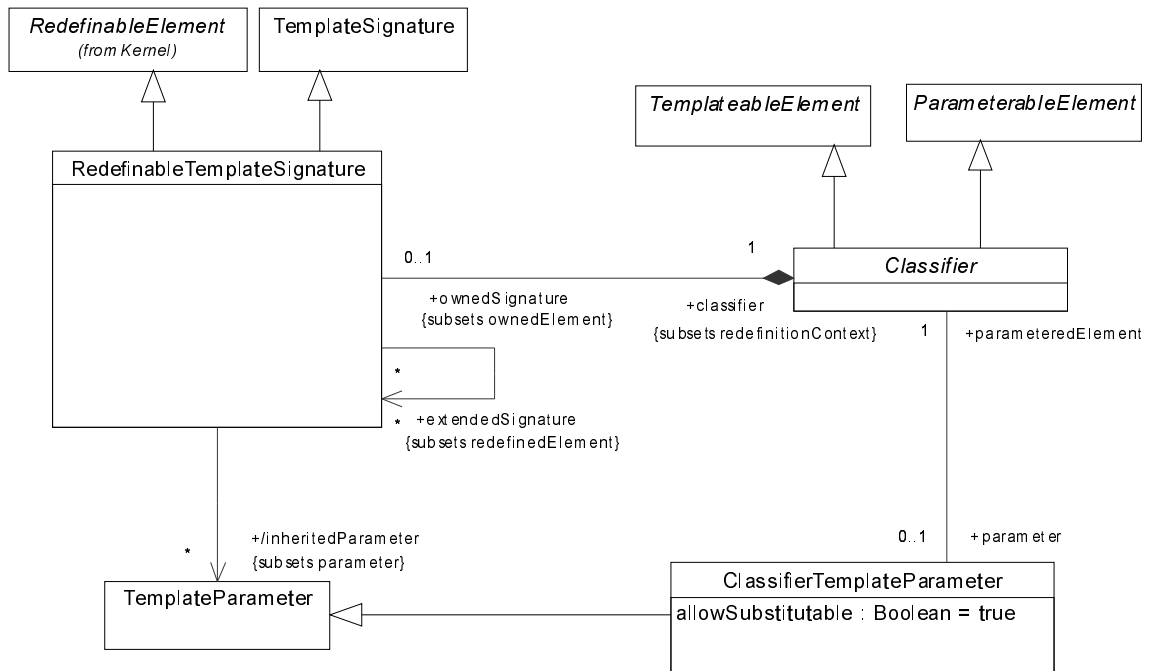
Figure 429 - Classifier templates
