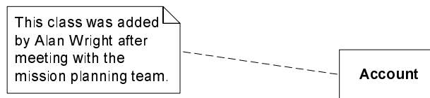
Figure 30 - Comment notation
