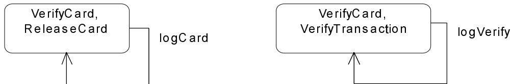
Figure 380 - State Lists
