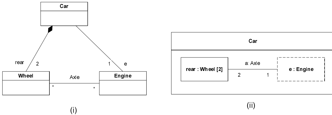
Figure 114 - Properties
