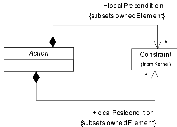
Figure 187 - Constraints (CompleteActivities)
