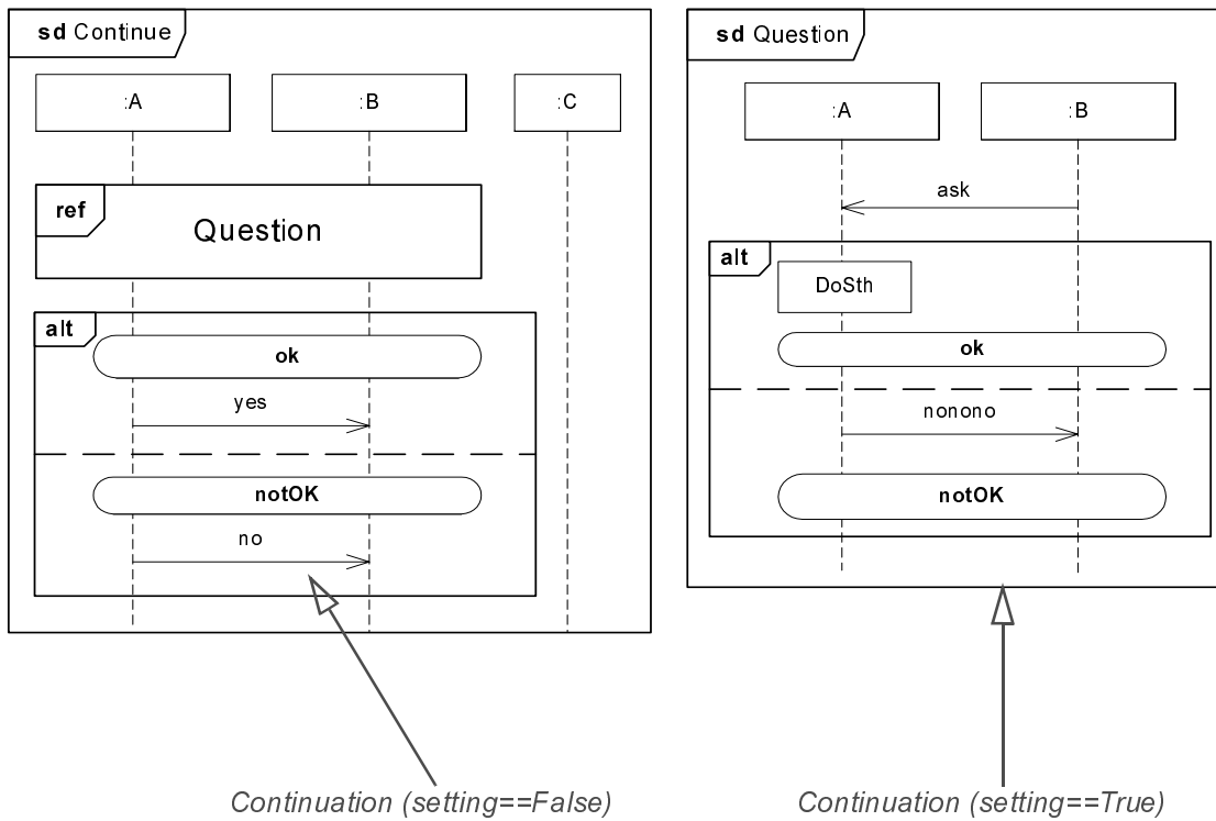
Figure 336 - Continuation
