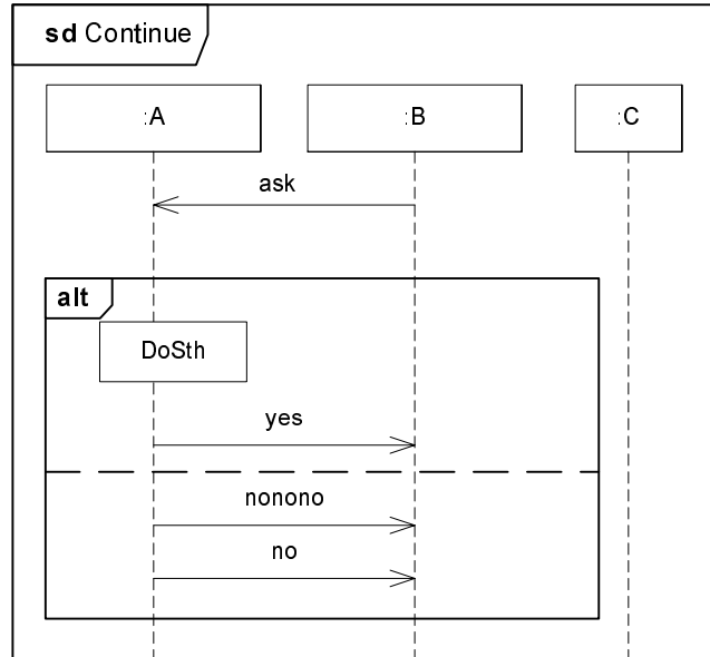
Figure 337 - Continuation interpretation
