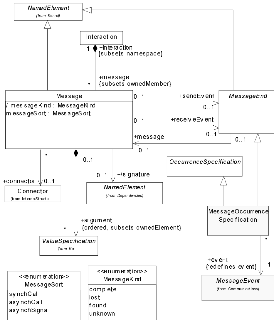
Figure 329 - Messages
