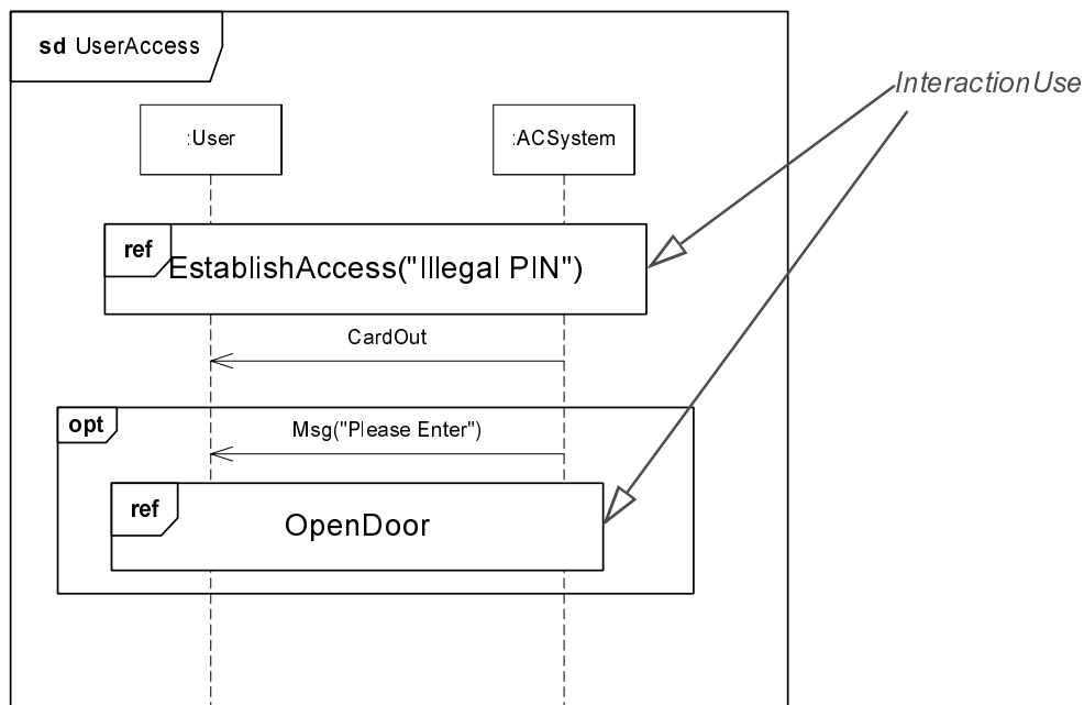
Figure 341 - InteractionUse
