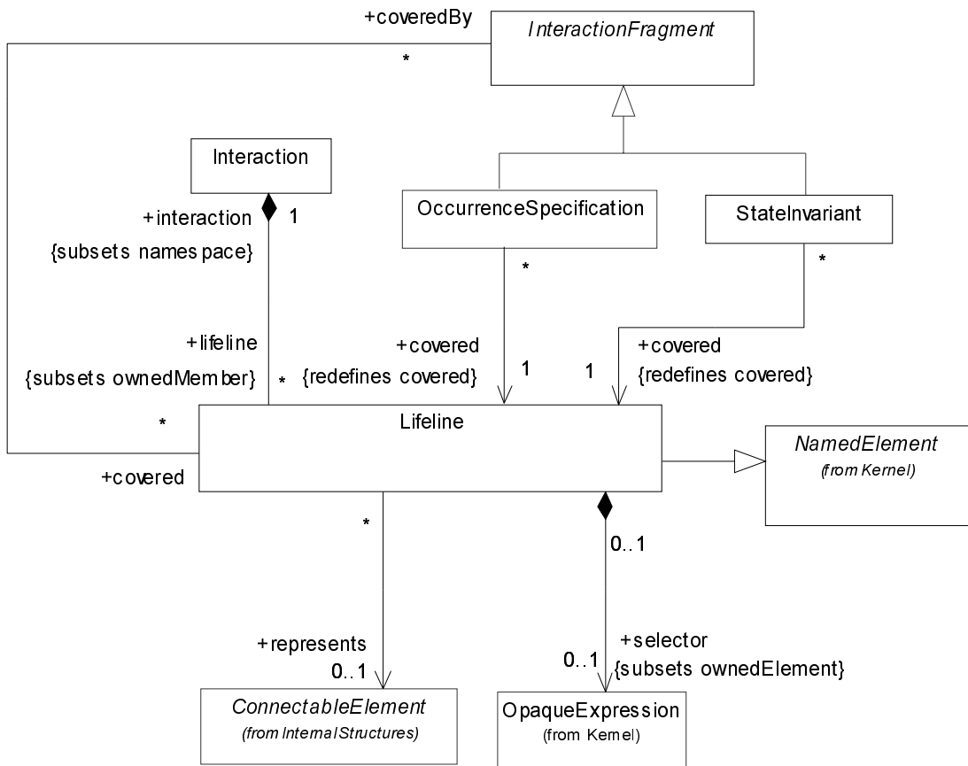
Figure 328 - Lifelines
