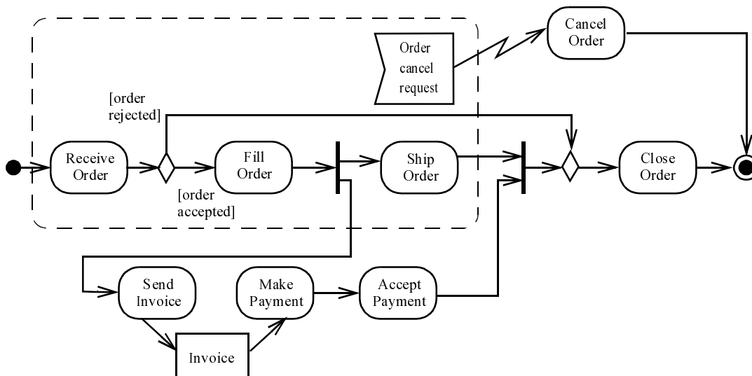
Figure 274 - InterruptibleActivityRegion example
