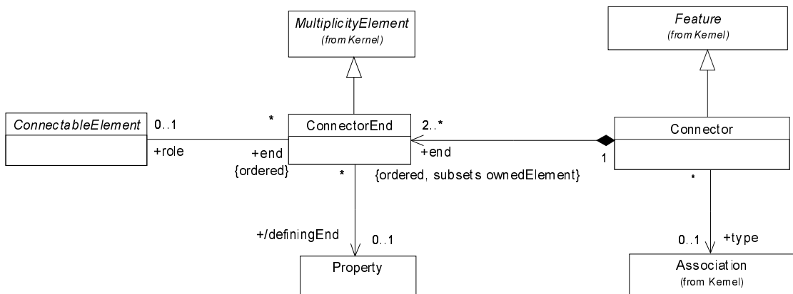
Figure 96 - Connectors
