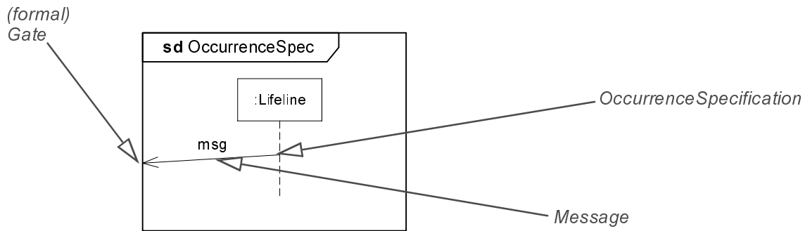
Figure 343 - OccurrenceSpecification
