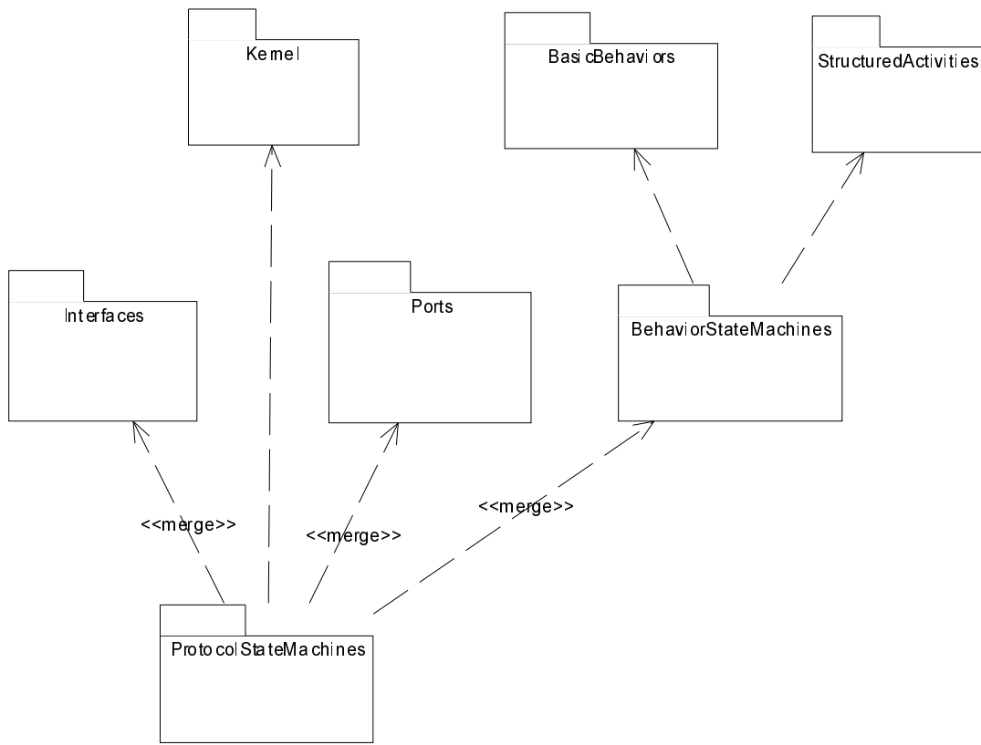
Figure 353 - Package Dependencies
