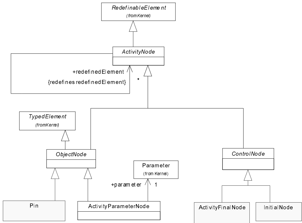
Figure 178 - Nodes (BasicActivities)
