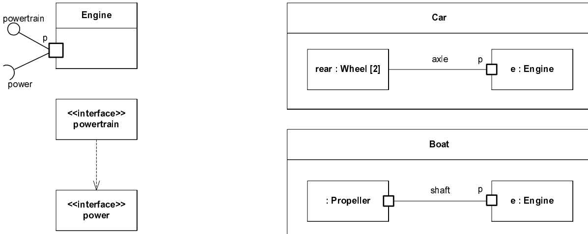
Figure 113 - Port examples
