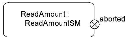
Figure 360 - Exit Point
