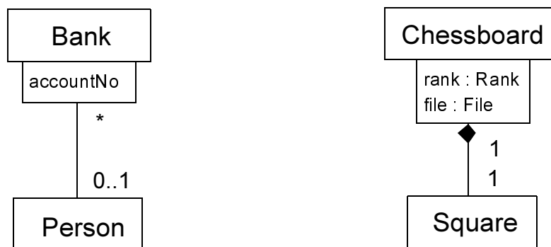
Figure 70 - Qualified associations
