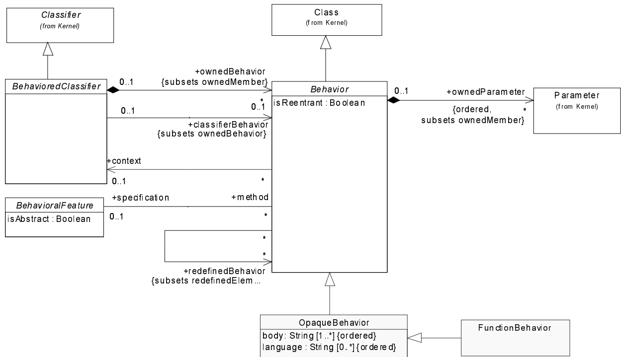
Figure 311 - Common Behavior
