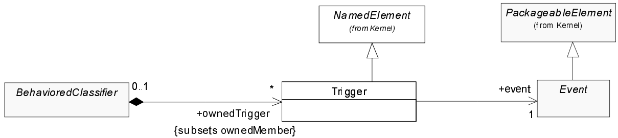
Figure 316 - Triggers
