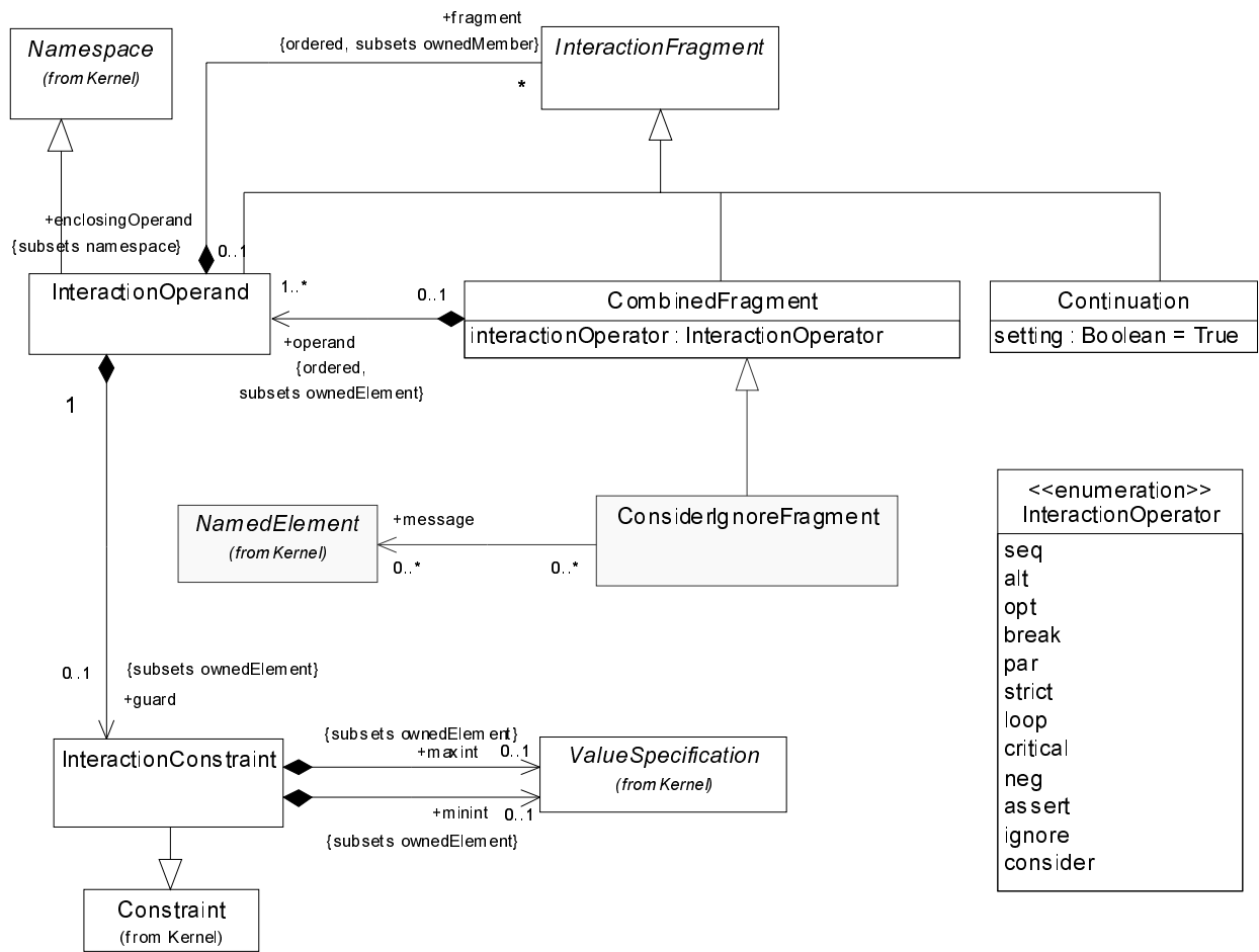
Figure 331 - CombinedFragments
