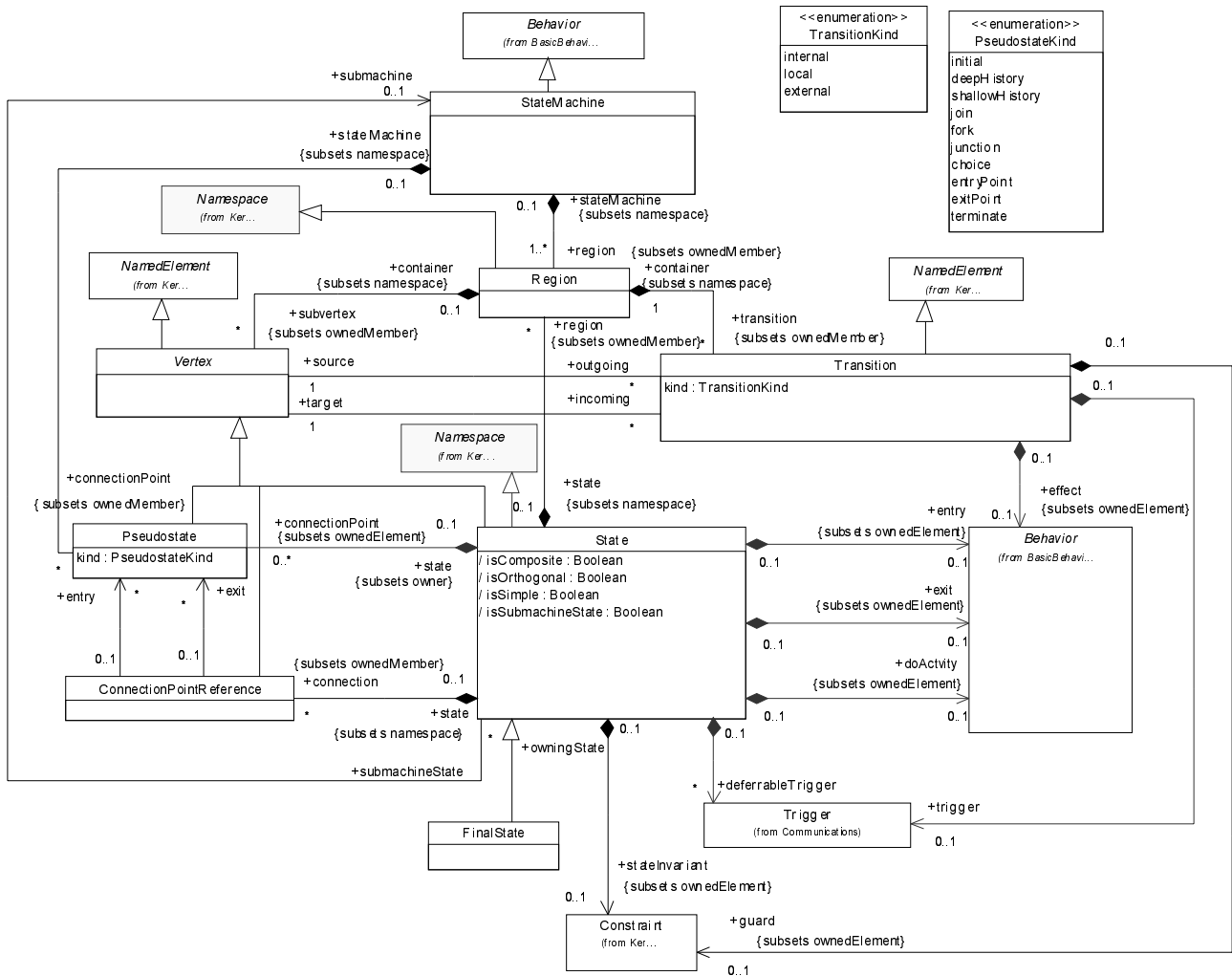
Figure 354 - State Machines
