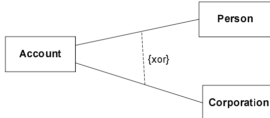
Figure 32 - {xor} constraint
