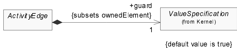
Figure 185 - Flows (IntermediateActivities)
