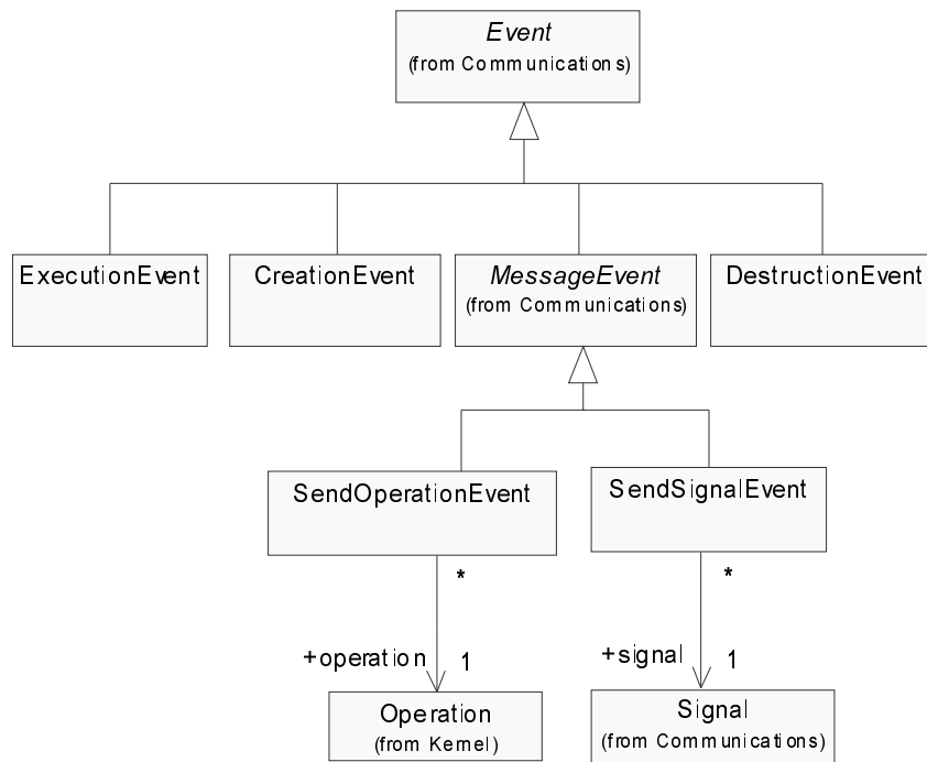
Figure 326 Events
