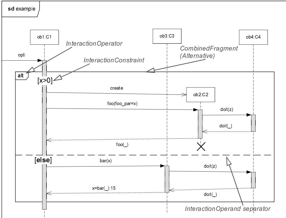
Figure 335 - CombinedFragment
