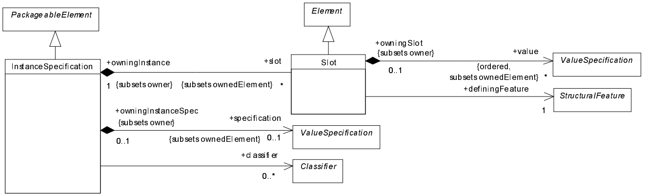
Figure 8 - The Instances diagram of the Kernel package.
