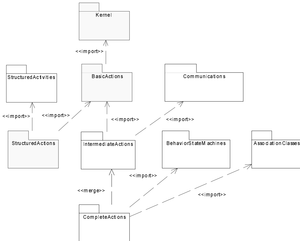
Figure 141 Dependencies of the Action packages
