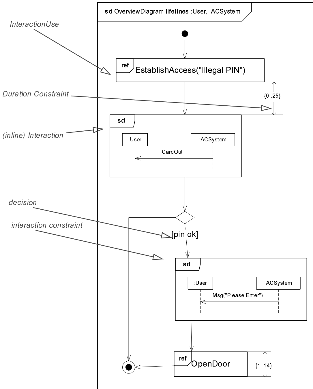
Figure 352 Interaction Overview Diagram representing a High Level Interaction diagram
