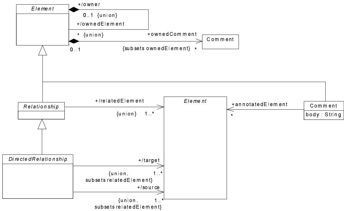
Figure 3 - The Root diagram of the Kernel package
