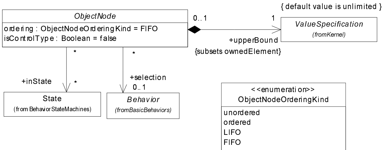
Figure 189 - Object nodes (CompleteActivities)
