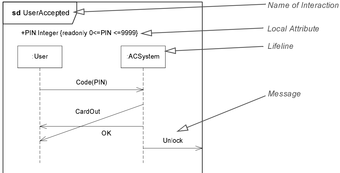
Figure 340 - An example of an Interaction in the form of a Sequence Diagram
