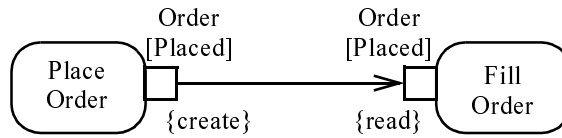
Figure 305 Pin example with effects
