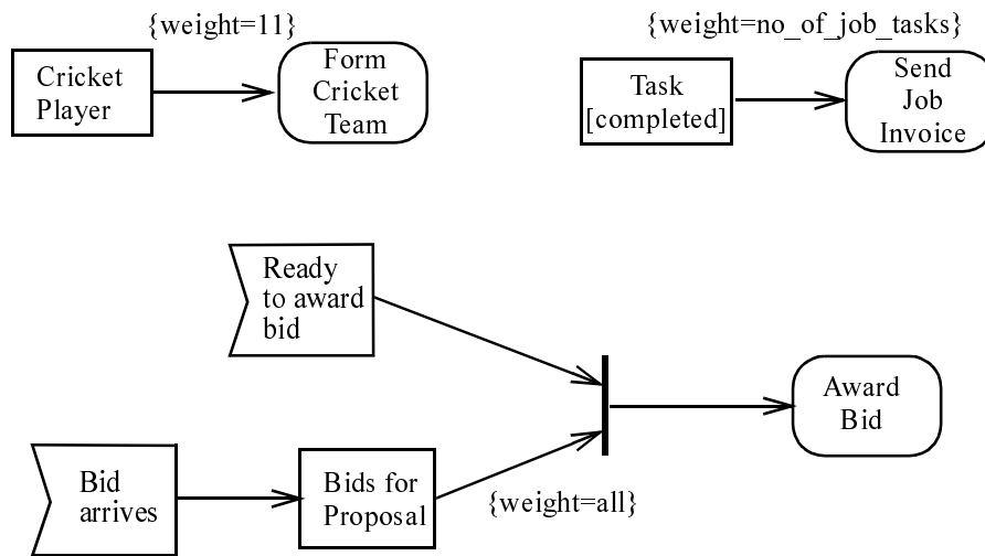
Figure 219 - Activity edge examples
