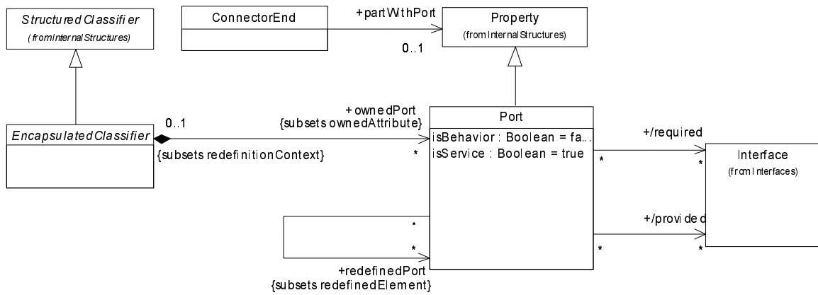
Figure 97 - The Port metaclass
