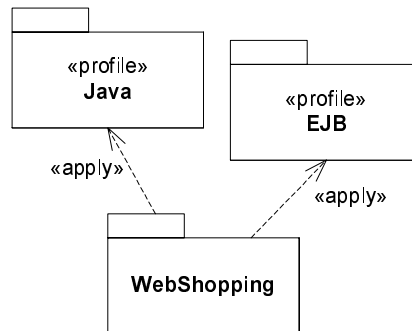
Figure 455 - Profiles applied to a package
