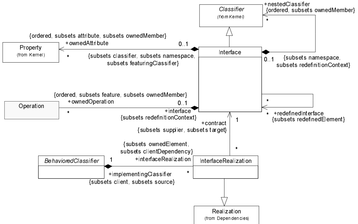
Figure 16 - The contents of Interfaces package
