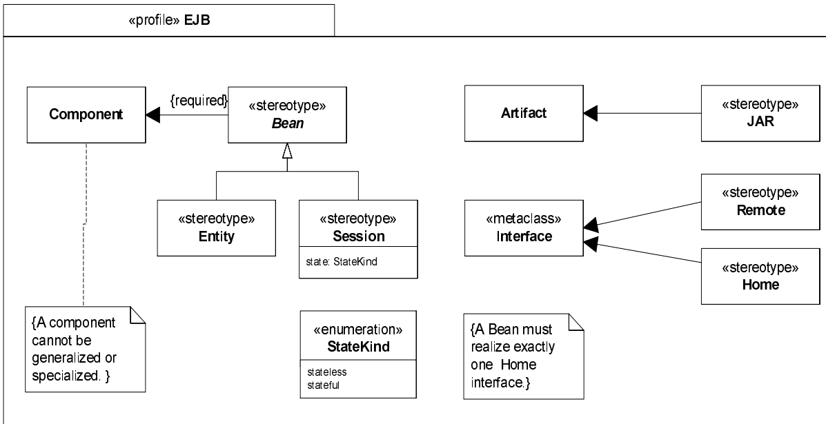
Figure 453 - Defining a simple EJB profile
