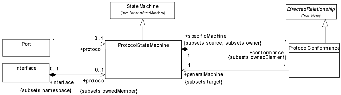
Figure 357 - Protocol state machines
