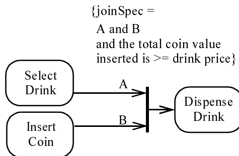
Figure 278 - Join node example
