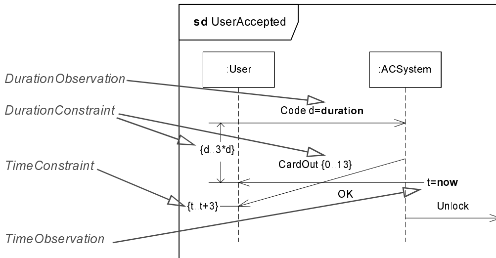
Figure 350 - Sequence Diagram with time and timing concepts
