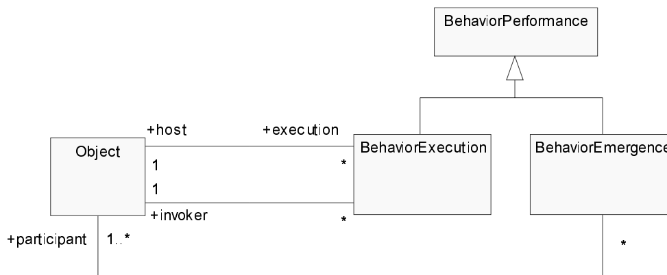
Figure 306 - Common Behaviors Domain Model
