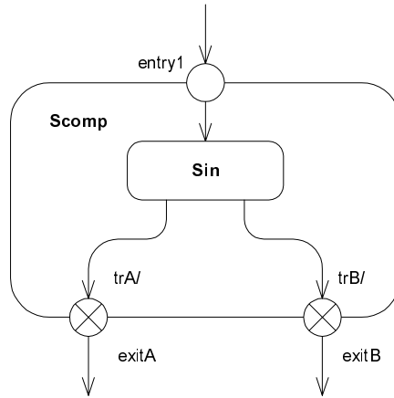
Figure 373 - Entry and exit points on composite states
