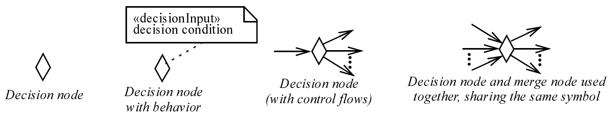
Figure 250 - Decision node notation
