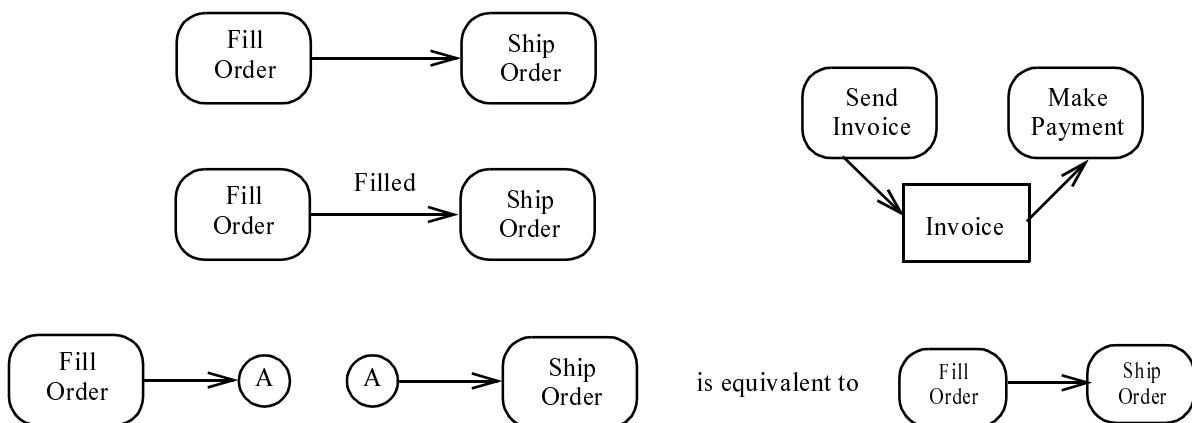
Figure 216 - Activity edge examples
