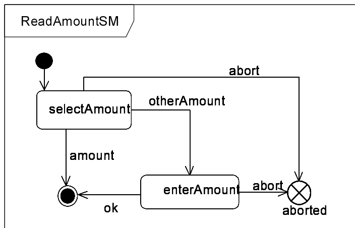
Figure 389 - State machine with exit point as part of the state graph
