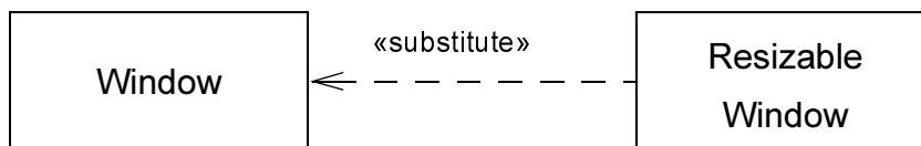
Figure 72 - An example of a substitute dependency
