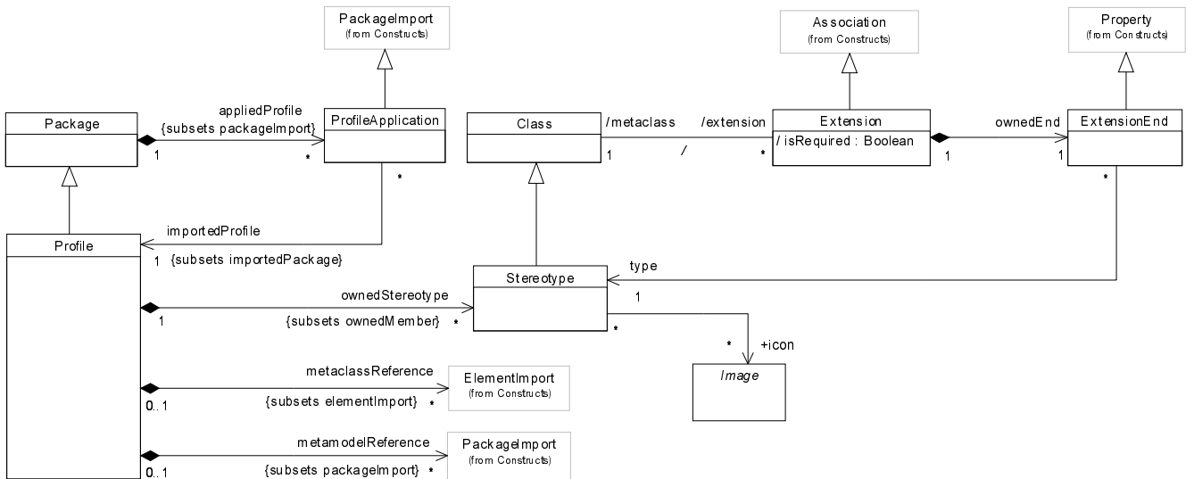
Figure 446 - The elements defined in the Profiles package
