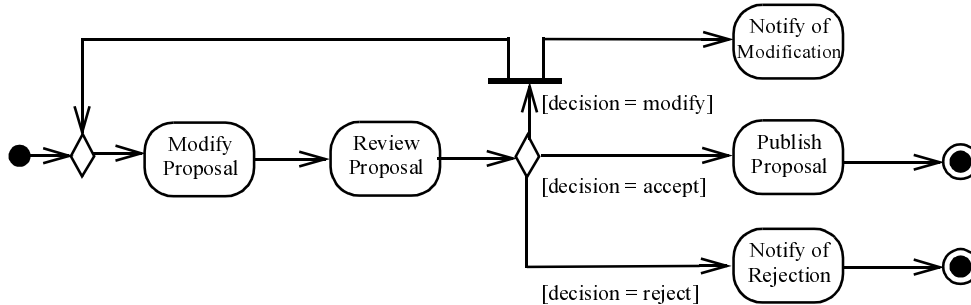
Figure 223 - Activity final example
