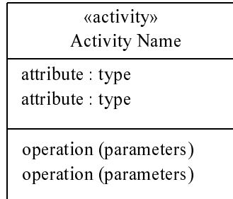
Figure 208 - Activity class notation
