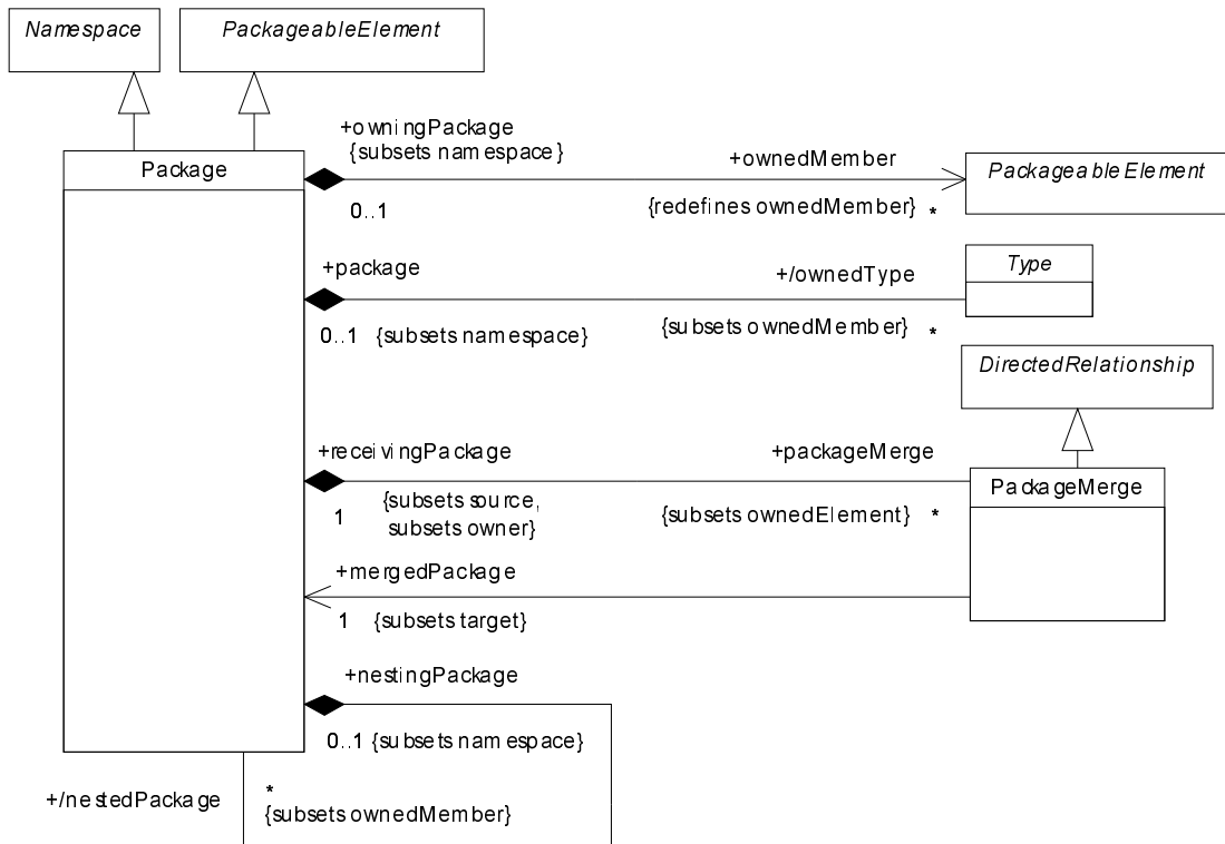
Figure 14 - The Packages diagram of the Kernel package
