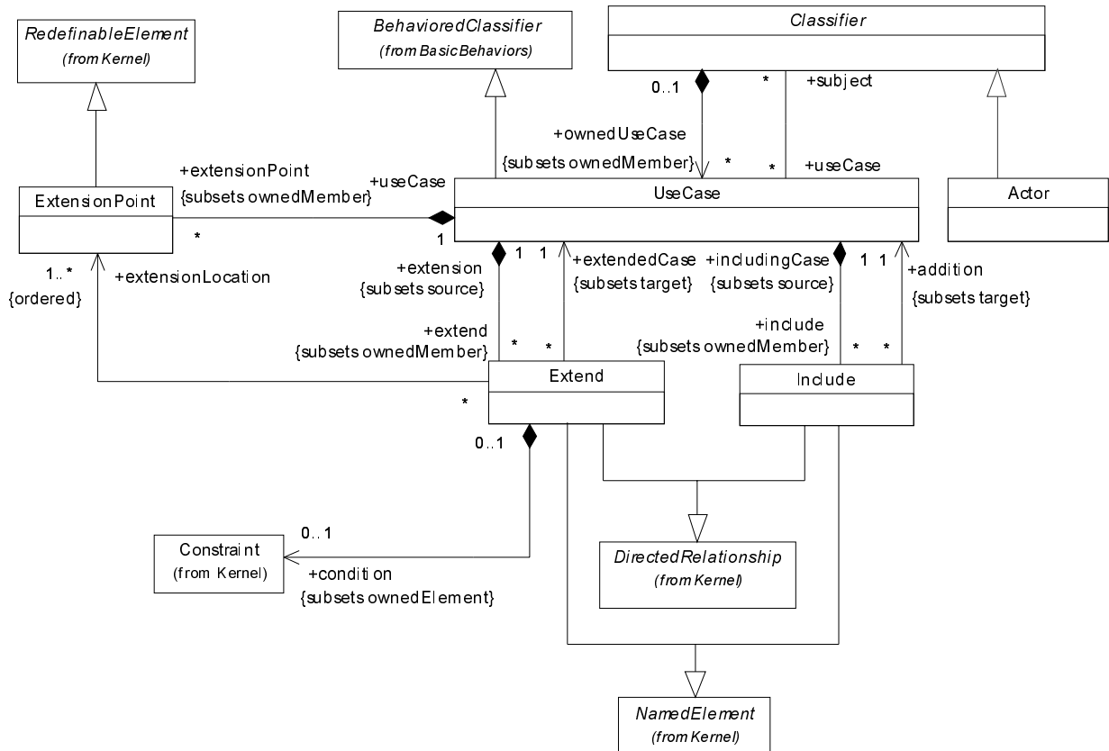
Figure 401 - The concepts used for modeling use cases
