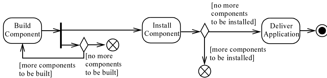
Figure 265 - Flow final and activity final example.
