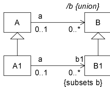
Figure 23 - Derived supersets (union)
