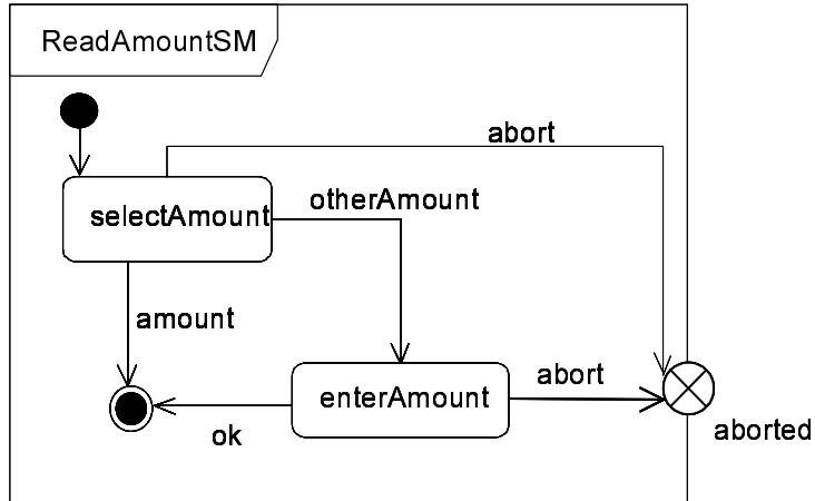
Figure 399 - State machine with exit point definition
