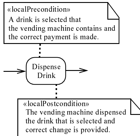
Figure 206 - Example of an action with local pre/postconditions.
