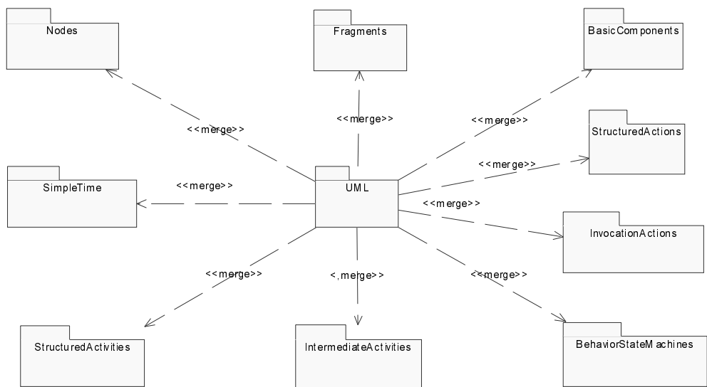
Figure 3 - Level 2 top-level package merges
