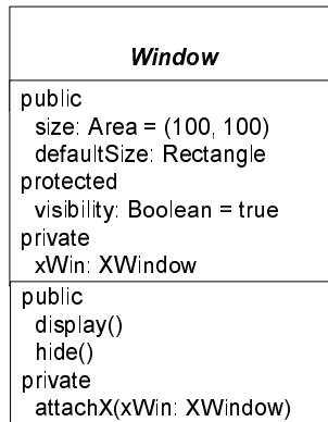
Figure 27 - Class notation: attributes and operations grouped according to visibility
