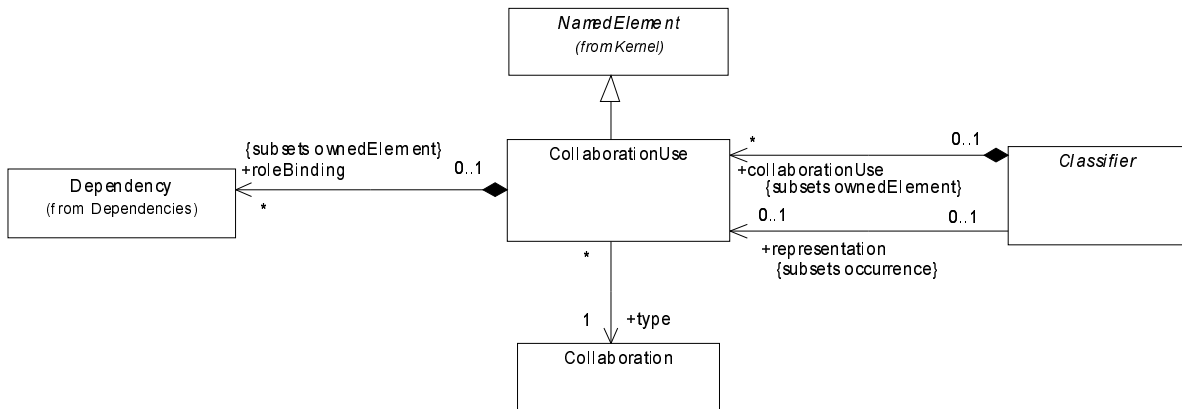
Figure 100 - Collaboration.use and role binding
