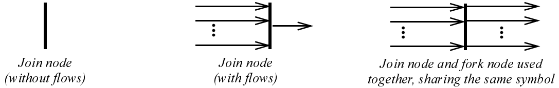
Figure 275 - Join node notations
