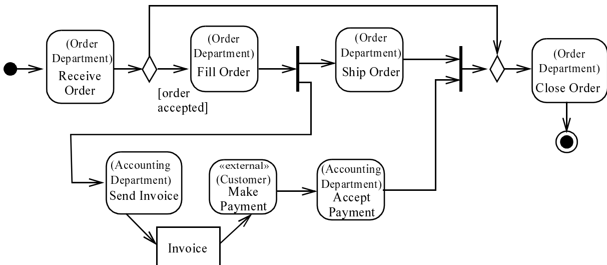
Figure 234 - Activity partition using annotation example
