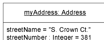
Figure 51 - Slots with values
