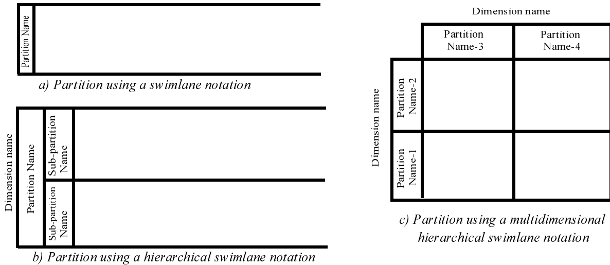
Figure 231 - Activity partition notations
