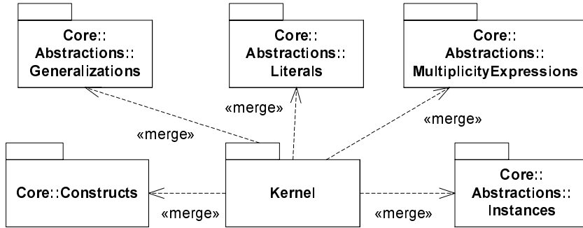
Figure 8 - The InfrastructureLibrary packages that are merged by Kernel; all dependencies in the picture represent package merges
