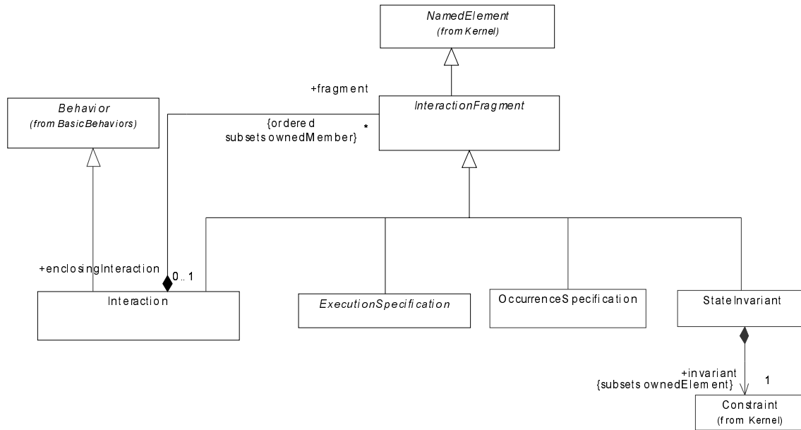
Figure 327 - Interactions
