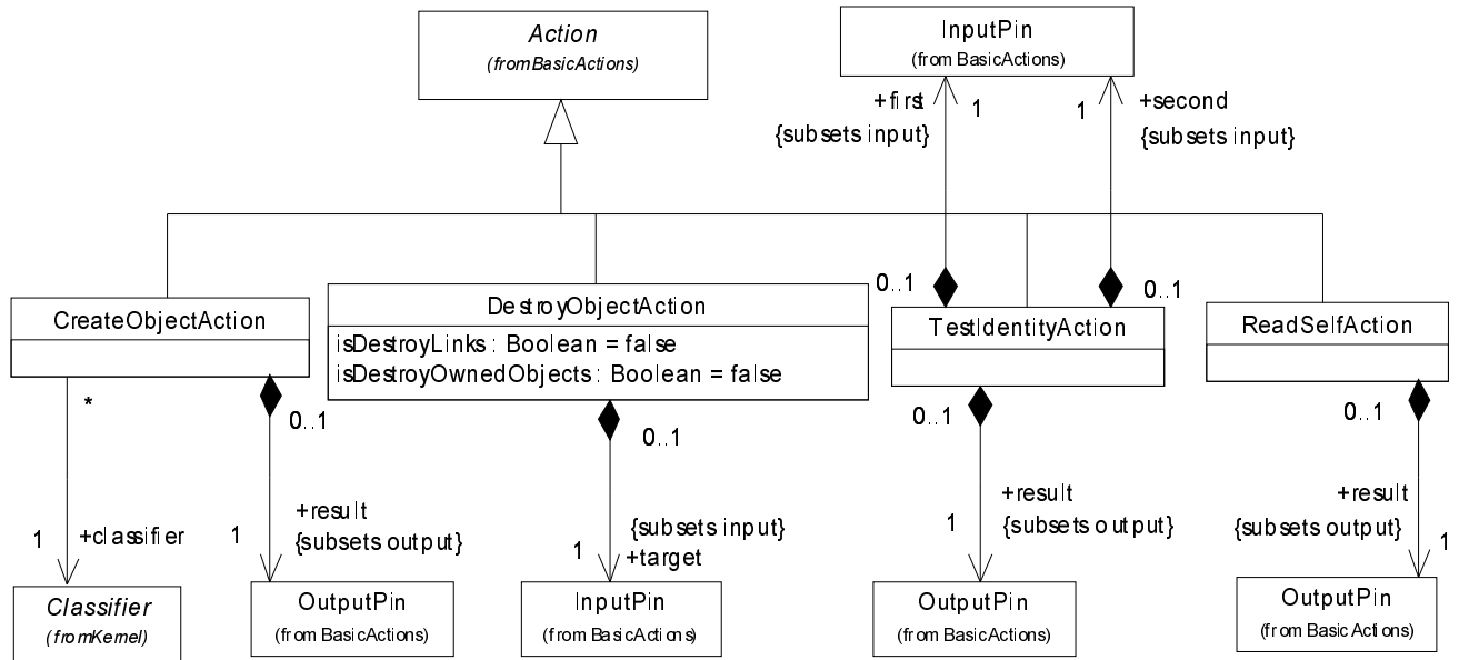
Figure 146 - Object actions
