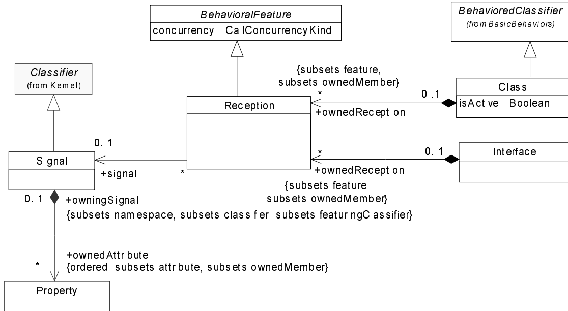
Figure 314 - Reception
