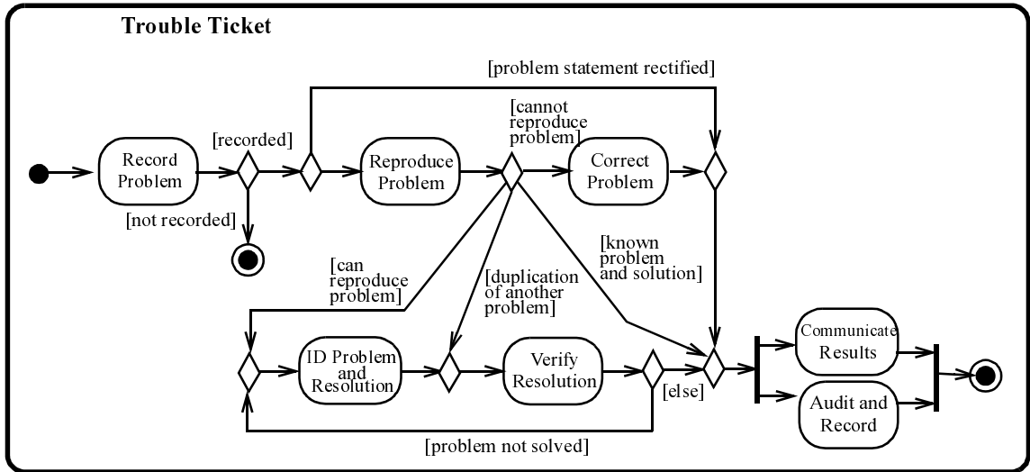
Figure 211 - Workflow example
