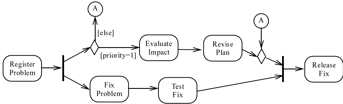
Figure 217 - Connector example
