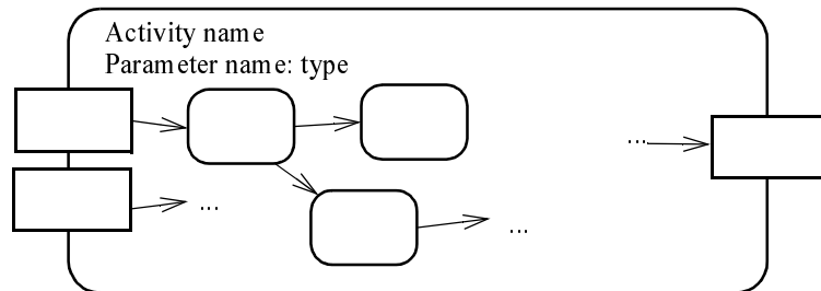
Figure 226 - Activity notation
