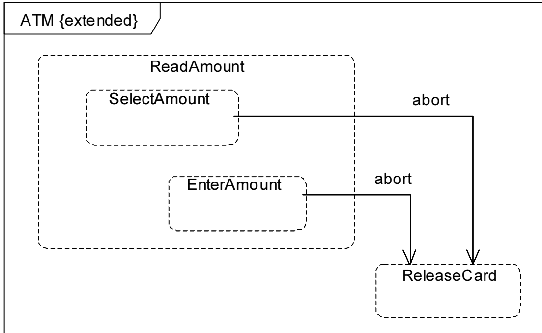
Figure 398 - Adding Transitions
