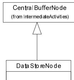
Figure 191 - Data stores
