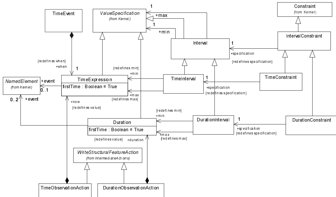
Figure 318 - SimpleTime
