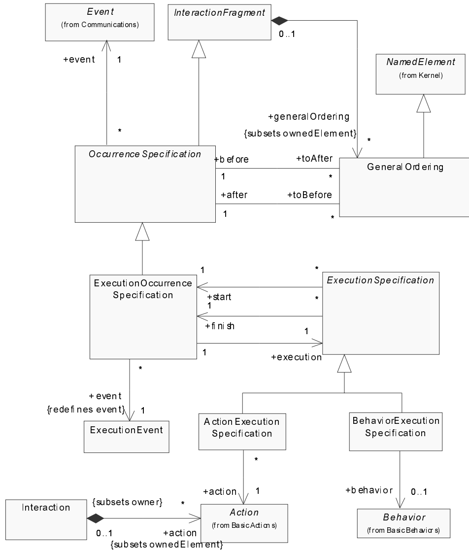
Figure 330 Occurrences
