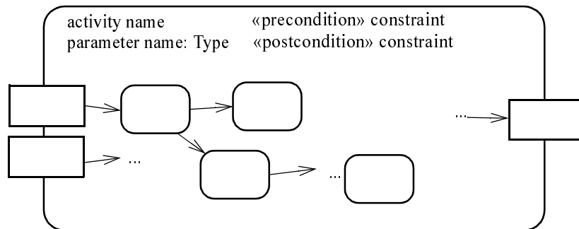
Figure 207 - Activity notation
