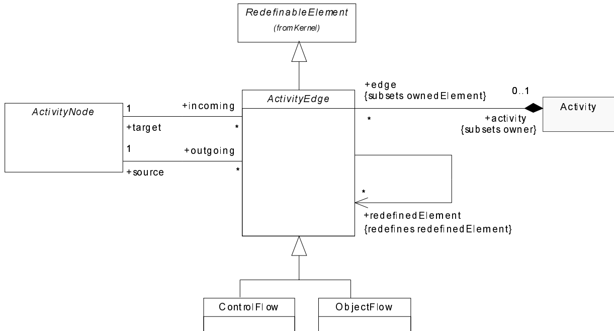
Figure 179 - Flows
