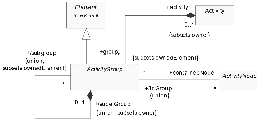
Figure 177 - Fundamental groups
