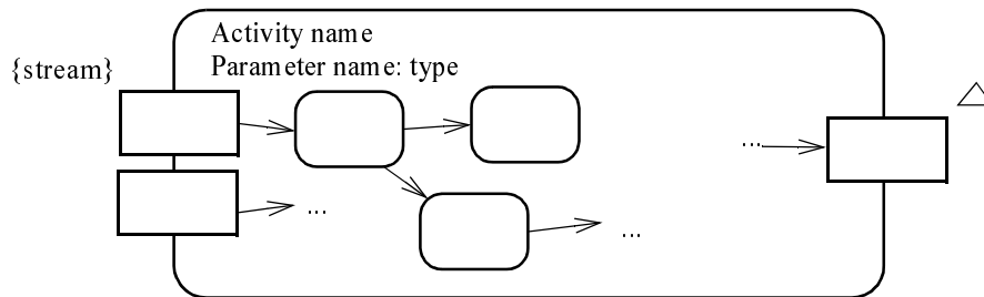
Figure 227 - Activity notation
