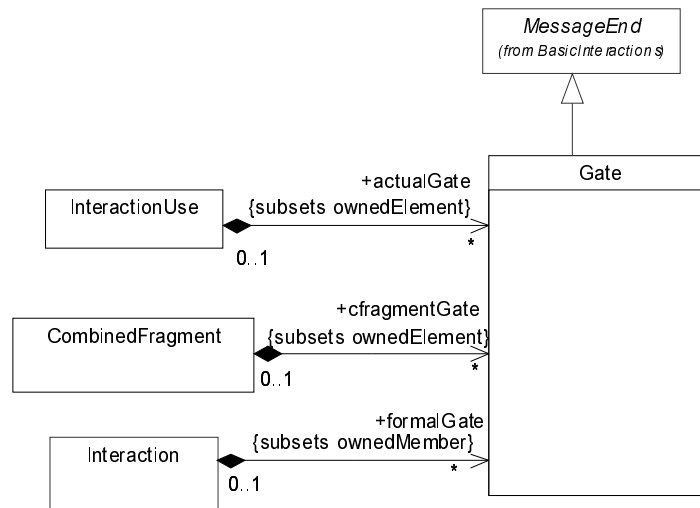
Figure 332 - Gates
