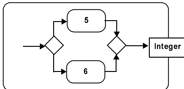
Figure 309 - Example ValueSpecificationAction
