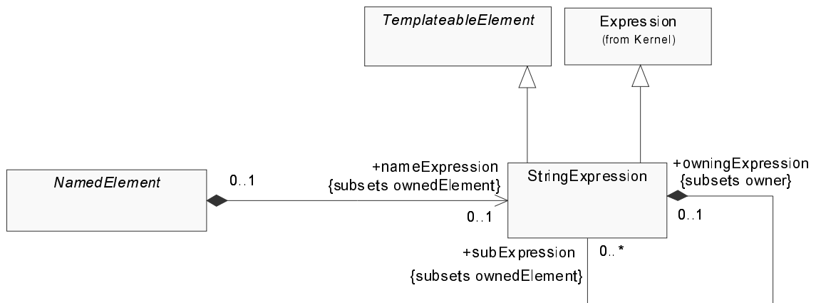
Figure 438 - Name expression
