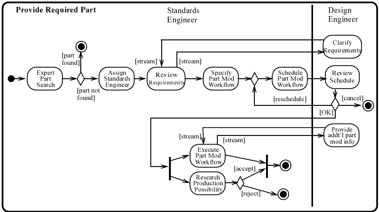
Figure 210 - Workflow example
