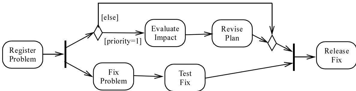
Figure 218 - Equivalent model to Figure 217
