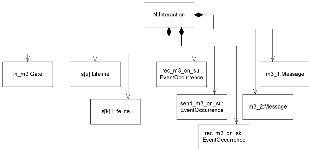
Figure 347 - Metamodel elements of a sequence diagram
