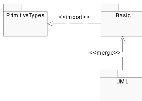
Figure 1 - Level 0 package diagram
