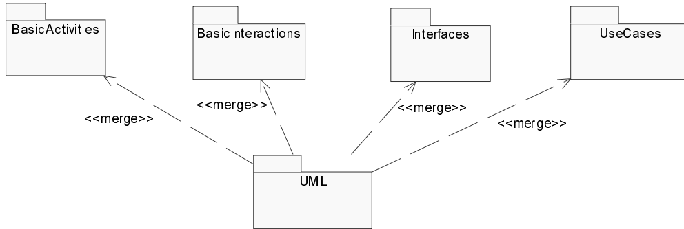
Figure 2 - Level 1 top-level package merges
