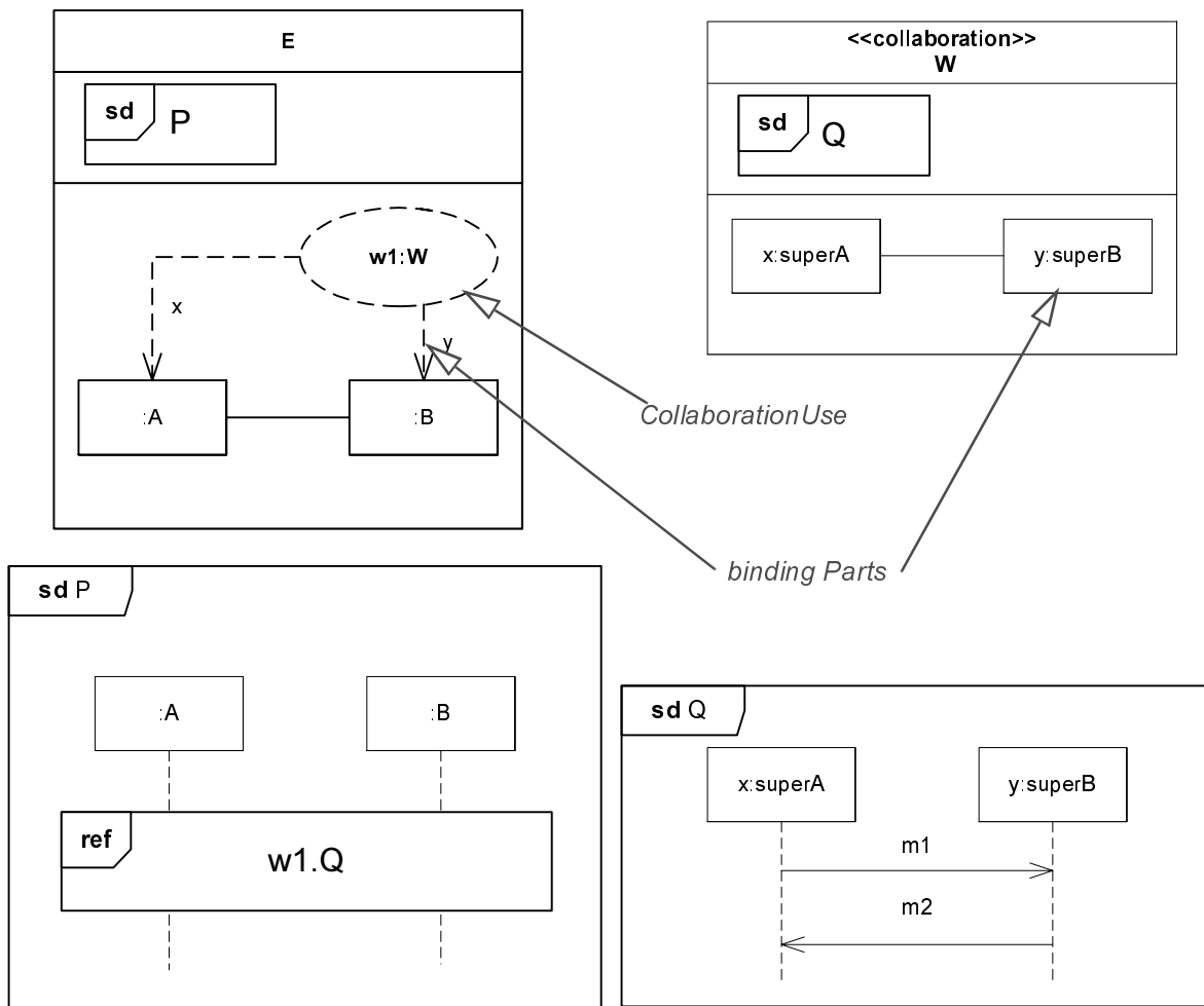
Figure 349 - Describing collaborations and their binding
