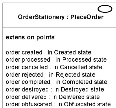
Figure 408 - Example of the classifier based notation for a use case
