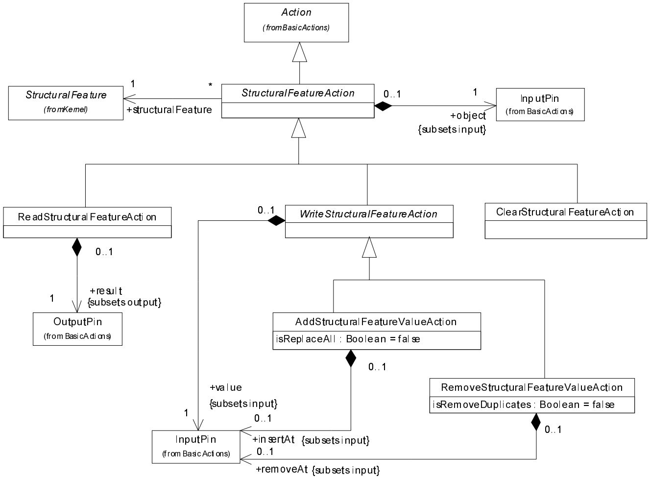
Figure 147 - Structural Feature Actions
