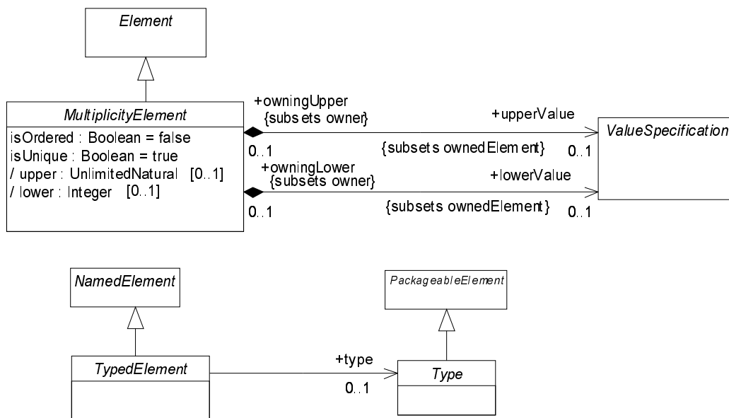
Figure 5 - The Multiplicities diagram of the Kernel package.
