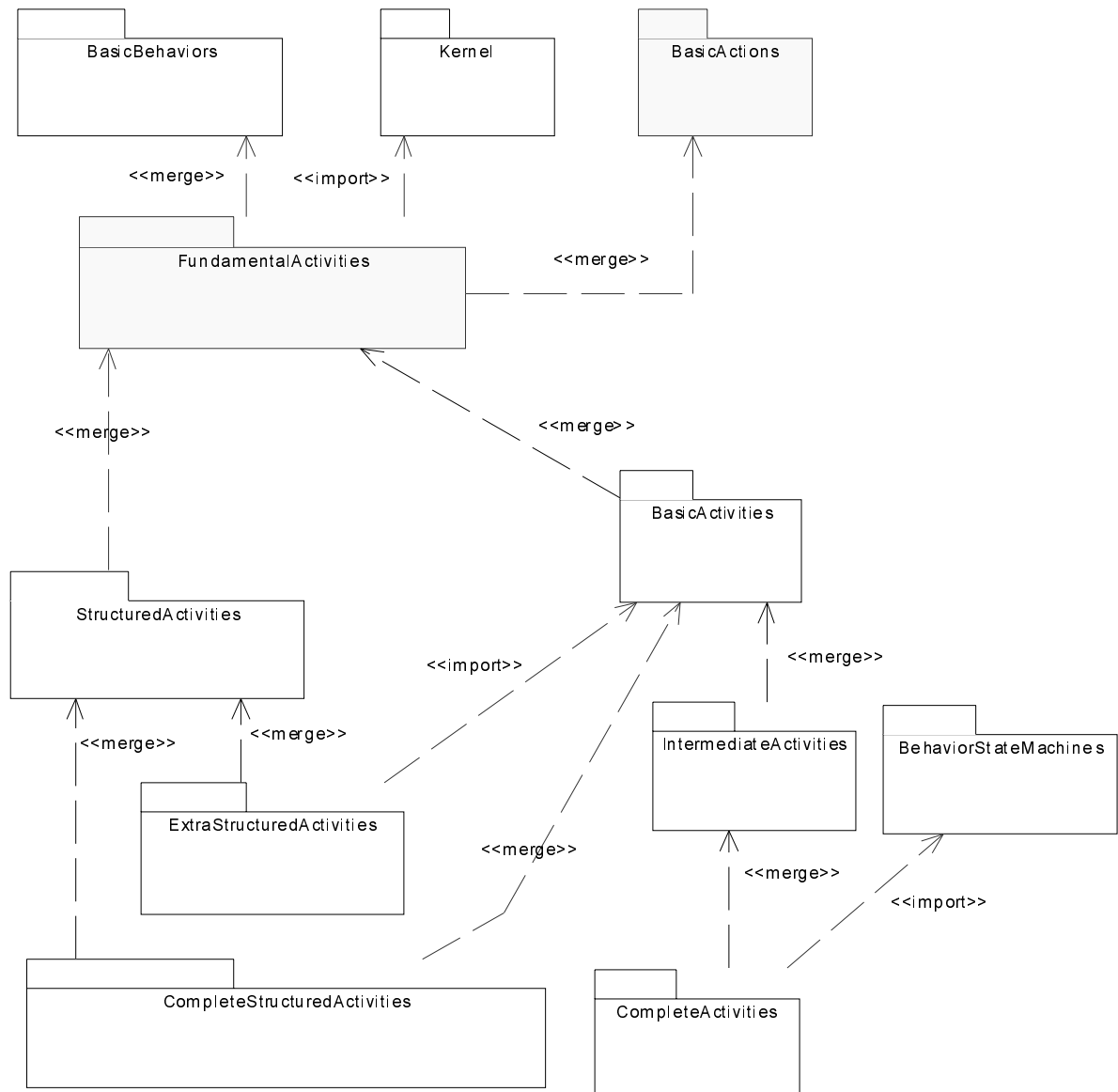
Figure 175 - Dependencies of the Activity packages
