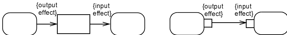
Figure 297 - Specifying effect that actions have on objects
