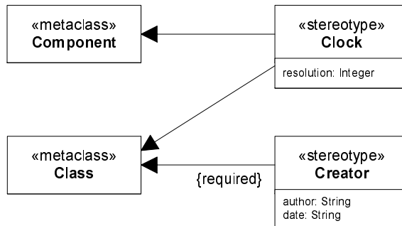
Figure 459 - Defining multiple stereotypes on multiple stereotypes
