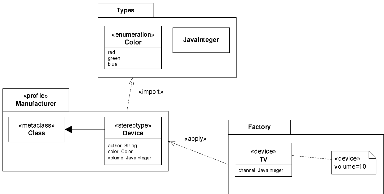
Figure 454 - Importing a package from a profile
