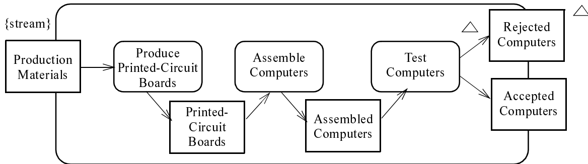
Figure 230 - Example of activity parameter nodes for streaming and exceptions
