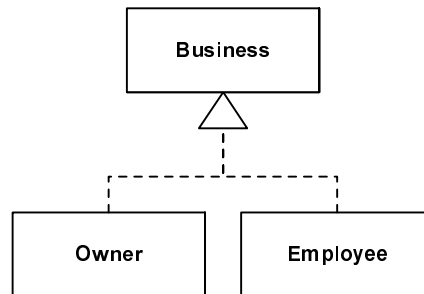
Figure 71 - An example of a realization dependency
