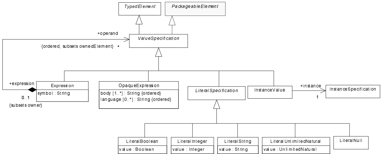
Figure 6 - The Expressions diagram of the Kernel package.
