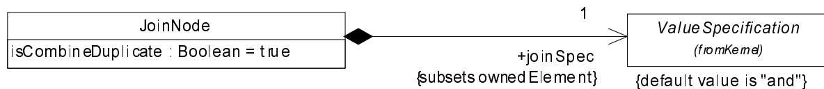
Figure 193 - Control nodes (CompleteActivities)
