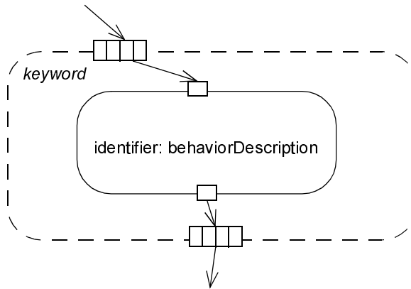
Figure 258 - Full form of previous shorthand notation
