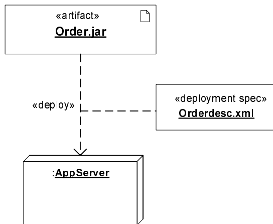
Figure 135 - A DeploymentSpecification for an artifact
