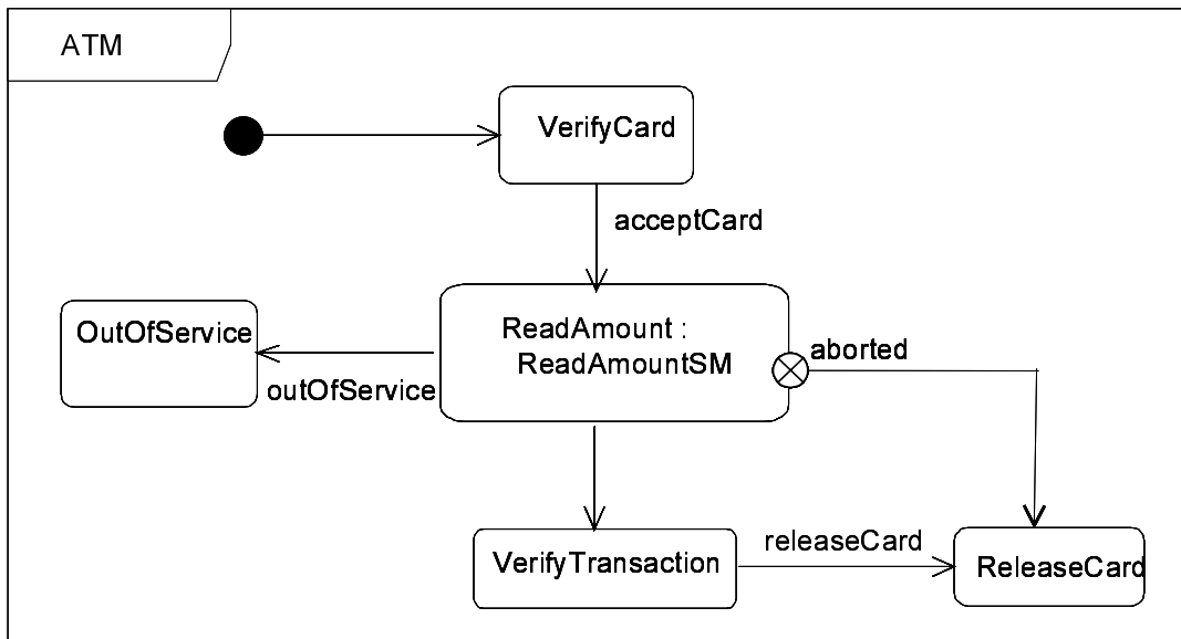
Figure 400 - SubmachineState with usage of exit point
