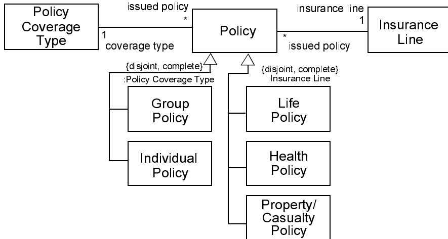
Figure 49 - Other power type examples
