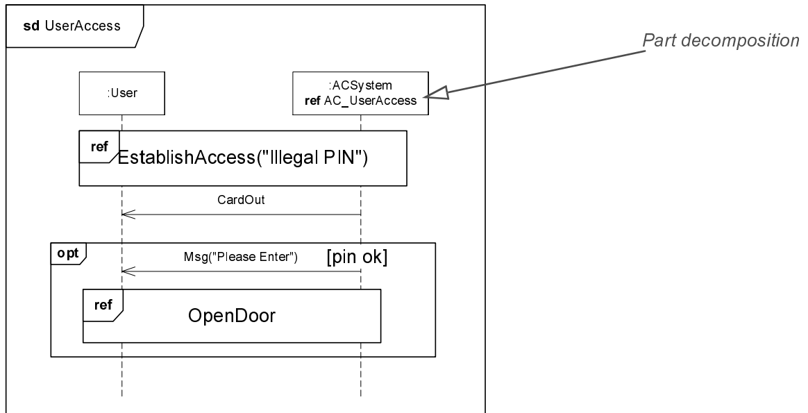
Figure 344 - Part Decomposition - the decomposed part
