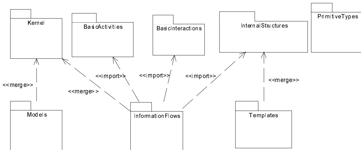
Figure 412 - Dependencies between packages described in this chapter
