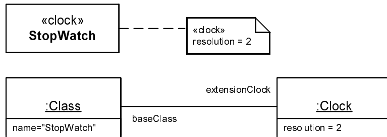
Figure 461 - Showing values of stereotypes and a simple instance specification
