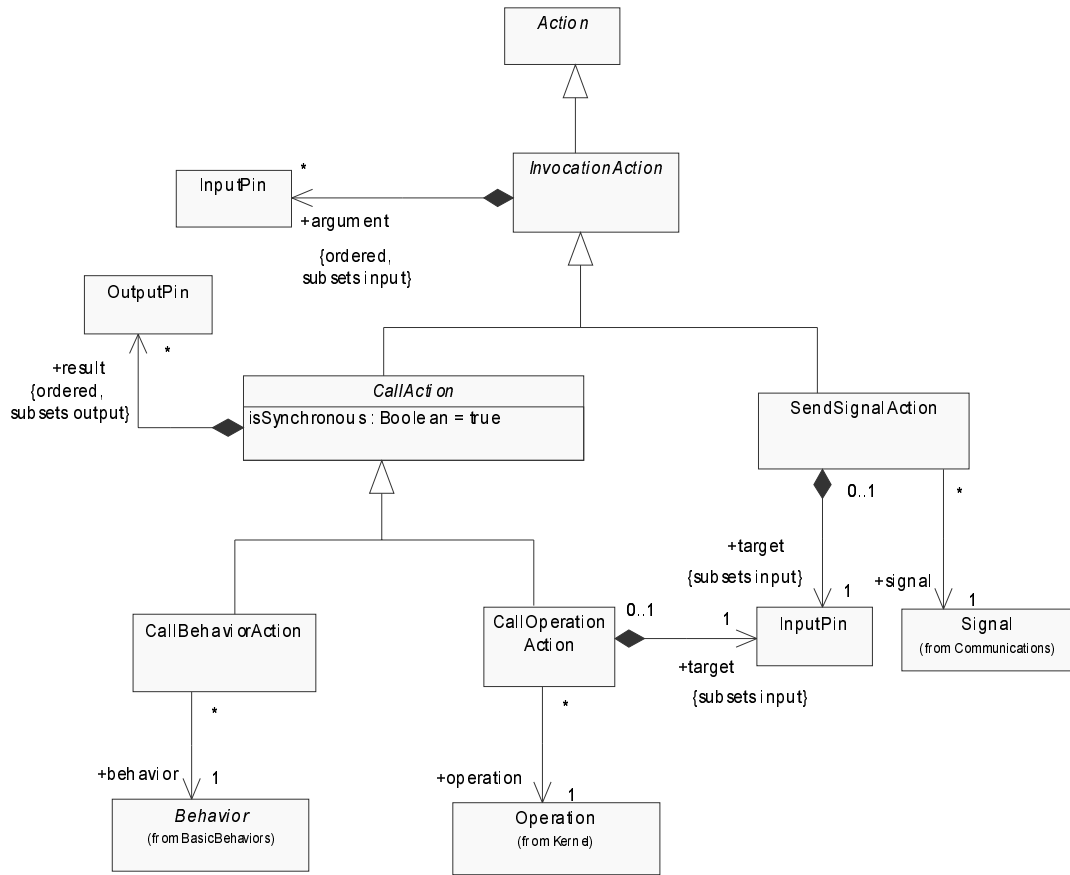
Figure 144 - Basic invocation actions
