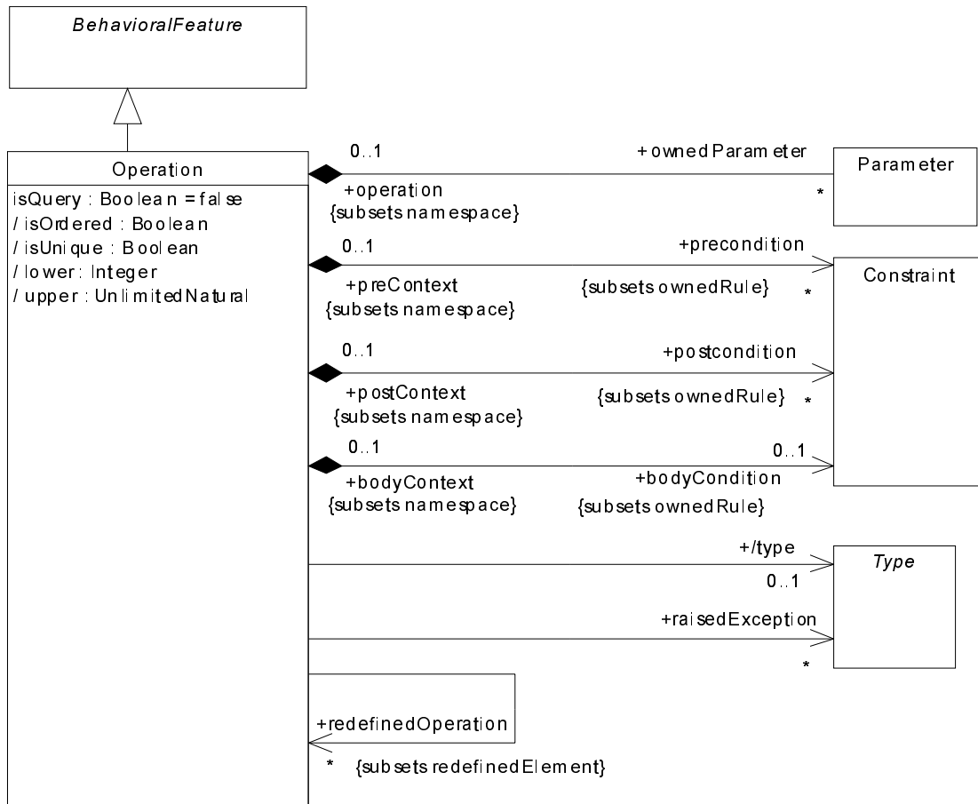
Figure 11 - The Operations diagram of the Kernel package
