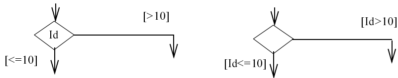
Figure 378 - Alternative Notation for Choice Pseudostate
