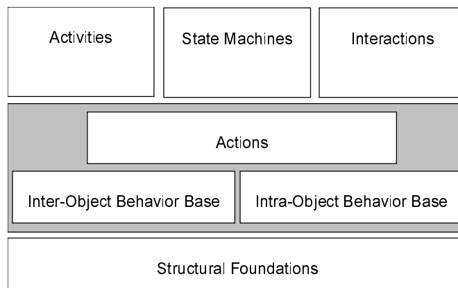
Figure 5 - A schematic of the UML semantic areas and their dependencies
