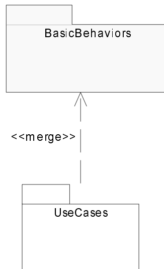
Figure 400 - Dependencies of the UseCases package
