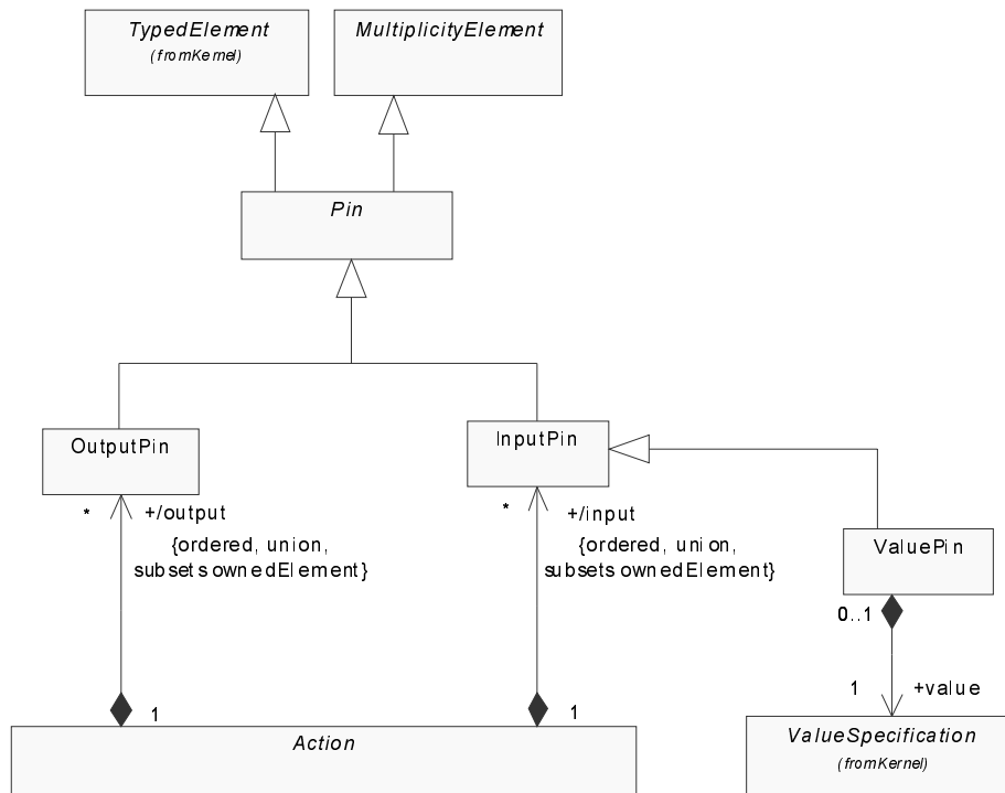
Figure 143 - Basic pins
