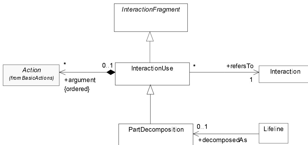
Figure 333 - InteractionUses
