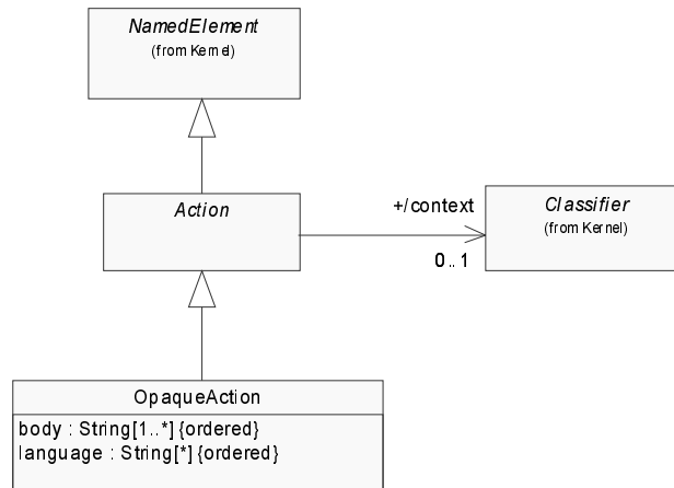
Figure 142 - Basic actions
