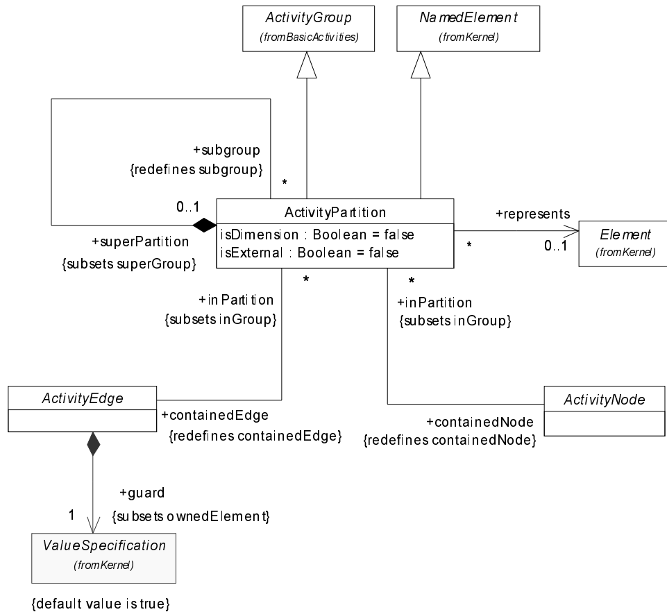
Figure 184 - Partitions
