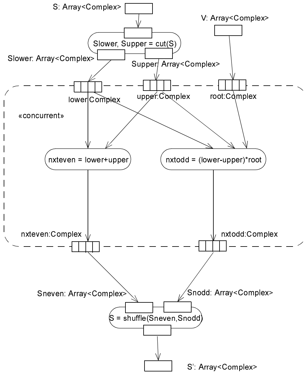
Figure 261 - Expansion region
