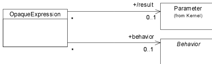
Figure 312 - Expression
