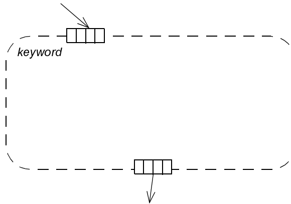
Figure 256 - Expansion region
