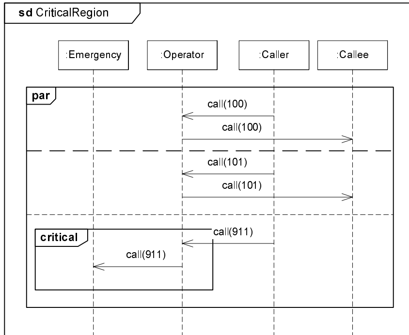
Figure 334 - Critical Region
