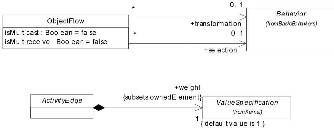
Figure 188 - Flows (CompleteActivities)
