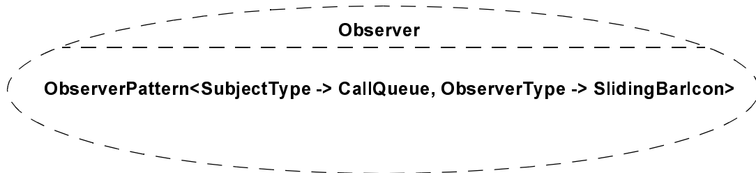
Figure 435 - Bound Collaboration
