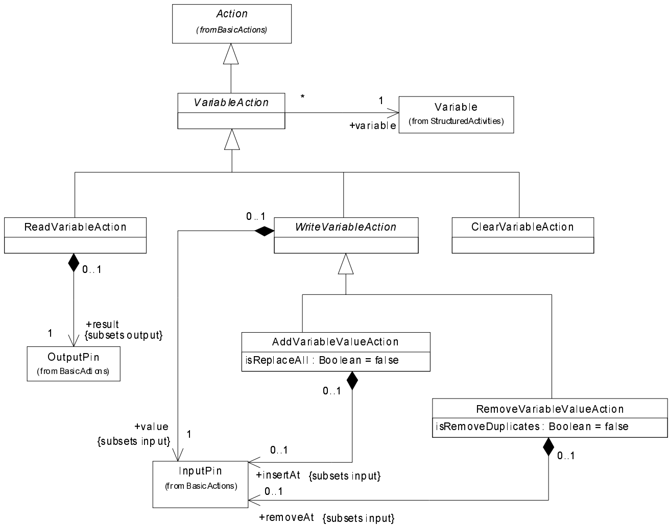
Figure 157 - Variable actions
