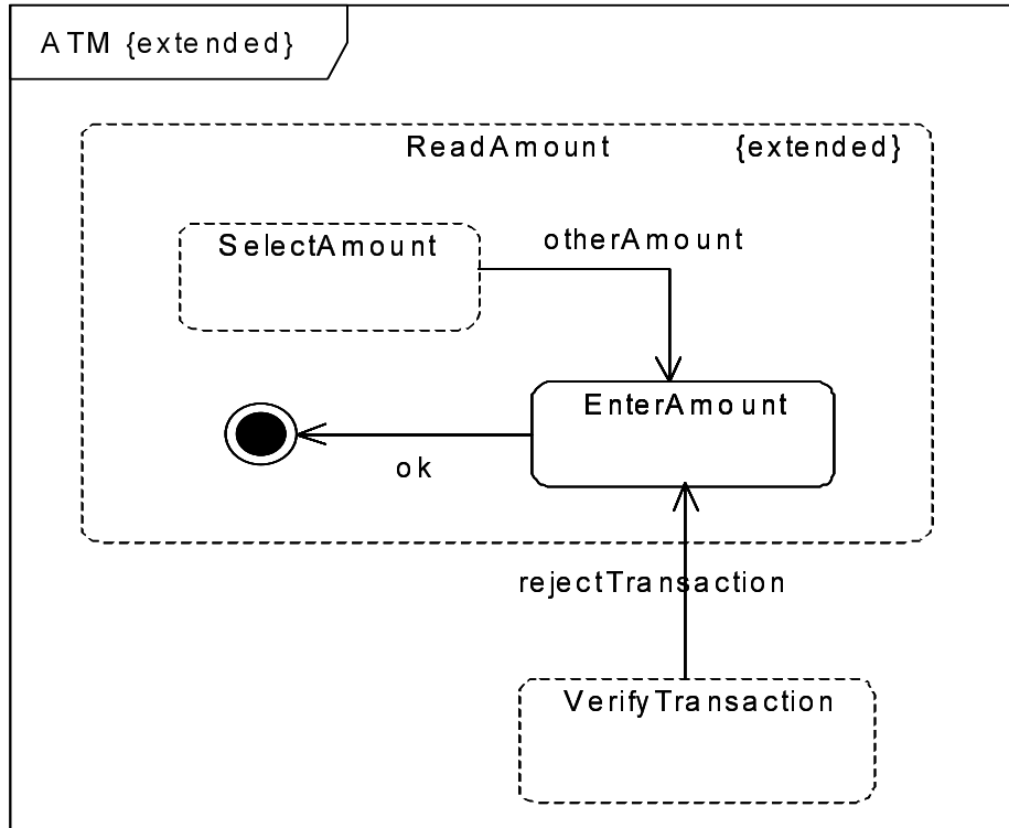
Figure 395 - An extended state machine
