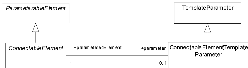
Figure 442 - Connectable element template parameters
