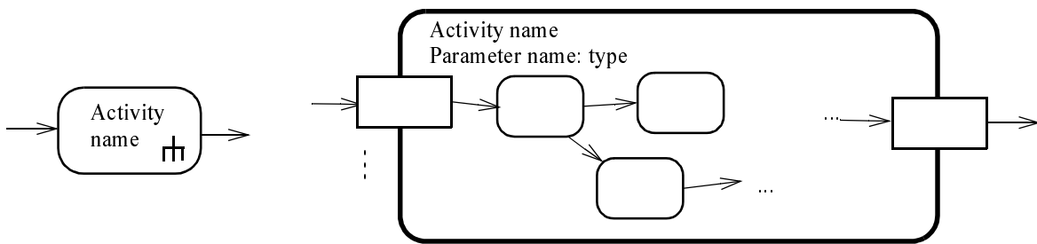
Figure 238 - Invoking Activities that have nodes and edges
