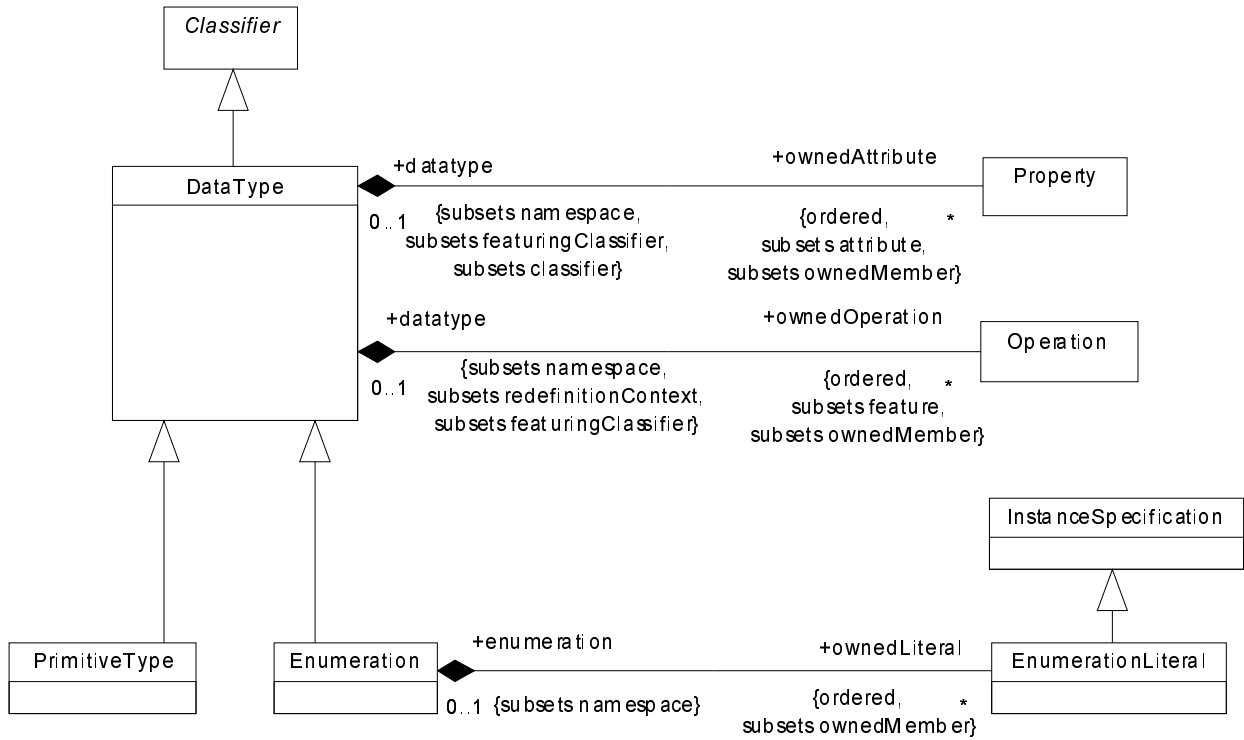
Figure 13 - The DataTypes diagram of the Kernel package
