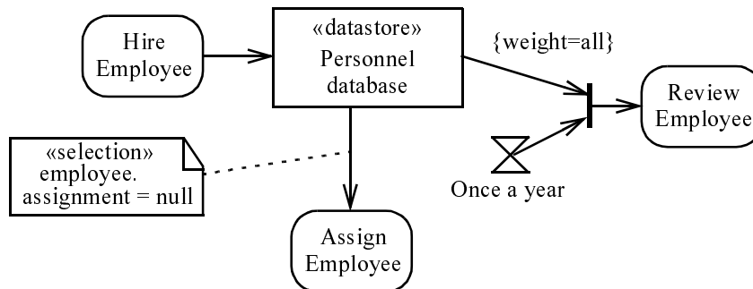
Figure 249 - Data store node example
