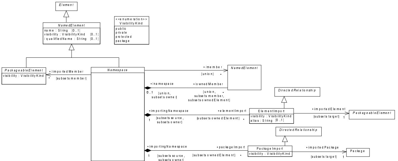
Figure 4 - The Namespaces diagram of the Kernel package
