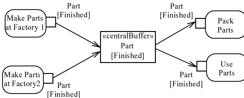
Figure 243 - Central buffer node example
