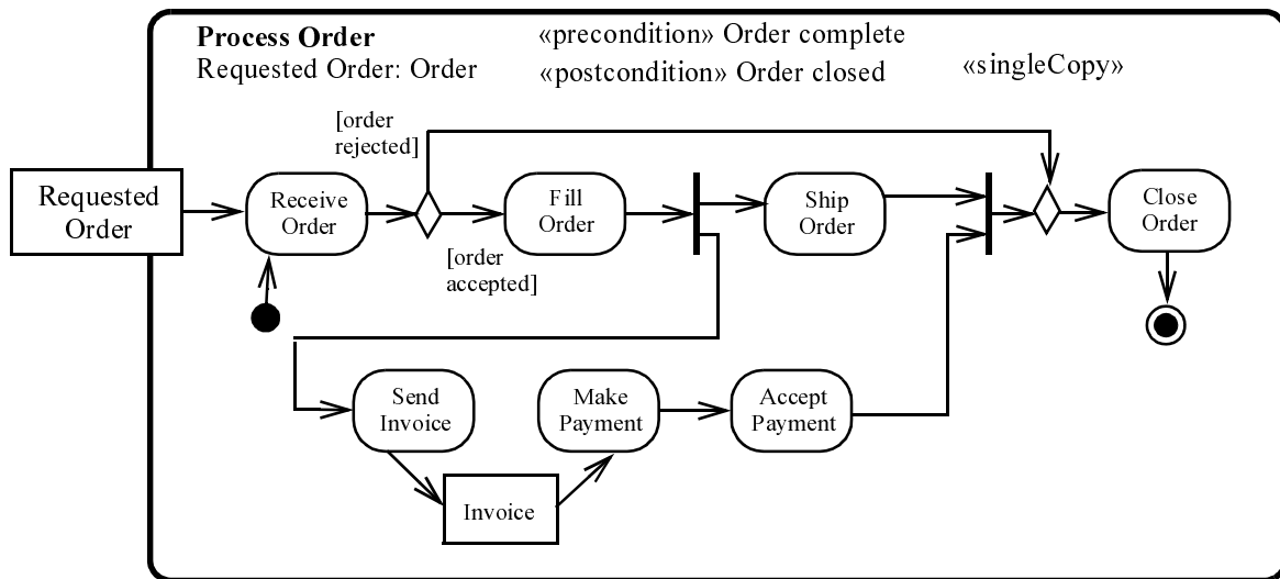
Figure 209 - Example of an activity with input parameter
