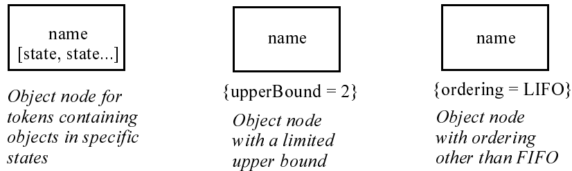
Figure 289 - Object node notations
