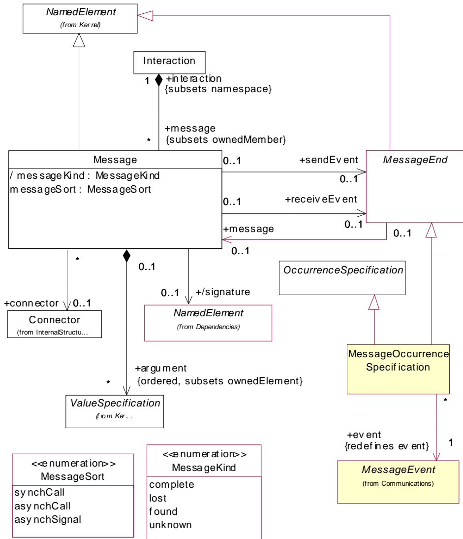
Figure 14.5 - Messages
