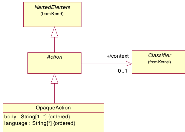
Figure 11.2 - Basic actions
