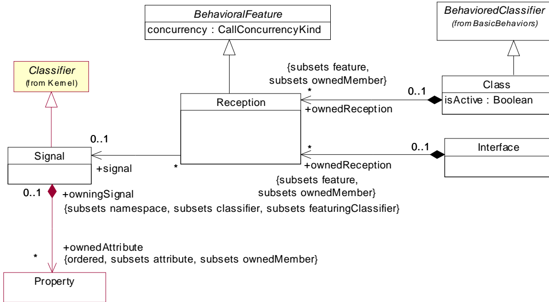
Figure 13.9 - Reception
