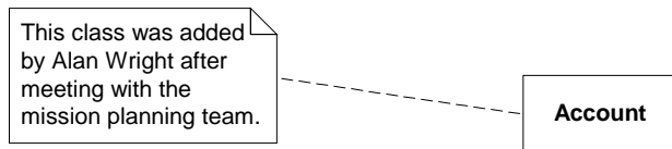
Figure 7.30 - Comment notation
