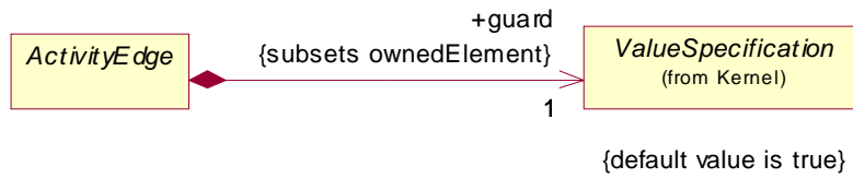
Figure 12.11 - Flows (IntermediateActivities)
