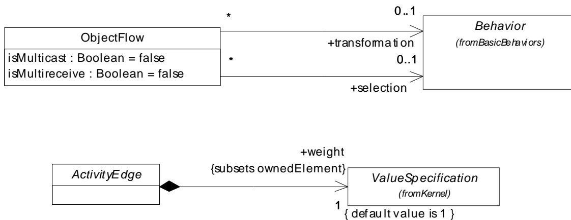
Figure 12.14 - Flows (CompleteActivities)
