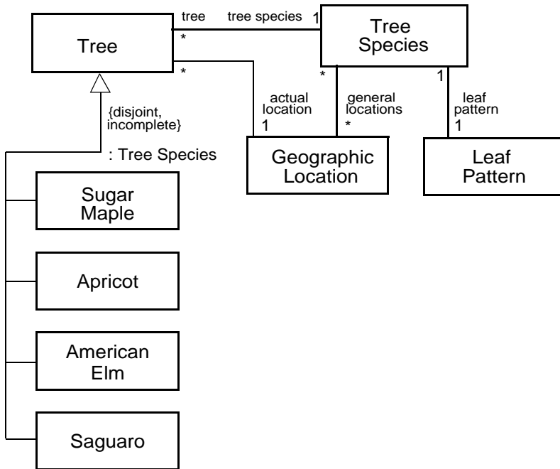
Figure 7.47 - Power type example and notation
