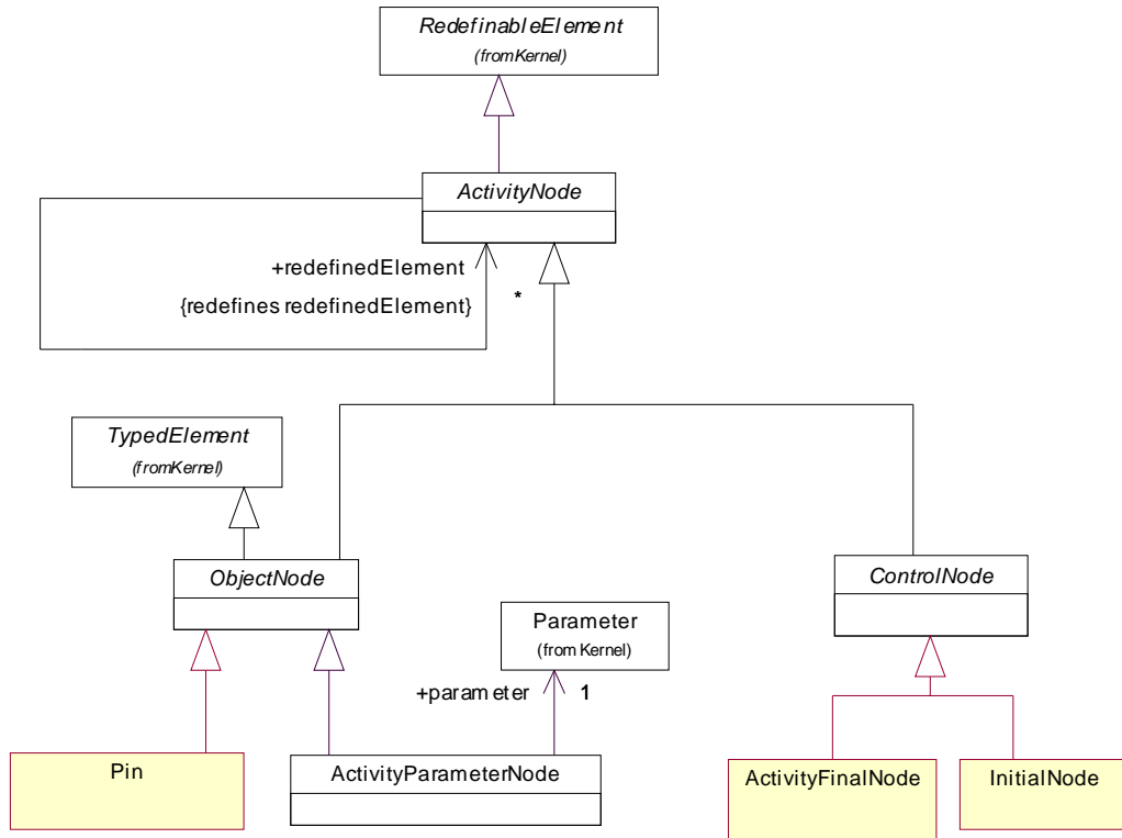
Figure 12.4 - Nodes (BasicActivities)
