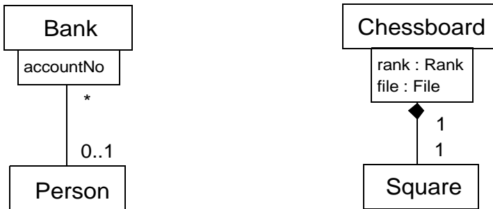
Figure 7.70 - Qualified associations
