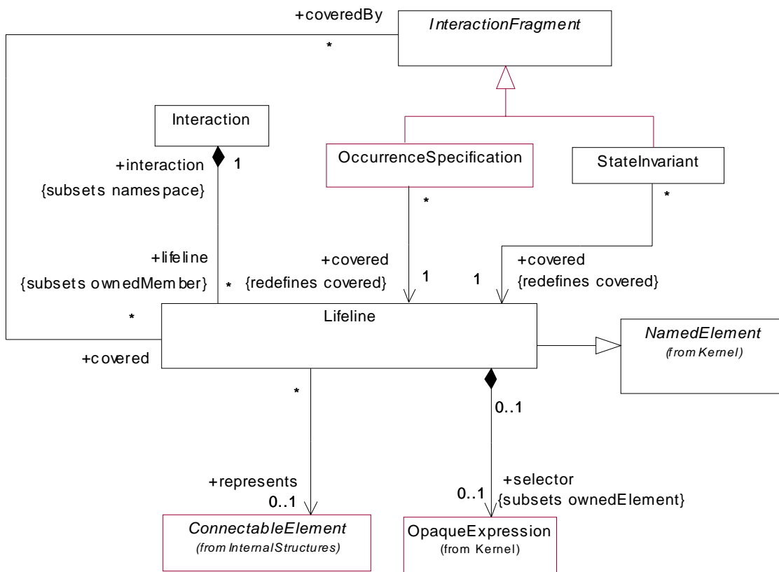
Figure 14.4 - Lifelines
