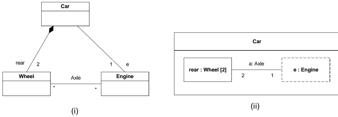
Figure 9.21 - Properties
