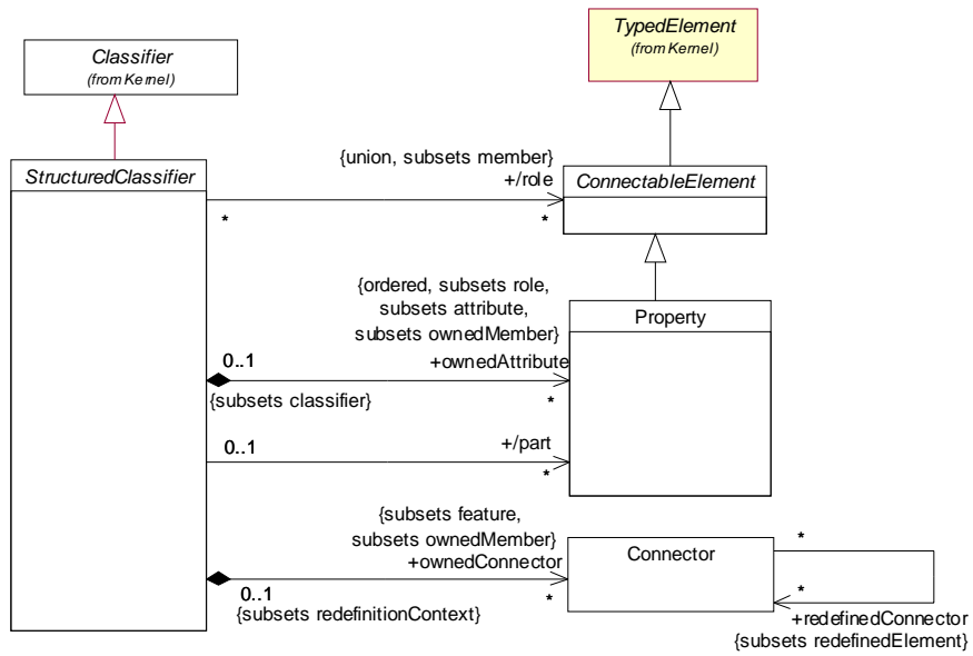
Figure 9.2 - Structured classifier
