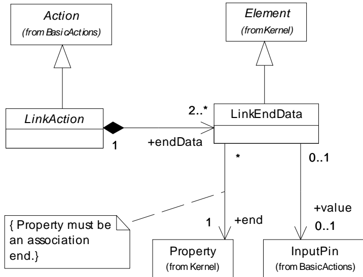
Figure 11.8 - Link identification
