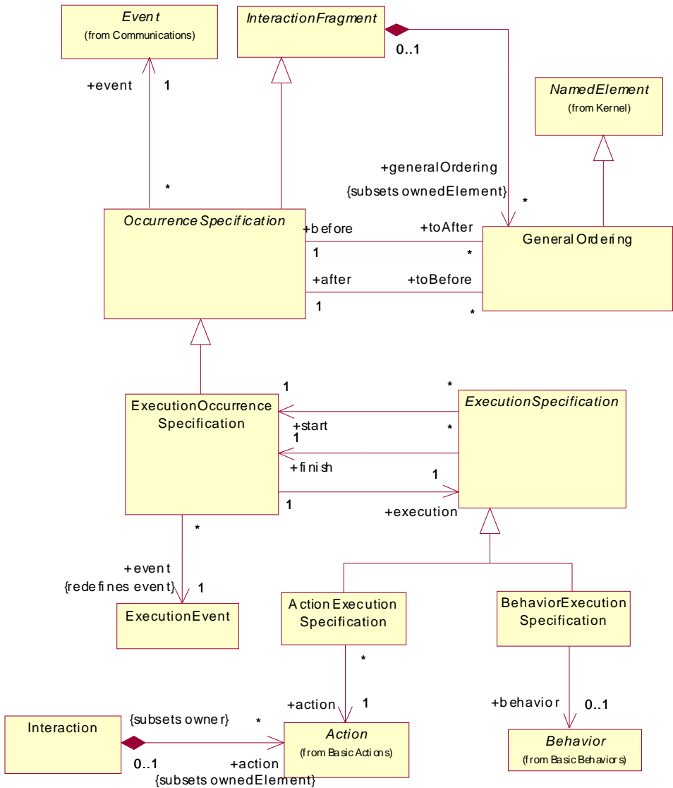
Figure 14.6 Occurrences
