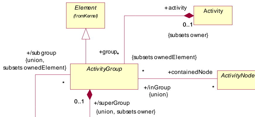
Figure 12.3 - Fundamental groups
