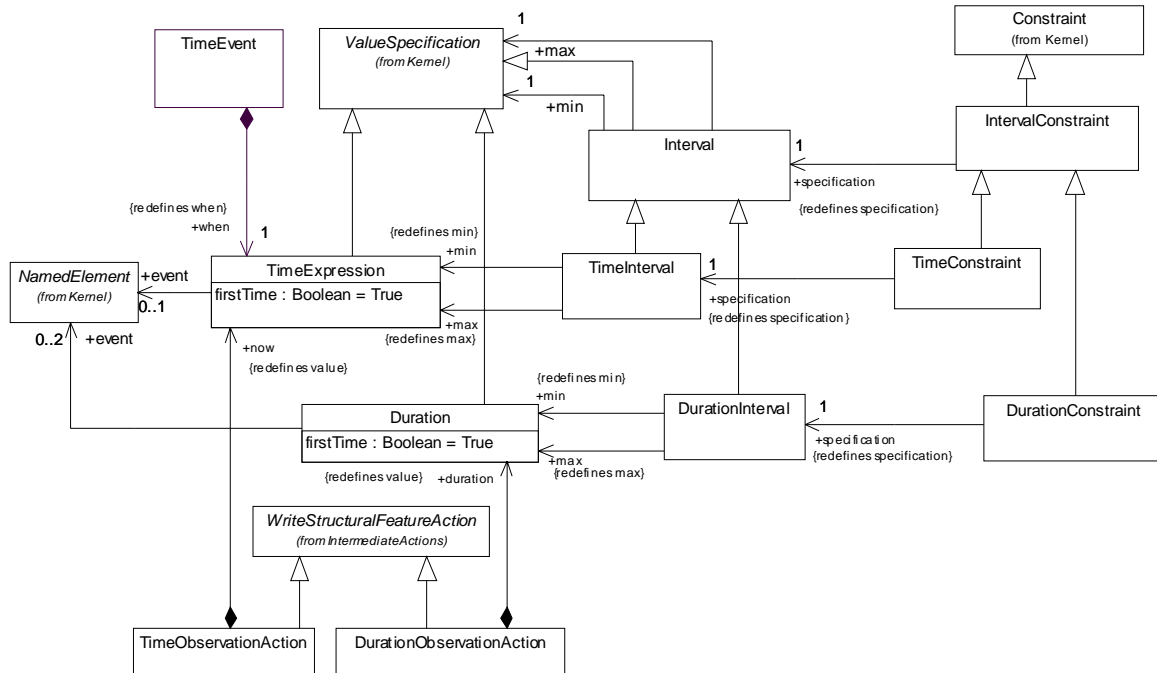
Figure 13.13 - SimpleTime
