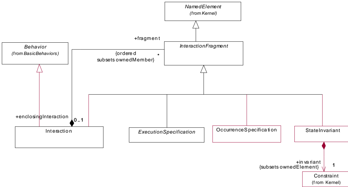
Figure 14.3 - Interactions
