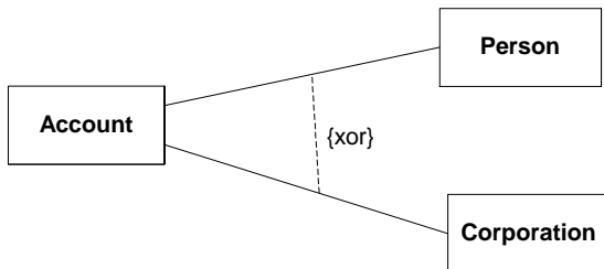
Figure 7.32 - {xor} constraint
