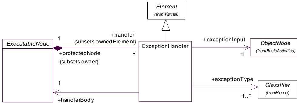
Figure 12.23 - Exceptions
