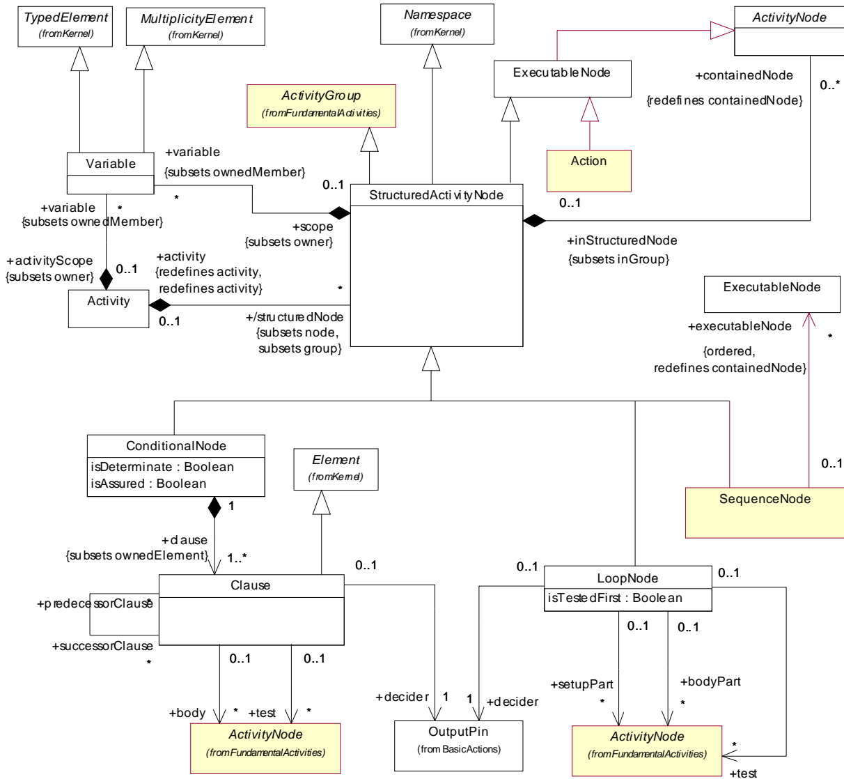
Figure 12.21 - Structured nodes
