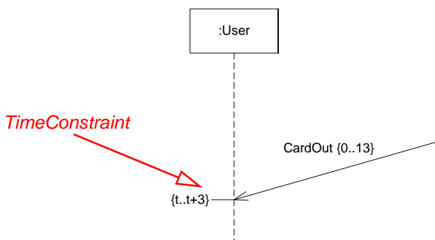
Figure 13.18 - TimeConstraint
