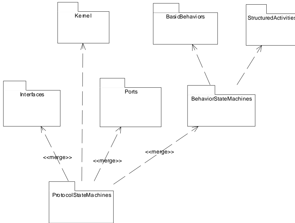
Figure 15.1 - Package Dependencies
