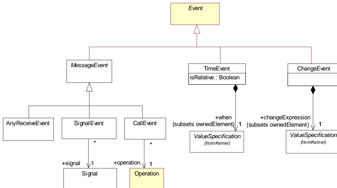
Figure 13.12 - Events
