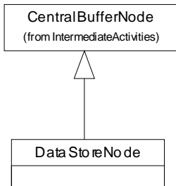
Figure 12.17 - Data stores
