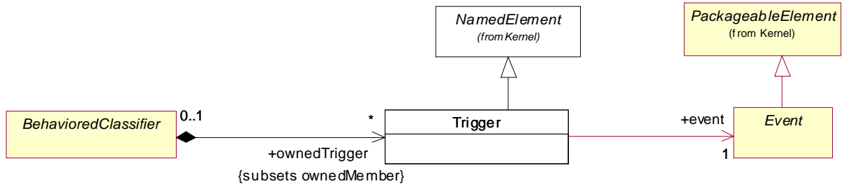
Figure 13.11 - Triggers
