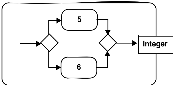
Figure 12.135 - Example ValueSpecificationAction
