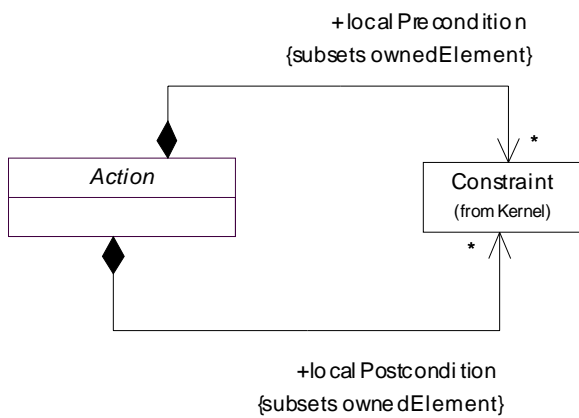
Figure 12.13 - Constraints (CompleteActivities)
