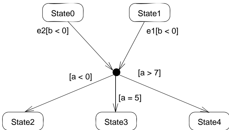
Figure 15.22 - Junction
