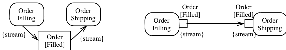
Figure 12.128 - Pin examples
