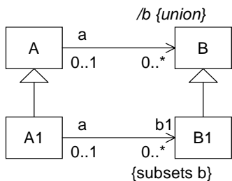
Figure 7.23 - Derived supersets (union)
