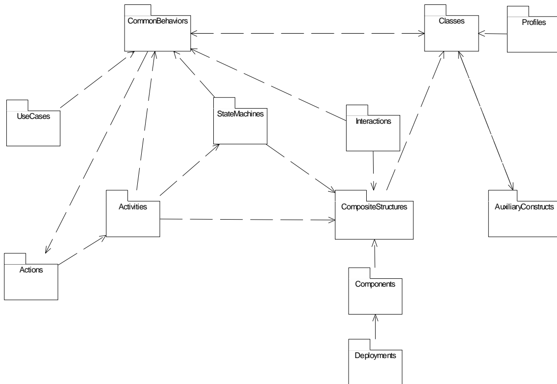
Figure 7.5 - The top-level package structure of the UML 2.0 Superstructure
