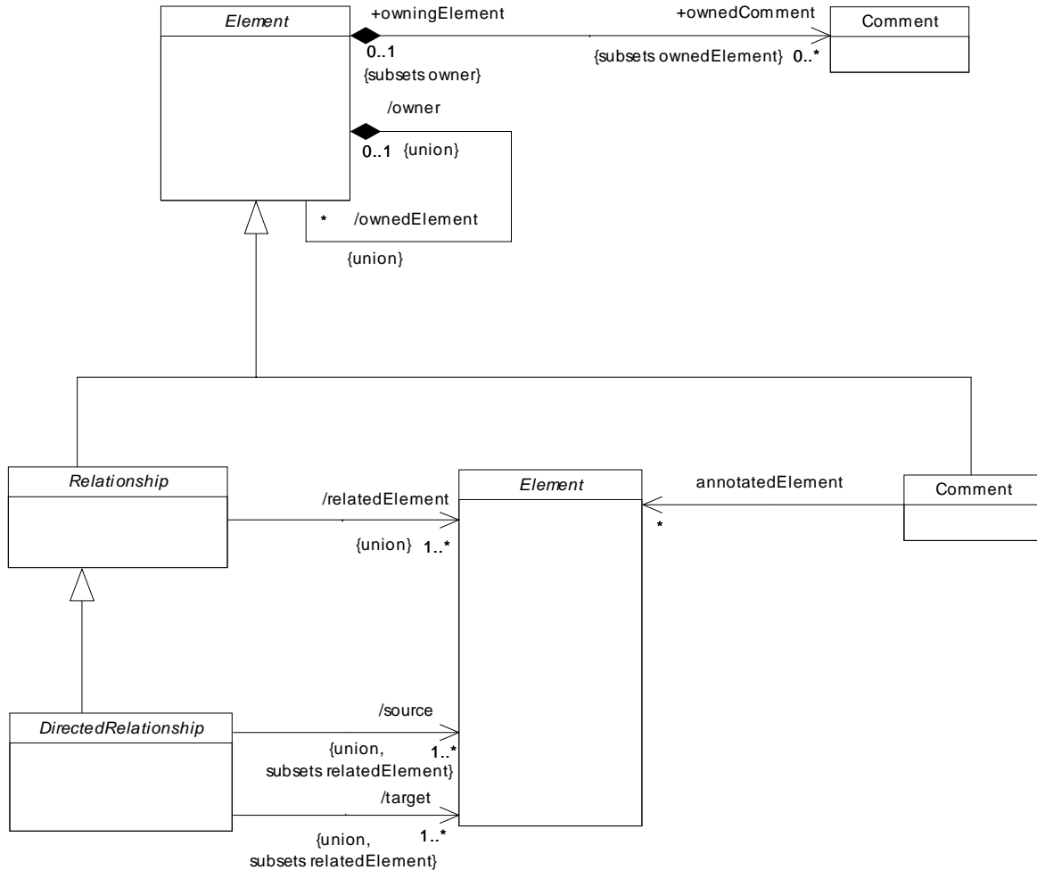
Figure 11.3 - The Root diagram of the Constructs package
