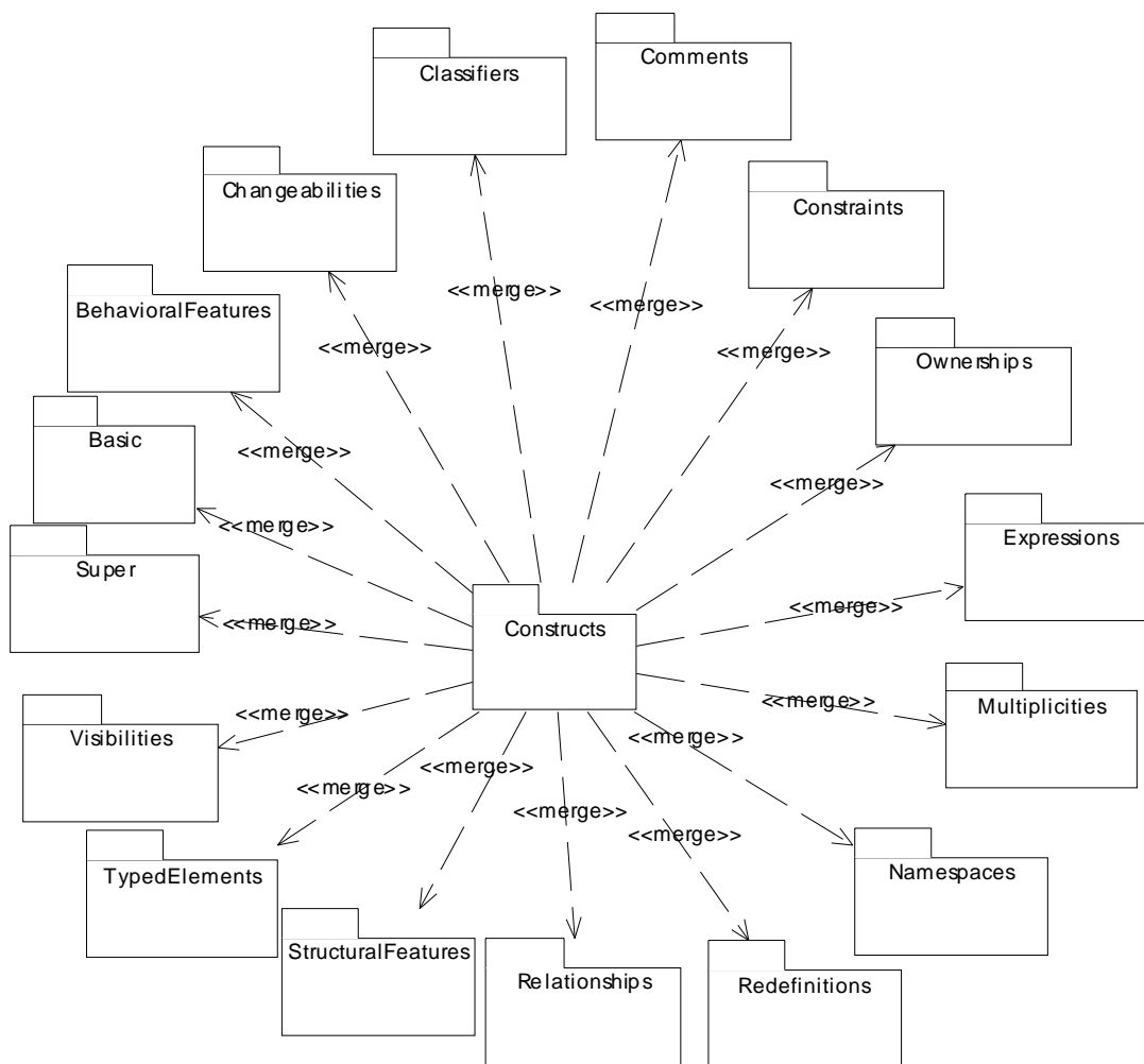
Figure 11.2 - The Constructs package depends on several other packages
