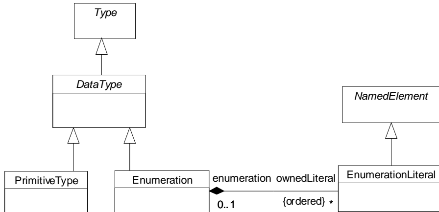
Figure 10.4 - The classes defined in the DataTypes diagram
