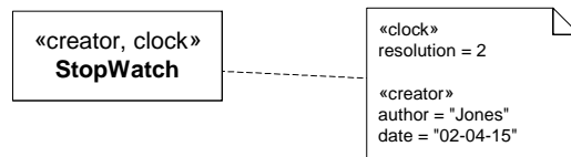
Figure 13.18 - Using stereotypes and showing values
