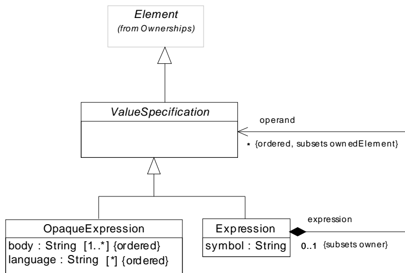
Figure 9.20 - The elements defined in the Expressions package
