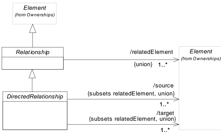
Figure 9.44 - The elements defined in the Relationships package
