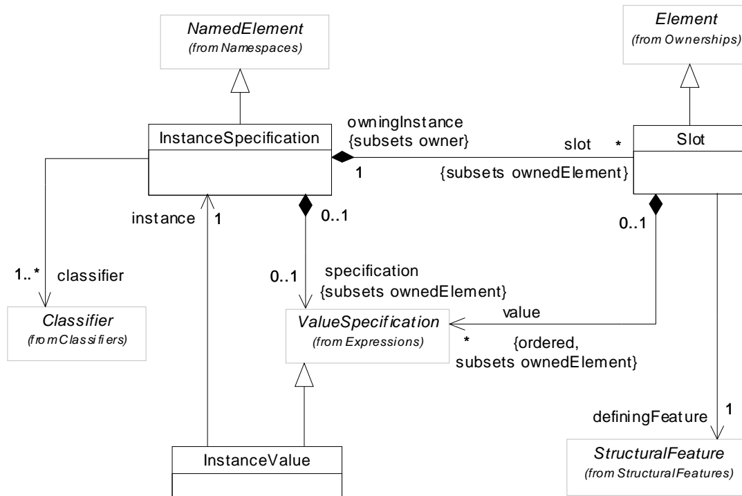
Figure 9.25 - The elements defined in the Instances package
