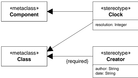
Figure 13.15 - Defining multiple stereotypes on multiple stereotypes
