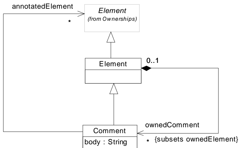
Figure 9.10 - The elements defined in the Comments package
