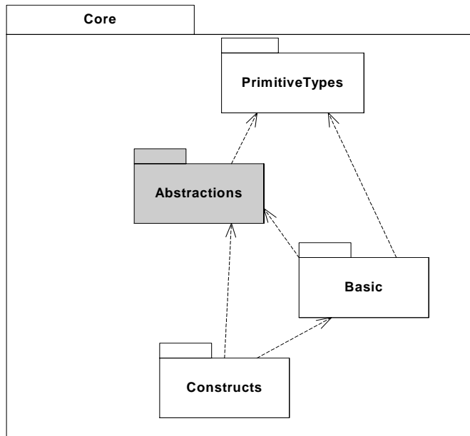
Figure 9.1 - The Core package is owned by the InfrastructureLibrary pack and contains several subpackages
