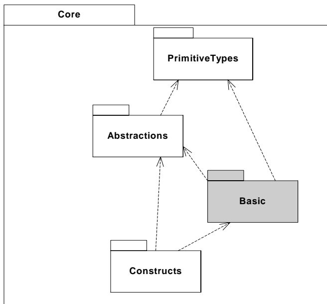
Figure 10.1 - The Core package is owned by the InfrastructureLibrary package, and contains several subpackages
