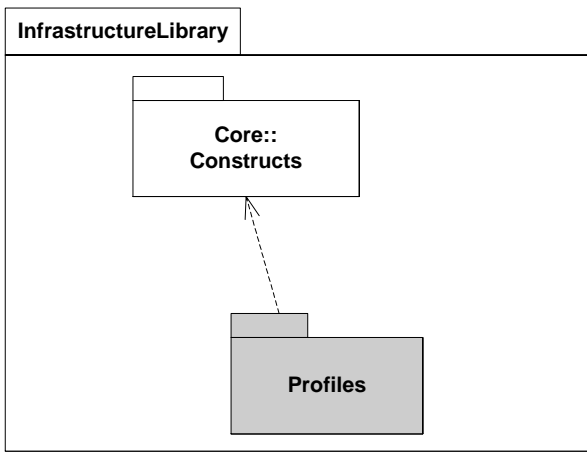
Figure 13.1 - The Profiles package is owned by the InfrastructureLibrary package
