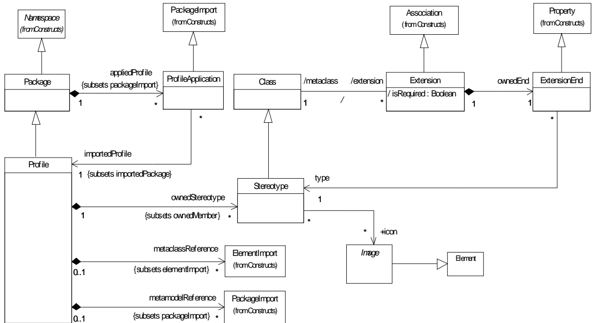
Figure 13.2 - The classes defined in the Profiles package
