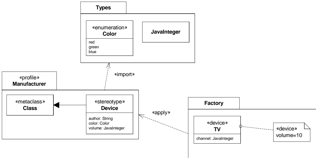
Figure 13.10 - Importing a package from a profile
