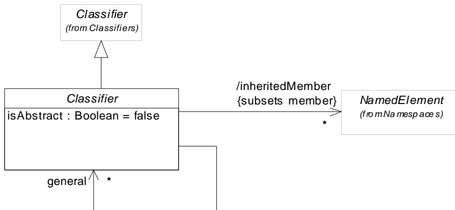
Figure 9.48 - The elements defined in the Super package
