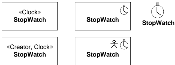
Figure 13.13 - Presentation options for an extended class
