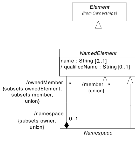
Figure 9.38 - The elements defined in the Namespaces package
