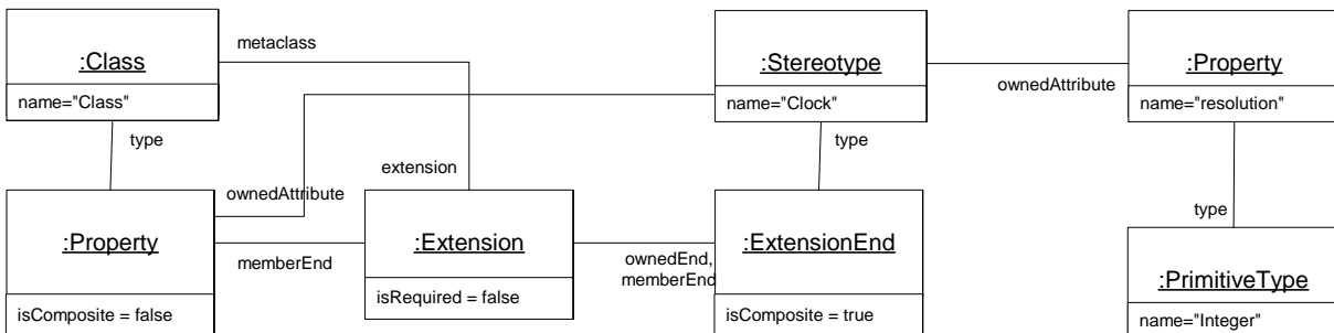
Figure 13.14 - An instance specification when defining a stereotype
