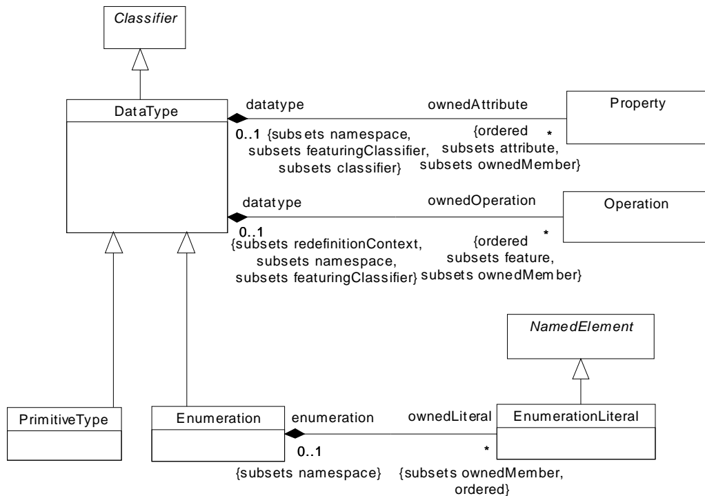
Figure 11.18 - The classes defined in the DataTypes diagram
