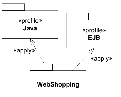
Figure 13.11 - Profiles applied to a package
