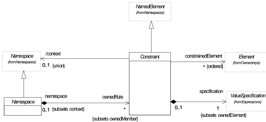
Figure 9.13 - The elements defined in the Constraints package
