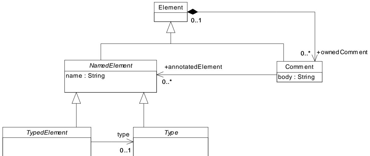
Figure 10.2 - The classes defined in the Types diagram
