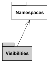
Figure 9.52 - The Visibilities package
