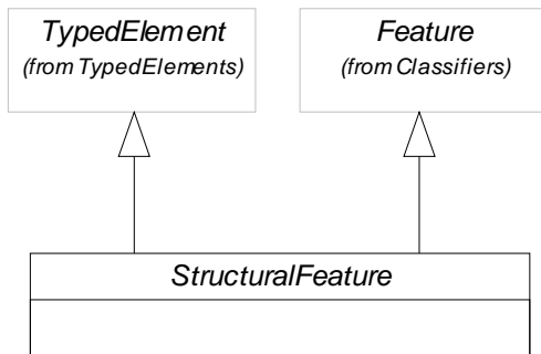
Figure 9.46 - The elements defined in the StructuralFeatures package
