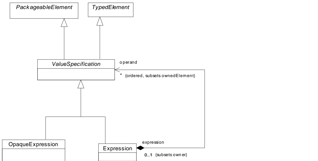
Figure 11.4 - The Expressions diagram of the Constructs package
