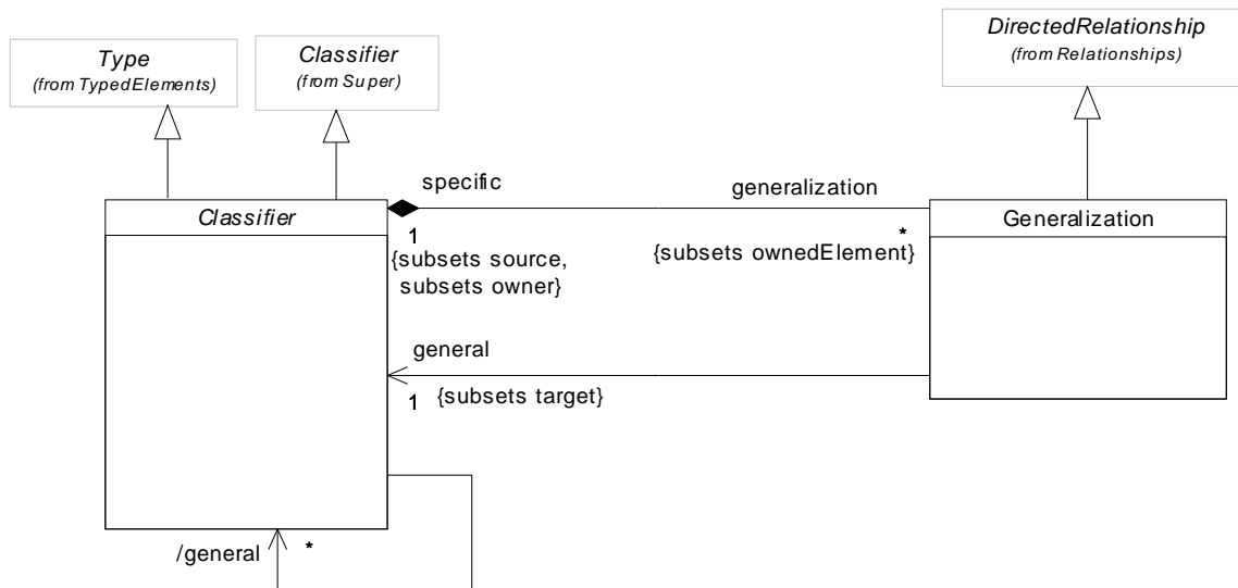
Figure 9.22 - The elements defined in the Generalizations package
