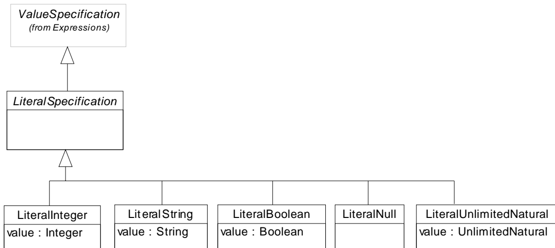
Figure 9.30 - The elements defined in the Literals package
