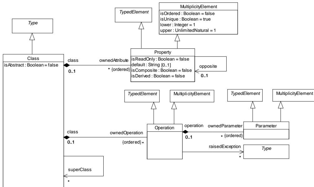
Figure 10.3 - The classes defined in the Classes diagram
