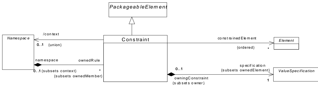
Figure 11.17 - The Classes diagram of the Constructs package
