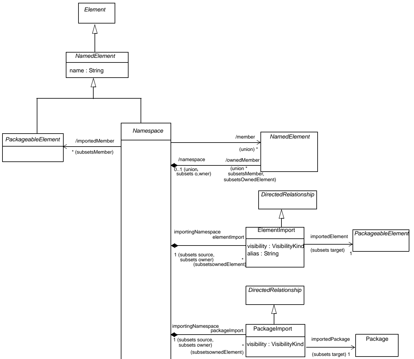
Figure 11.21 - The Namespaces diagram of the Constructs package
