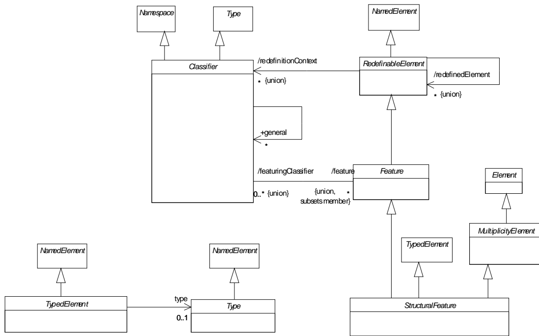
Figure 11.16 - The Classifiers diagram of the Constructs package
