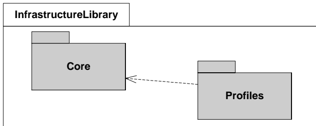
Figure 7.1 The InfrastructureLibrary packages
