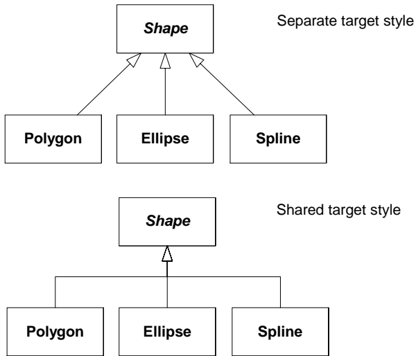
Figure 9.23 - Examples of generalizations between classes
