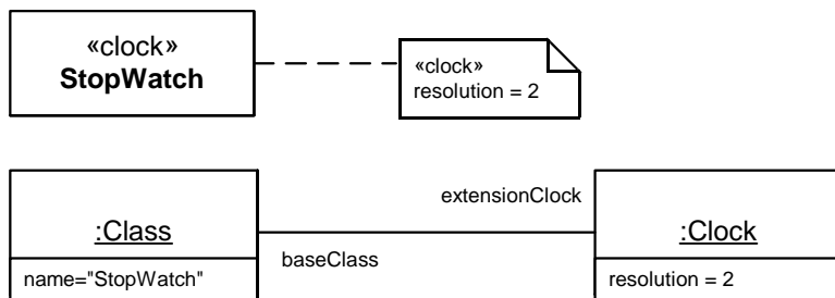
Figure 13.17 - Showing values of stereotypes and a simple instance specification
