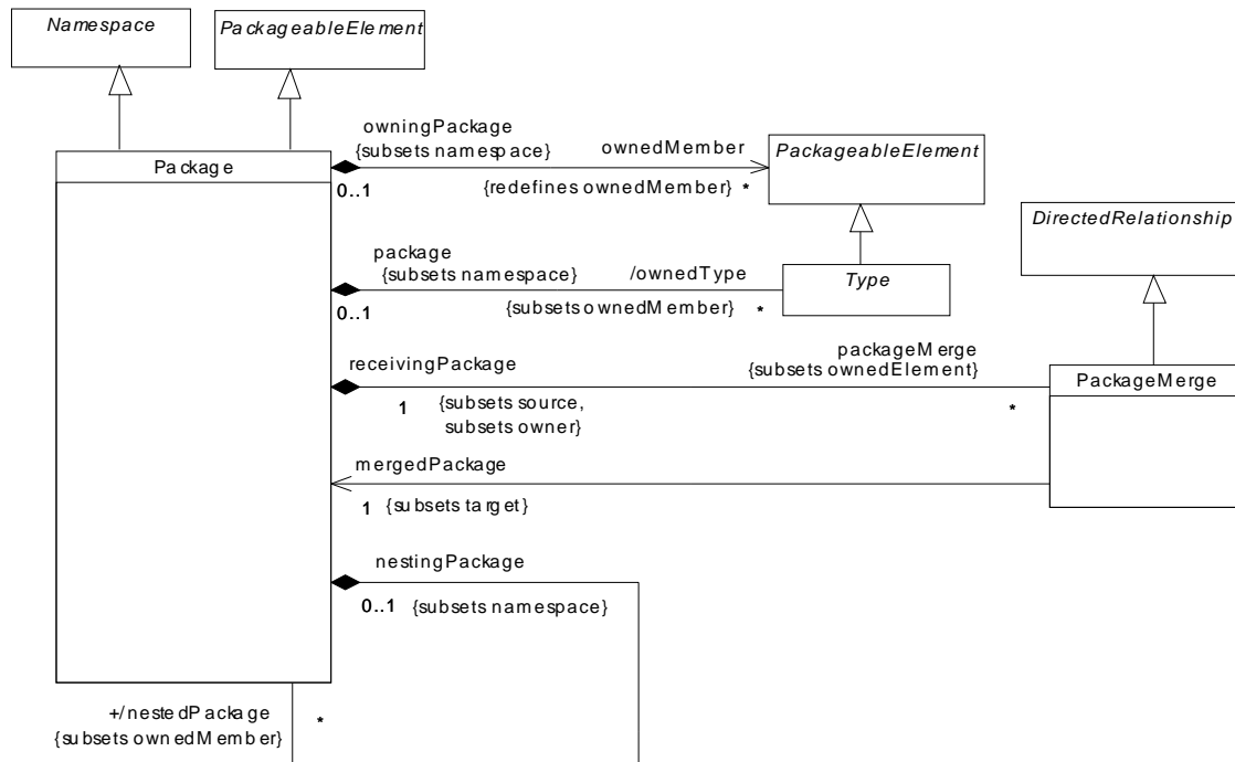
Figure 11.26 - The Packages diagram of the Constructs package
