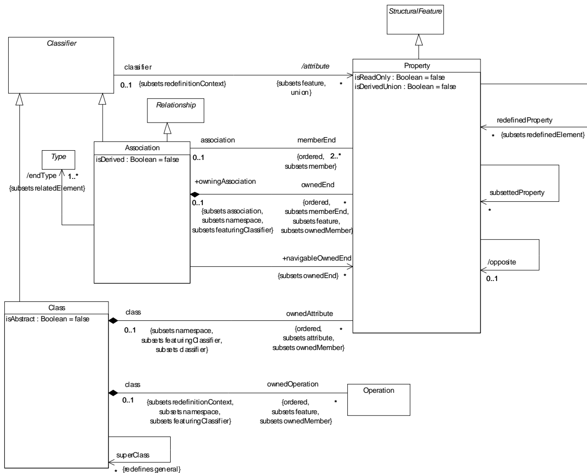
Figure 11.5 - The Classes diagram of the Constructs package
