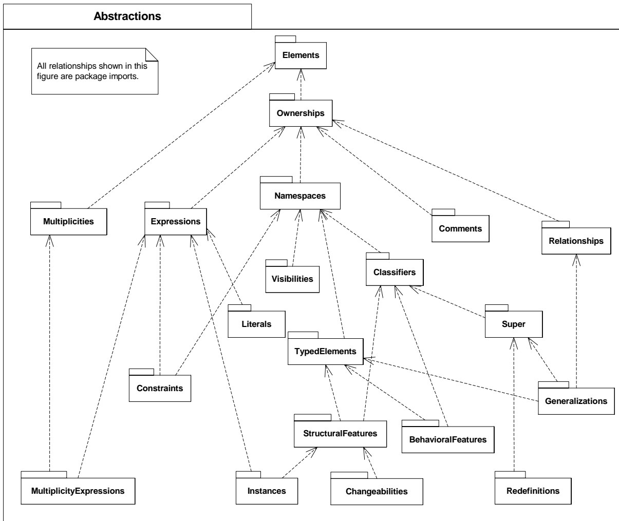
Figure 9.2 - The Abstractions package contains several subpackages, all of which are specified in this chapter
