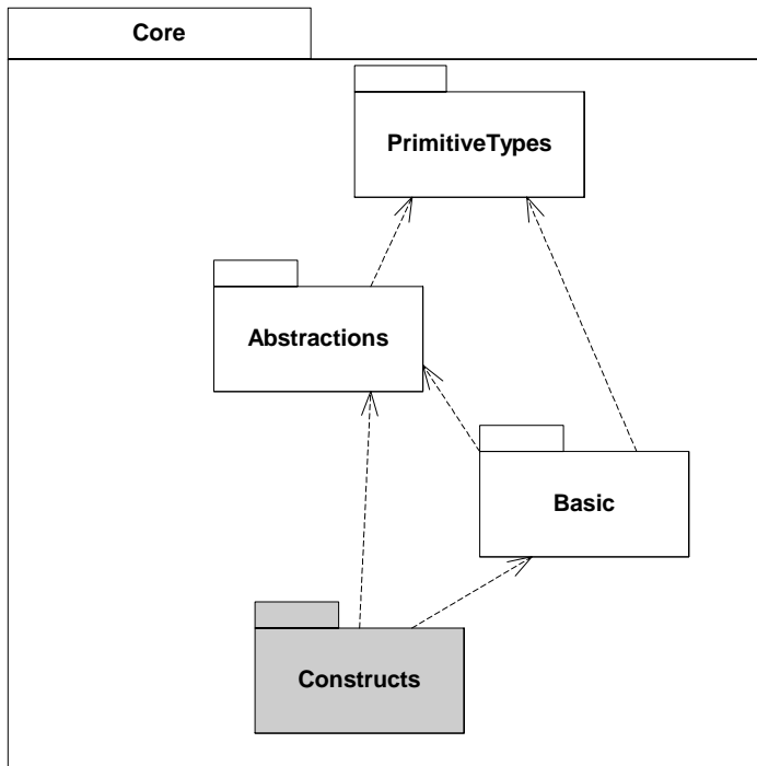
Figure 11.1 - The Core package is owned by the InfrastructureLibrary package, and contains several subpackages
