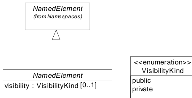
Figure 9.53 - The elements defined in the Visibilities package
