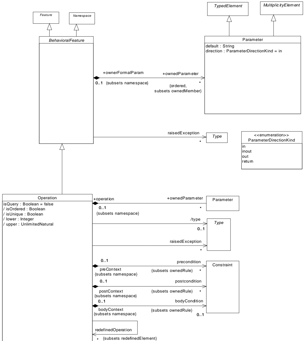
Figure 11.25 - The Operations diagram of the Constructs package
