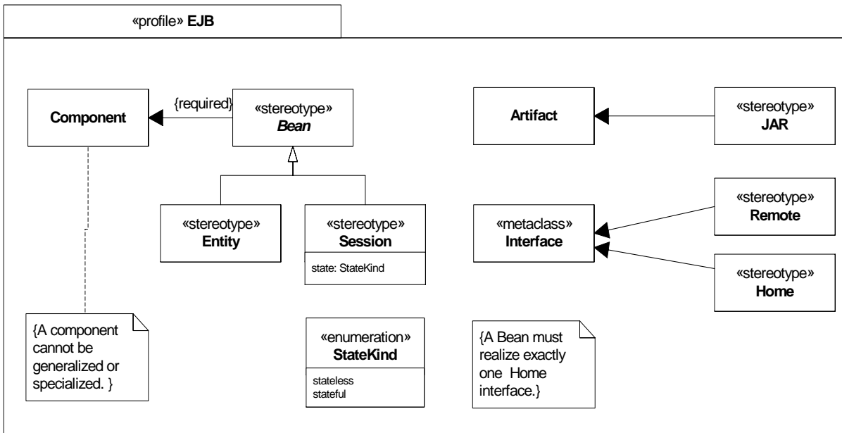
Figure 13.9 - Defining a simple EJB profile
